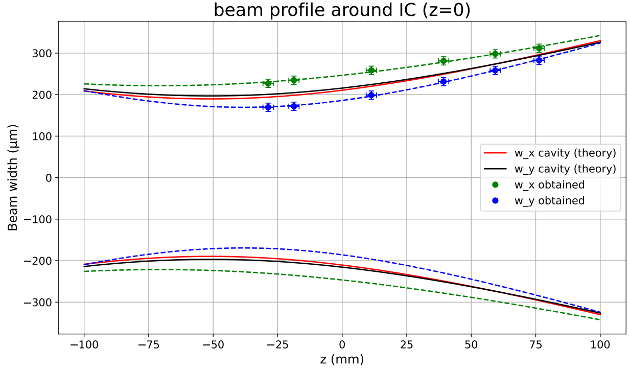
Figure 3: Beam profile measurements fitted to the gaussian beam propagation.
