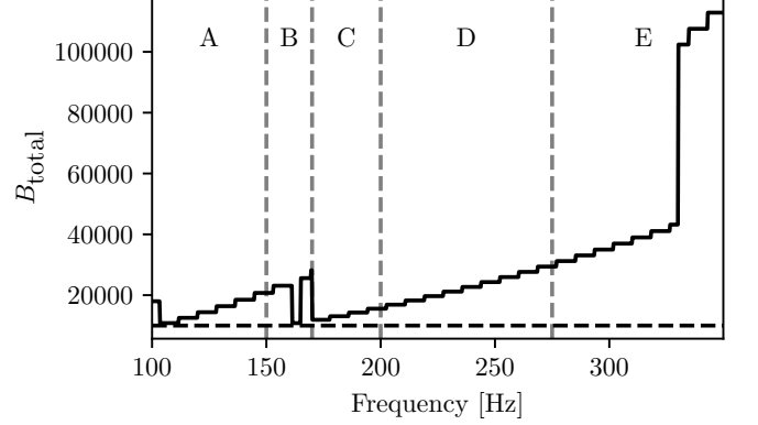
FIG. 3. Total number of boxes per 0.125 Hz frequency band across the full search range. The lettered regions (A-E) correspond to the frequency intervals defined in Table II. The dashed horizontal line marks the minimum enforced number of boxes ( 10^4 ). Sudden changes in the number of boxes correspond to transitions between regions where either the minimum box constraint or the 10^8 templates-per-box criterion dominates the partitioning as explained in App. A.
