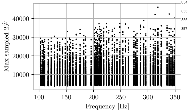
FIG. 8. First-stage MCMC follow-up results on injection studies with T_{\text{coh}} = 12 h. Each point corresponds to the maximum 2\hat{\mathcal{F}} value sampled for each injected signal. 14750 Injections were run, with 2 obtaining a final 2\hat{\mathcal{F}} below 3850. Signals were injected at the sensitivity depths values obtained per each region shown in Table IV.
