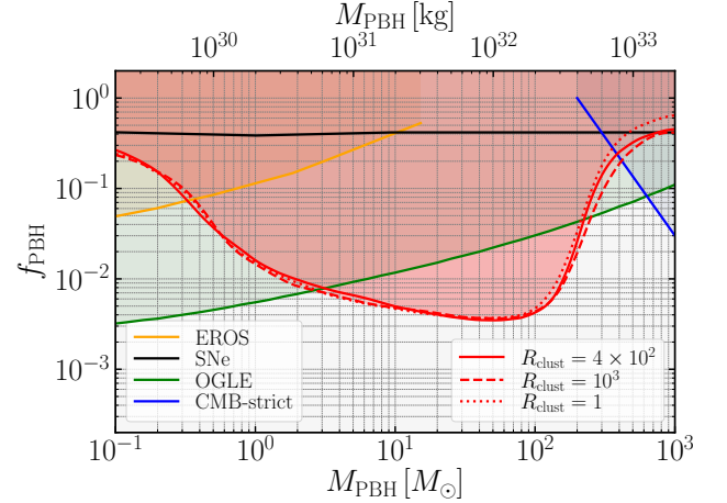
FIG. 14. The 95% CL constraints on f_{\text{PBH}} as a function of M_{\text{PBH}} (= \mu) from the Bayesian analysis, shown for R_{\text{clust}} = 1, 4 \times 10^2, 10^3 (dotted, solid, and dashed red curves). We also show other observational constraints such as supernova lensing constraints (SNe, black) [322], Massive Compact Halo Object constraints (EROS, yellow) [323], the recent Optical Gravitational Lensing Experiment constraints (OGLE, green) [324], and Cosmic Microwave Background constraints (CMB, blue) [325].
