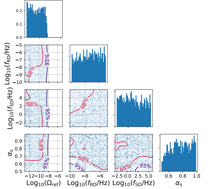
FIG. 8. Posteriors of the Bayesian analysis for an SD+CBC model. Contour regions in purple correspond to 95% CL and those in red to 68% CL.
