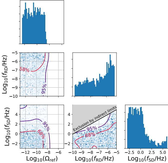
FIG. 8. Posteriors of the Bayesian analysis for an SD+CBC model. Contour regions in purple correspond to 95% CL and those in red to 68% CL.
