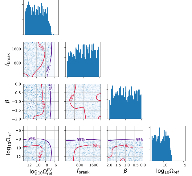
FIG. 19. Posterior distributions for early Universe turbulence with an overlaying CBC background model with \Pi(f) = (f/\text{Hz})^\beta .
