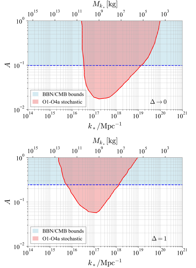
FIG. 12. Constraints on the curvature perturbation amplitude for \Delta = 0 (delta function case) and \Delta = 1 .
