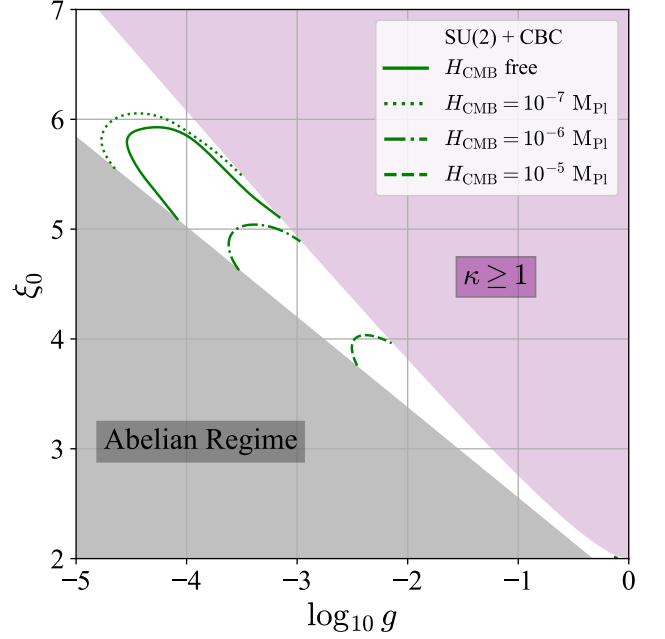
FIG. 10. Marginalized posterior in the \xi_0 - \log_{10} g plane obtained from a search for early Universe axion inflation with an overlaid astrophysical background, assuming fixed values of H_{\text{CMB}} = 10^{-7} M_{\text{Pl}}, 10^{-6} M_{\text{Pl}}, 10^{-5} M_{\text{Pl}} (dotted, dot-dashed, and dashed green lines, respectively), and also treating it as a free parameter (solid green line). The gray shaded region denotes the Abelian regime, where efficient gravitational-wave production is expected. The purple shaded region corresponds to the parameter space where strong back-reaction is anticipated, namely \kappa \geq 1 , and the gravitational wave amplitude estimates may no longer be reliable.
