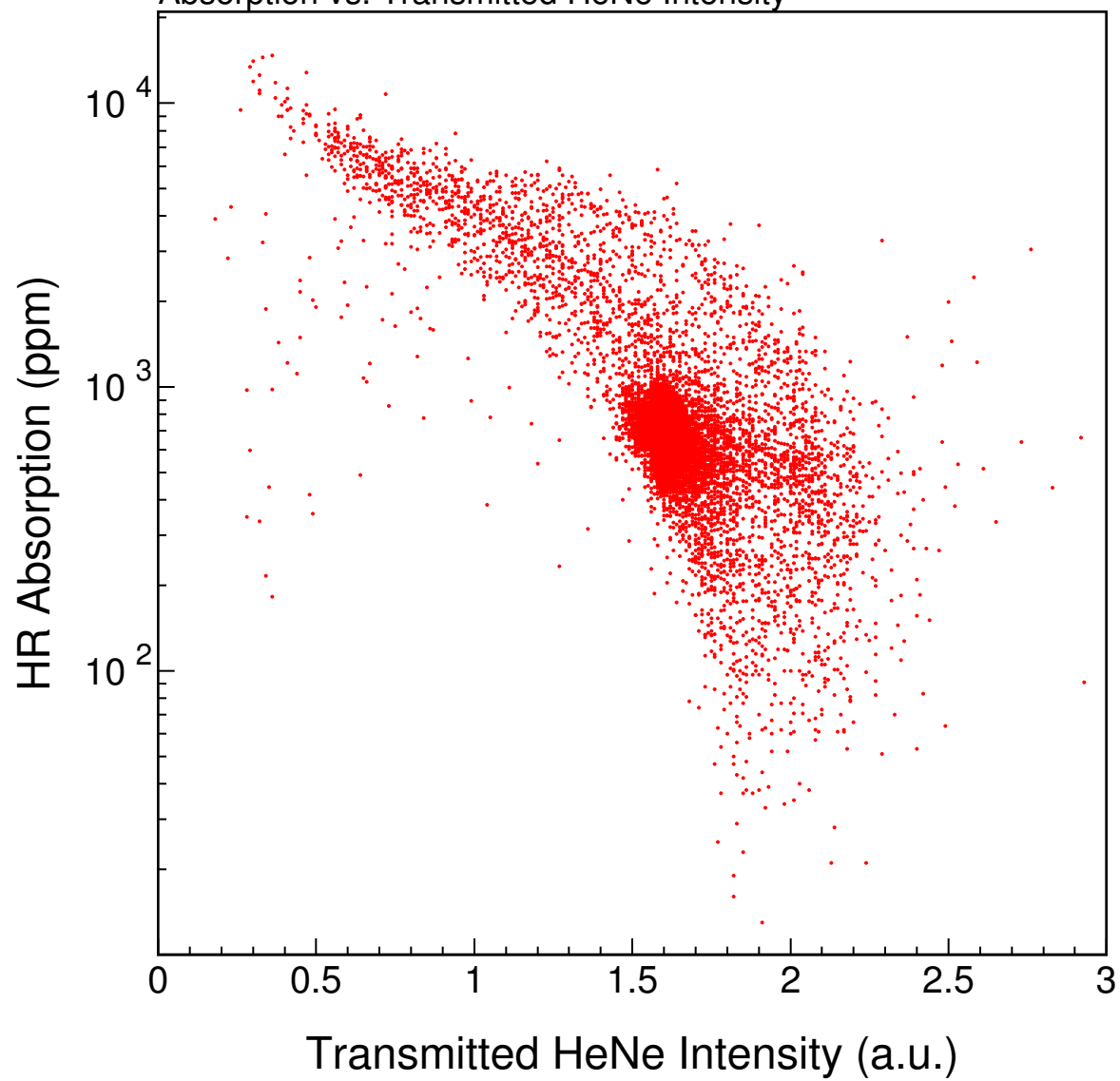
Pathfinder (ETM05) HR Absorption Scan, 030625 Absorption vs. Transmitted HeNe Intensity
