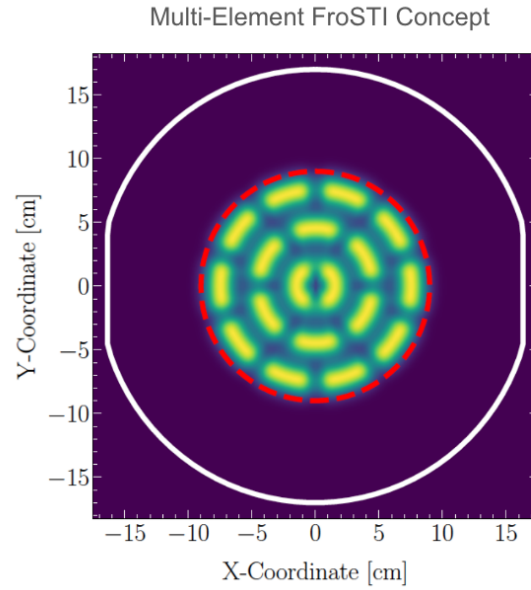
Figure 12: Model of a multi-element FROSTI concept.
