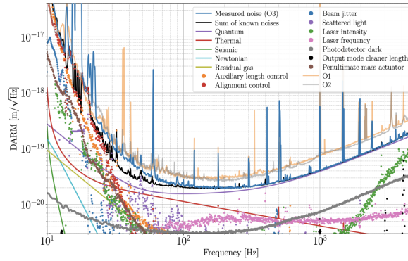
Figure 3: Noise Budget of LHO O3 [6]
