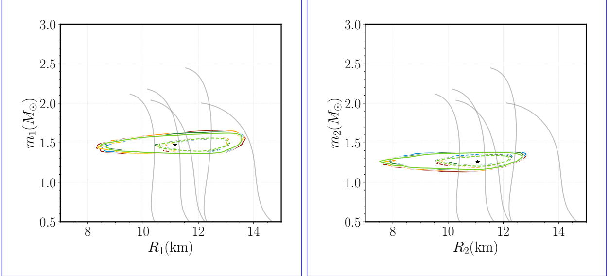
Figure 14: Mass-radius curves for a simulated GW170817-like BNS at a distance of 100 Mpc. We use universal relations to map from the tidal parameters to the neutron star radius R . Note that we do not enforce that both stars obey the same EOS. The LIGO sensitivities are A+ ( bluered ), A# (A+ coatings) ( orange ), A# Wideband (A+ coatings) ( green ), ( blue ), A# Wideband ( golden ), Voyager Wideband ( light green ) and Voyager Deep ( reddark green ). The gray grey curves indicate predictions for a set of EOS, the star marks the parameters of the simulated signal.
