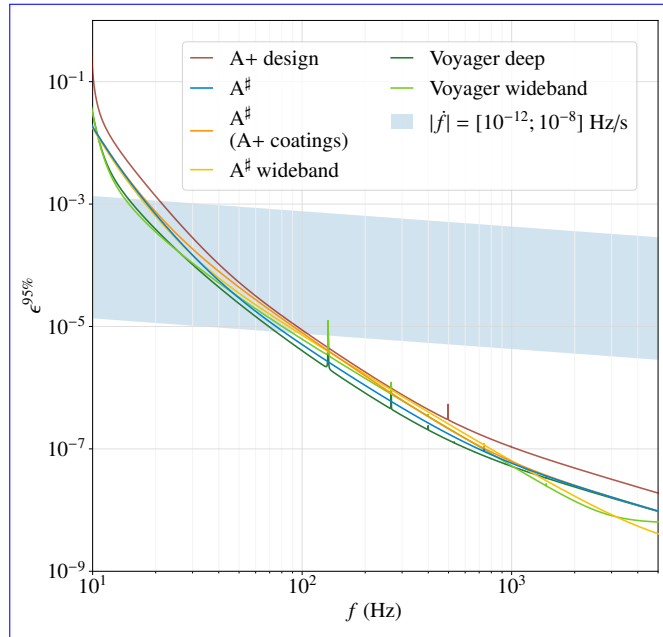
Figure 16: Sensitivity reach to all-sky searches of CWs (95% C.L.). The various continuous curves are the minimum detectable ellipticity as a function of frequency for different detector configurations, assuming a source distance of 5 kpc, an observation time T_{\text{obs}} = 1 year, a duty cycle D = 80\% and data segments duration T_{\text{FFT}} = 1 day. The shaded area is delimited by lines of constant spin-down of, respectively, 10^{-12} Hz/s and 10^{-8} Hz/s.
