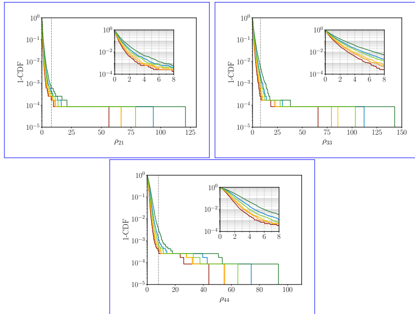
Figure 12: Expected distribution of SNR in the higher-order modes (\ell, |m|) = (2, 1), (3, 3), (4, 4) for BBH events drawn from the underlying astrophysical population with a network SNR \rho_N > 12 for five six different LIGO sensitivities: A+ ( blue red), A # (A+ coatings) (orange), A # Wideband (A+ coatings) (blue), A # Wideband (golden), Voyager Wideband (light green) and Voyager Deep ( red dark green). The inset shows a zoom-in of the region where \rho_{\ell m} \leq 8 . The vertical dashed line indicates an SNR of 6.
