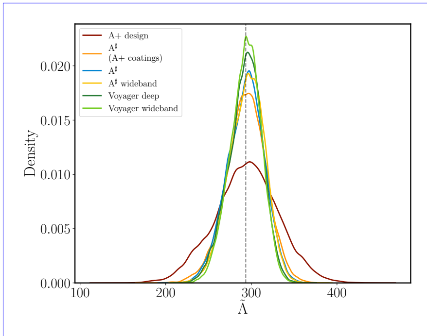
Figure 13: One-dimensional posterior probability density of the binary tidal deformability \tilde{\Lambda} for a simulated GW170817-like BNS event at a distance of 100 Mpc for different LIGO sensitivities. The dashed vertical line indicates the parameter of the simulated signal.
