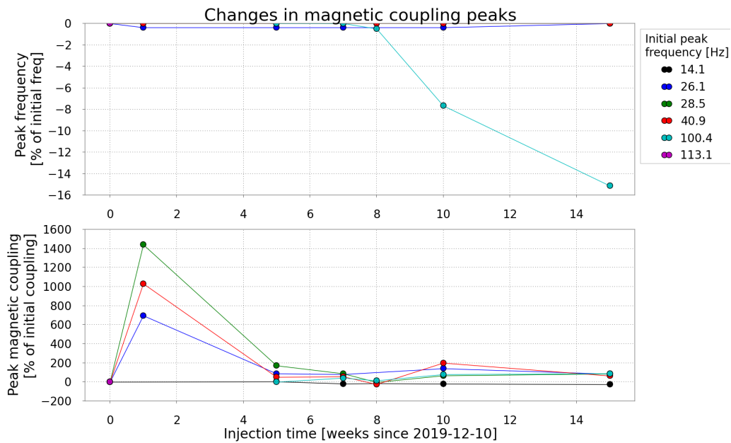
Figure 27. Weekly trends in frequency (top) and amplitude (top) of peaks in the magnetic coupling functions.
