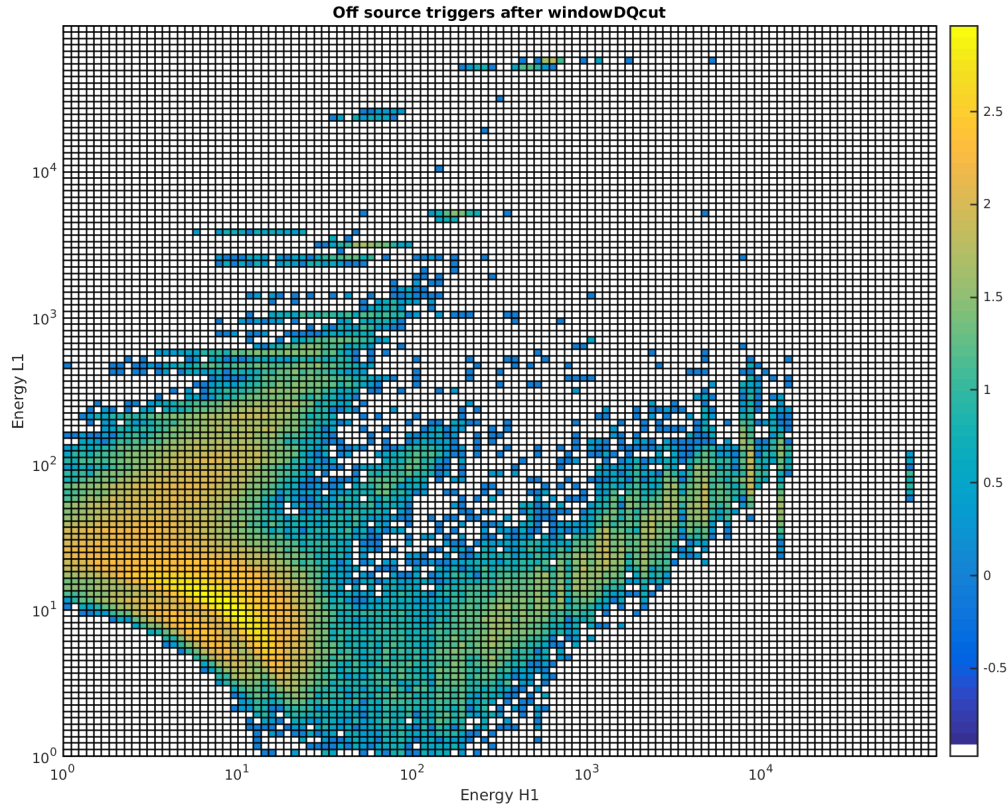
Figure 33. Distribution of off-source triggers in the LIGO detectors without autogating. The x- and y-axes are the signal energy in H1 and L1, respectively.
