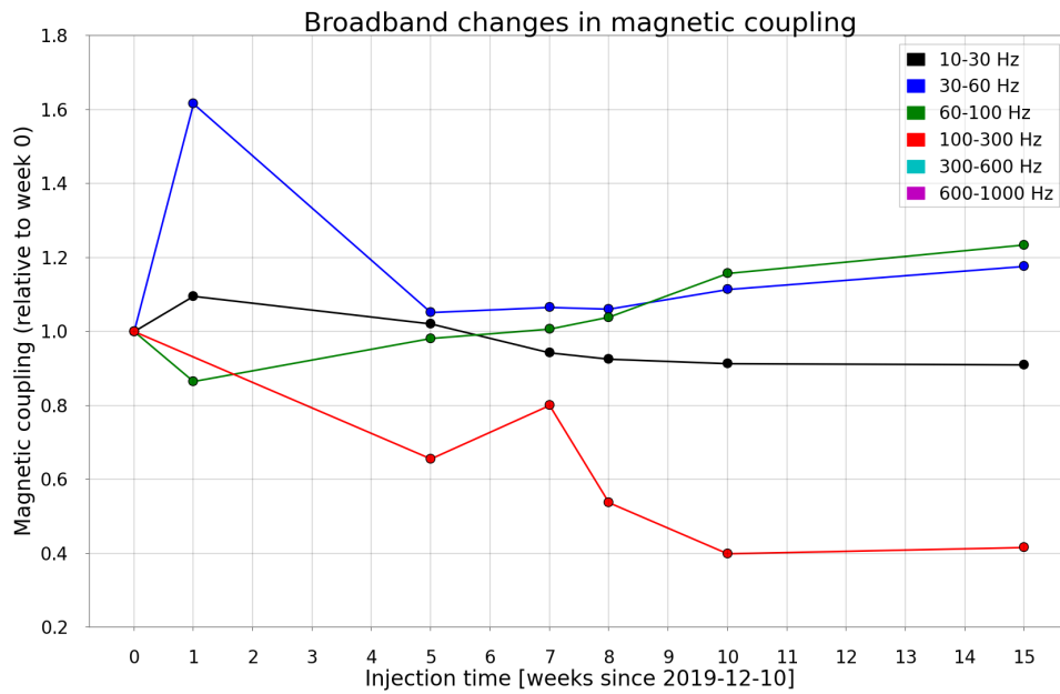
Figure 26. Time-lines of magnetic coupling changes relative to the start of the observing run.
