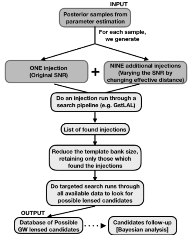
Figure 9. The pipeline to search for sub-threshold gravitational waves as used in [7]. The template bank is reduced by injecting signals with altered and original SNR into the data and only preserving the templates which recover these injections. The new template bank is used to search through all the data, which now has a reduced noise background due to the reduced template bank. Follow-up then needs to be performed on the candidates from this targeted search. Figure from [7].
