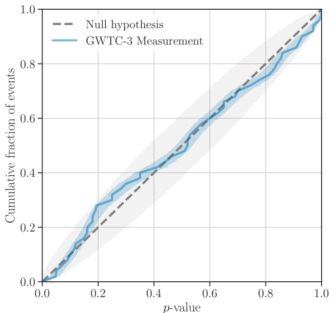
FIG. 2. Results of the residuals analysis (Sec. IV A). The blue curve shows the fraction of events with p -values of the residual SNR less than or equal to the abscissa (PP plot). The light-blue band represents the 90% credible interval of the observed p -values. The diagonal dashed line denotes the null hypothesis with the surrounding light-grey area denoting the 90% uncertainty region of the null hypothesis due to the finite number of events.
