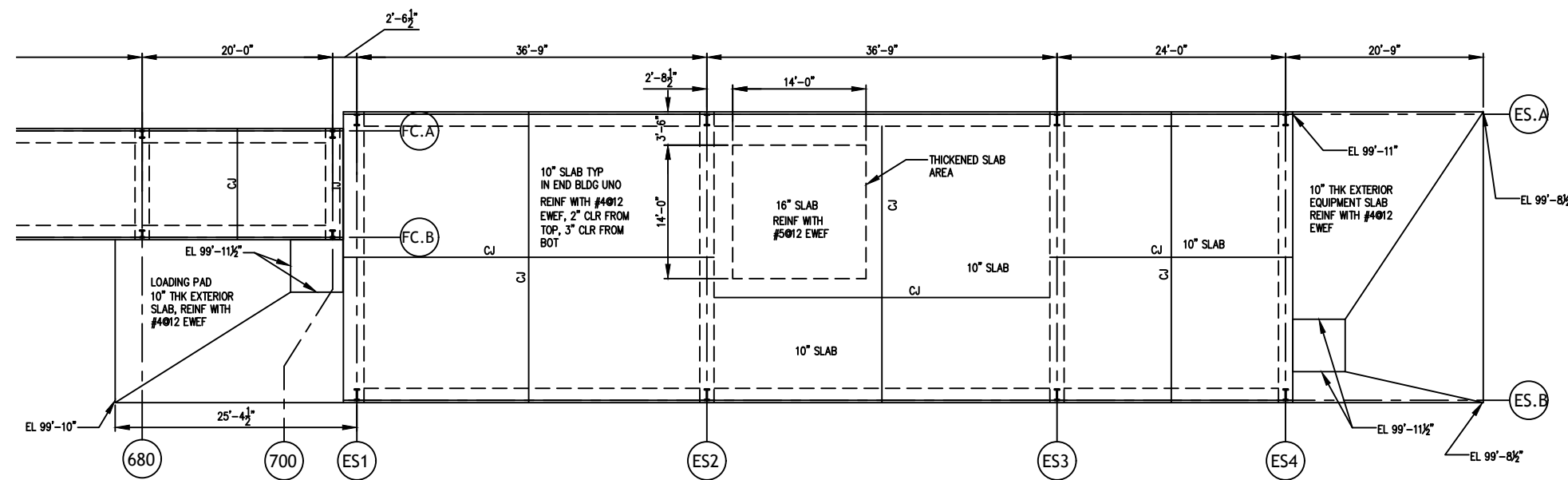
1 FCES - SLAB PLAN S100 1/8" = 1'-0"
