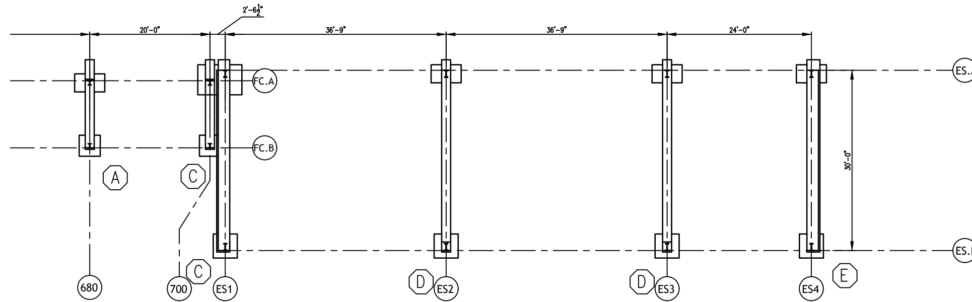
1 FCES - FOUNDATION PLAN S100 1/8" = 1'-0"
