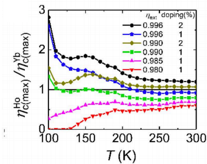
Figure 6: A graph showing the ratio of expected maximum cooling efficiencies at different temperatures of Ho:YLF coolant to the optimal efficiencies found in Yb:YLF. We can see that Ho:YLF has the potential for significant efficiency improvements at low temperature, especially with improvements to quantum efficiency. Figure from [28]
