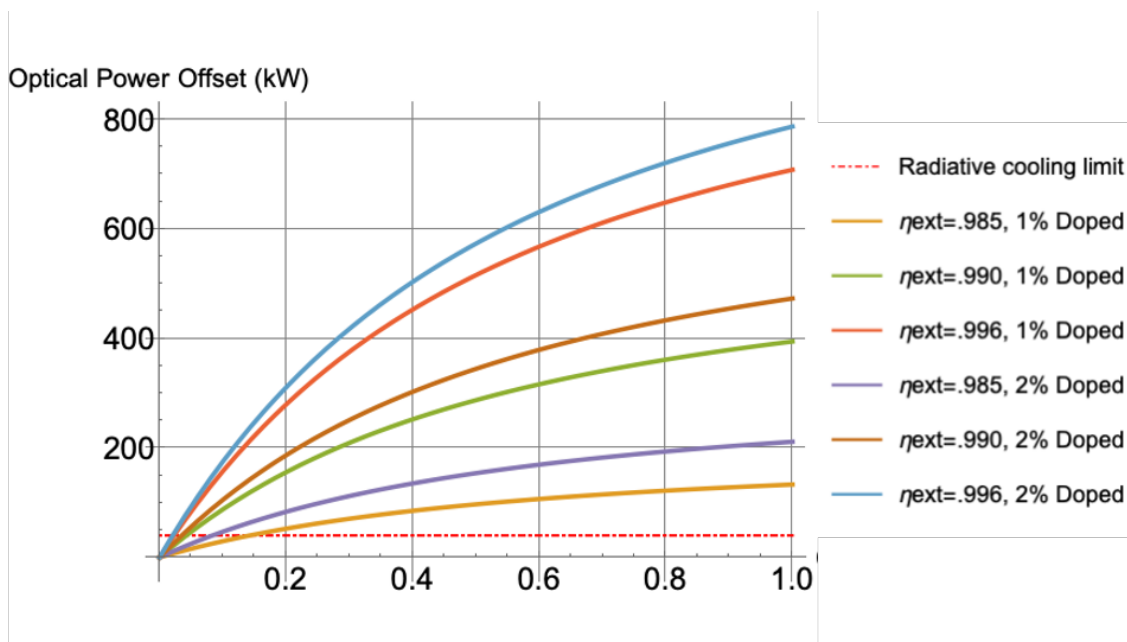
Figure 11: Plots of cavity power offset versus crystal mass for several specifications of holmium-doped crystals. The limit for radiative cooling is shown in the red dotted line. Note that crystals with current values of quantum efficiency ( \eta_{ext}=.980 ) are not depicted here because they do not cool at 123 K. Mass dependence on cooling comes from the limits of absorption when pumping on the cooling tail of the absorption spectrum. The cooling power shows strong dependence on \eta_{ext} as well as weaker dependence on doping concentration, reflecting the fact that current crystals have higher absorption efficiency than quantum efficiency at 123 K. For reference, the crystal used for the spectroscopy that was a basis for these plots had a mass of \sim 5 g.
