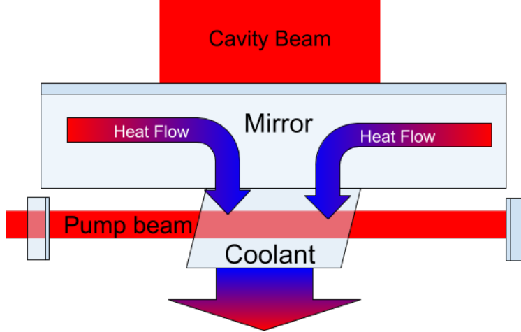
Figure 13: A schematic for the proposed arrangement of using an optical coolant to cool PSOMA. Even though the arrow representing the fluorescence is only pointed away from the mirror, the fluorescence in reality would be isotropic from all points in the path of the beam.
