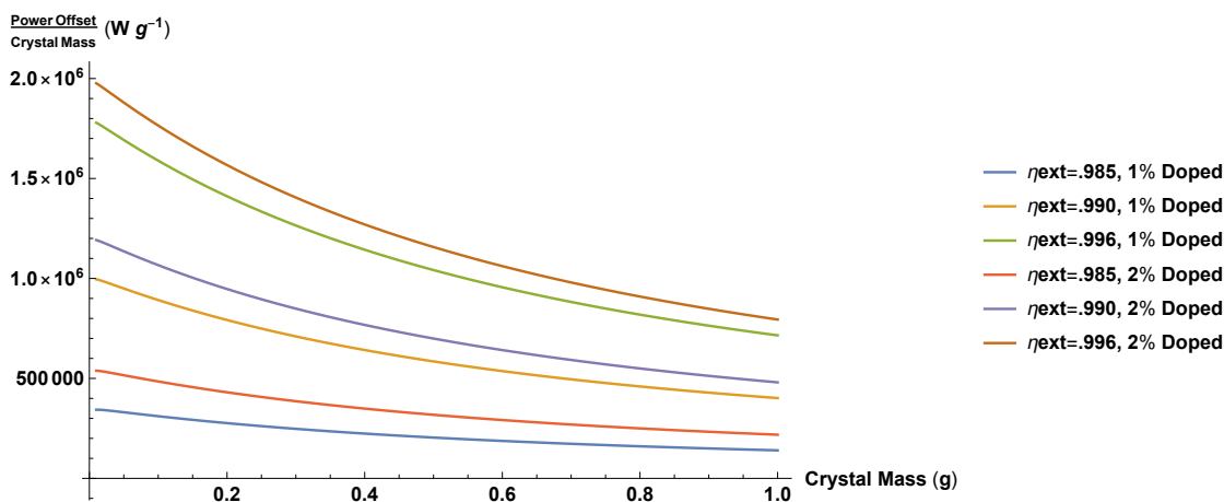
Figure 12: Plots of per mass offset power versus mass for several specifications of holmium-doped crystals. Like before, crystals with \eta_{ext}=.980 are excluded. All of these crystals would be able to offset much more power per mass than can be done radiatively.
