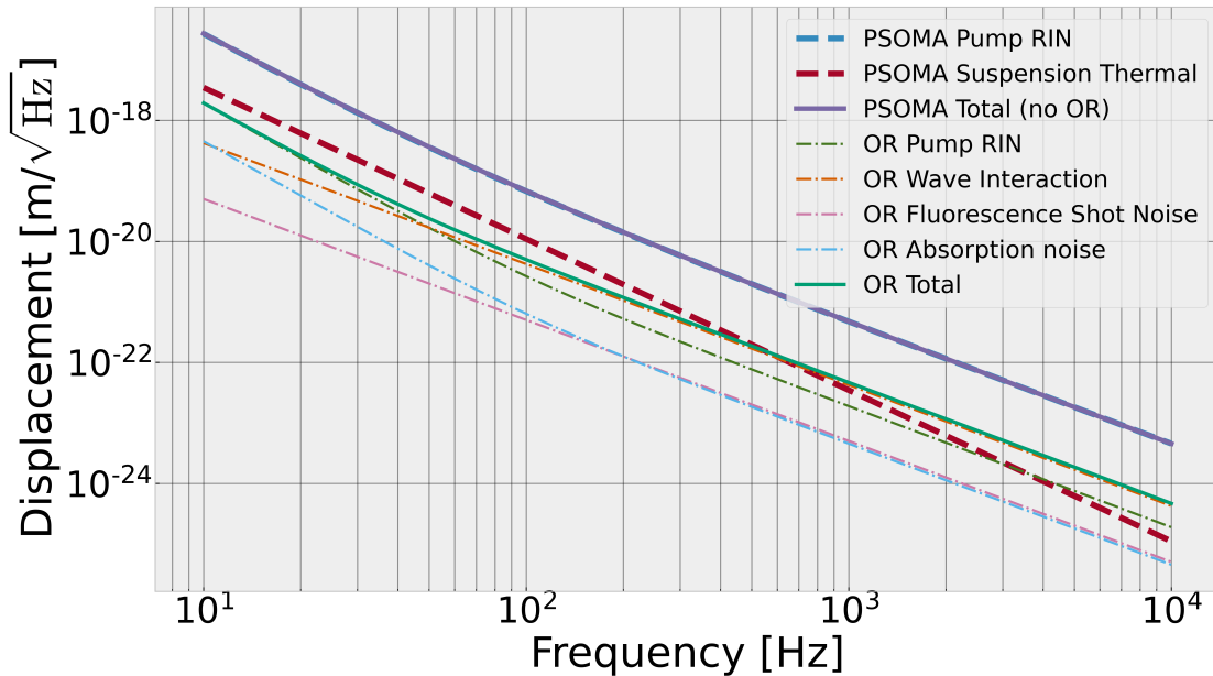
Figure 14: Noise curves for the noise introduced by the optical refrigerator plotted alongside existing displacement noise sources in PSOMA. We see that the OR does not significantly impact the noise budget. Note that the absorption noise is plotted here as if it were in the direction of the cavity axis, while in reality that would not be the case and the contribution of this noise source would be lower.
