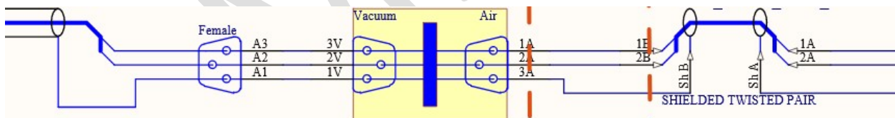
Figure 2: 3pin Shield Connections
