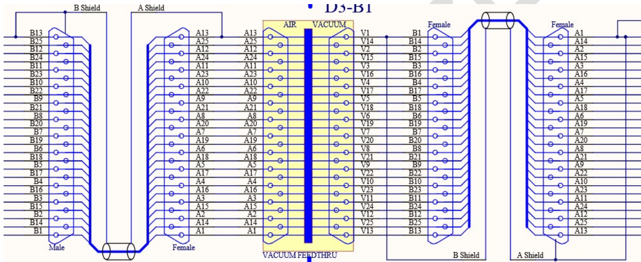
Figure 1: 25pin Shield Connections
