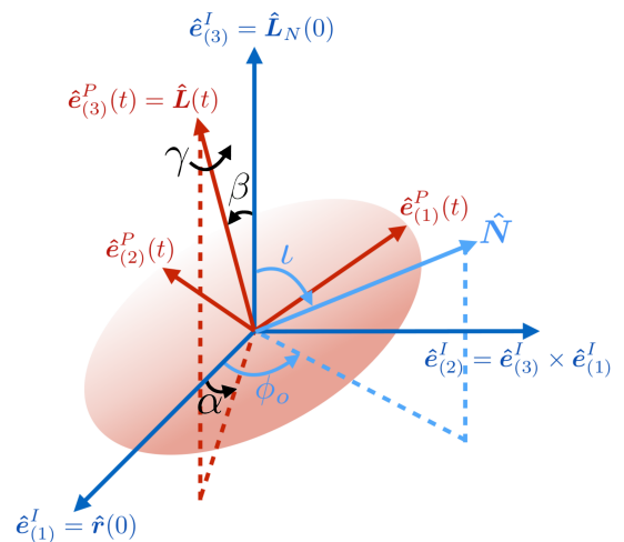
FIG. 5: Frames used in the construction of the SEOBNRv4PHM model: the observer’s frame (blue), defined by the directions of the initial orbital angular momentum \hat{\mathbf{L}}(0) and separation \mathbf{r}(0) , and co-precessing frame (red), instantaneously aligned with \hat{\mathbf{L}}(t) and described by the Euler angles (\alpha, \beta, \gamma) (see text below for details).
