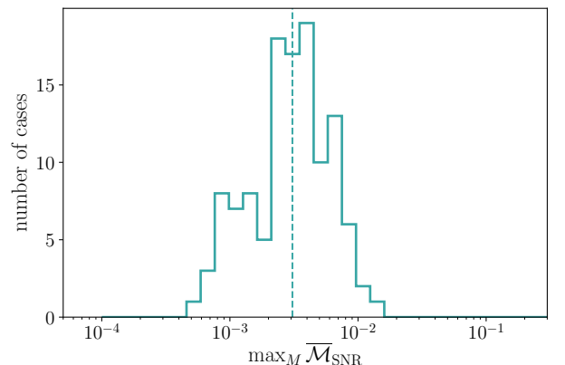
FIG. 4: The sky-and-polarization-averaged unfaithfulness between NR and symmetrized NR waveforms, maximized over the total mass for the new 118 NR precessing waveforms. The inclination used is \pi/3 . The vertical dashed line shows the median.
