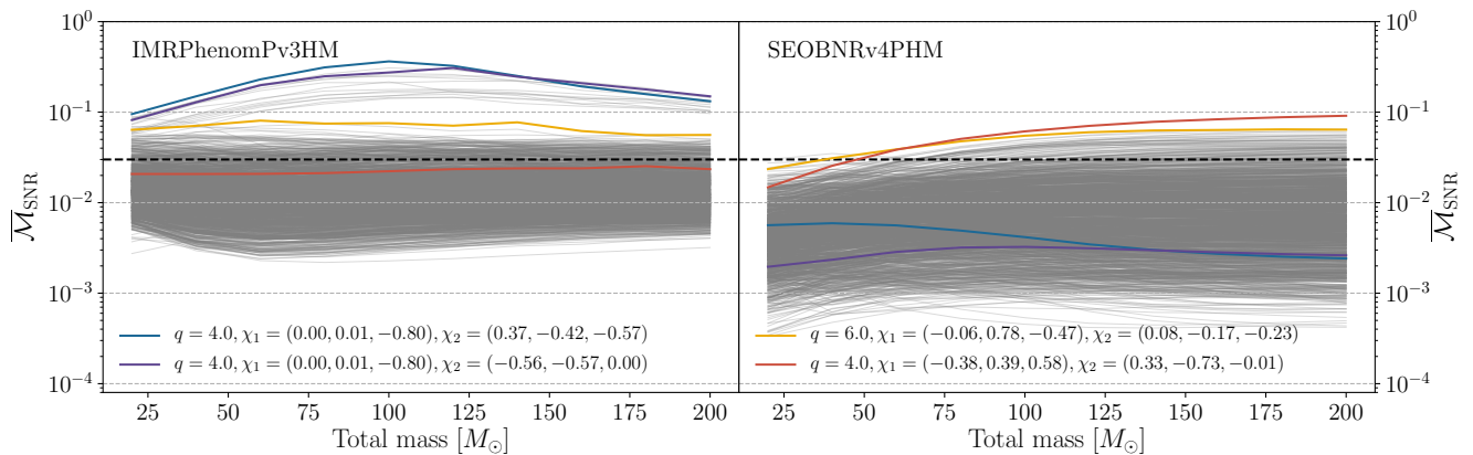
FIG. 10: The sky-and-polarization averaged, SNR-weighted unfaithfulness as a function of binary’s total mass for inclination \iota = \pi/3 , between IMRPhenomPv3HM and NR (left) and SEOBNRv4PHM and NR (right) for 1404 quasi-circular precessing BBH simulations in the SXS public catalog. The colored lines highlight the cases with the worst maximum mismatches for both models. Note that for the majority of cases, both models have unfaithfulness below 5%, but SEOBNRv4PHM has no outliers beyond 10% and many more cases at lower unfaithfulness.
