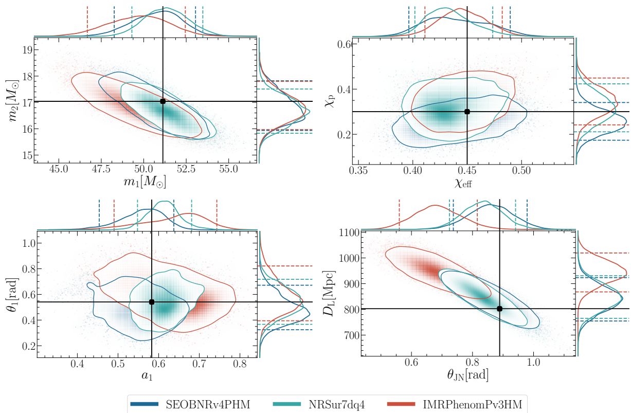
FIG. 15: 2D and 1D posterior distributions for some relevant parameters measured from the first synthetic BBH signal with mass ratio q = 3 , total source-frame mass of M = 70M_{\odot} , spins of the two BHs \chi_1 = (0.30, 0.00, 0.50) and \chi_2 = (0.20, 0.00, 0.30) defined at a frequency of 20 Hz. The inclination with respect to the line of sight of the BBH is \iota = \pi/3 . The other parameters are specified in the text. The signal waveform is generated with the waveform model NRSur7dq4. In the 2D posteriors, solid contours represent 90% credible intervals and black dots show the value of the parameter used in the synthetic signal. In the 1D posteriors they are represented respectively by dashed lines and black solid lines. The parameter estimation is performed with the waveform models SEOBNRv4PHM (blue), NRSur7dq4 (cyan) and IMRPhenomPv3HM (red). Top left : component masses in the source frame, Top right : \chi_{\text{eff}} and \chi_p , Bottom left : magnitude and tilt angle of the primary spin, Bottom right : \theta_{\text{JN}} and luminosity distance.
