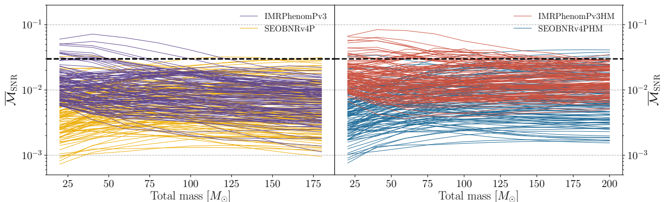
FIG. 11: The sky-and-polarization averaged, SNR-weighted unfaithfulness as a function of binary’s total mass for inclination \iota = \pi/3 , between IMRPhenomPv3 and SEOBNRv4P and NR (left), and IMRPhenomPv3HM and SEOBNRv4PHM and NR (right) for the 118 SXS NR waveforms described in Appendix B. The NR data has \ell = 2 modes for the left panel, while all modes up to and including \ell = 4 in the right panel. The unfaithfulness is low using both waveform families, however, SEOBNRv4P(HM) has fewer cases above 3%, and the distribution is consistently shifted to lower values of unfaithfulness.
