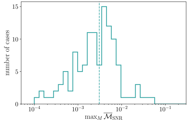
FIG. 2: The sky-and-polarization-averaged unfaithfulness between the highest and second highest resolutions in the NR simulation maximized over the total mass for the new 118 NR preprocessing waveforms. The inclination used is \pi/3 . The vertical dashed line shows the median.
