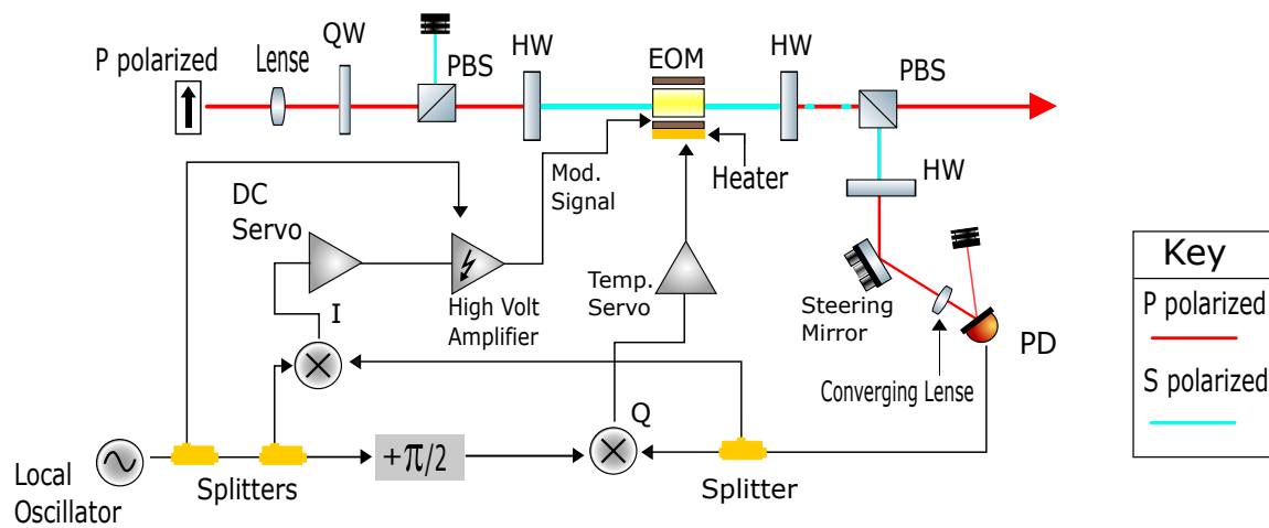
Figure 2: Experimental Set-up
