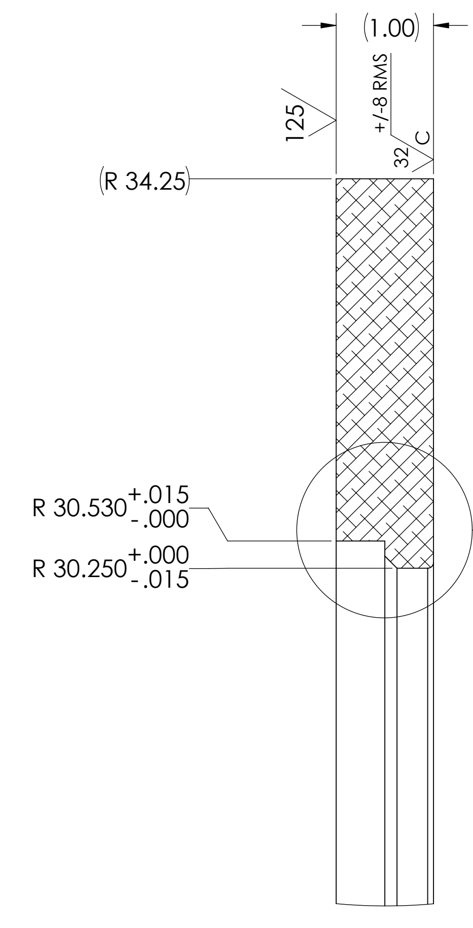
DETAIL H SCALE 1 : 1
