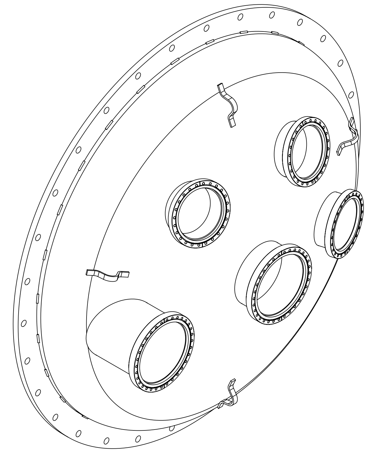
ISO VIEW
