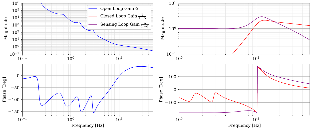
Figure 24: Transfer functions of the FC length control loop tuned for a 20 Hz UGF.
