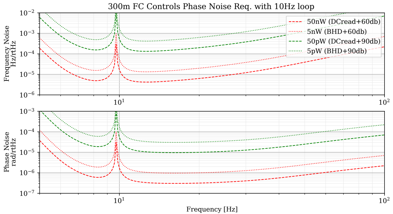
Figure 10: The phase noise requirements inferred from sensing noise injection within a 10Hz control loop.
