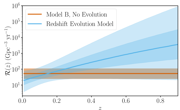
Figure 6. Constraints on evolution of the BBH merger rate density as a function of redshift. Including the 10 BBHs from O1 and O2 in our analysis, we find a preference for a merger rate that increases with increasing redshift. The solid blue line gives the posterior median merger rate density and dark and light bands give 50% and 90% credible intervals. In orange, the solid line and shaded region shows the median and 90% credible interval of the rate inferred for Model B as discussed in subsection 4.1, assuming a non-evolving merger rate.
