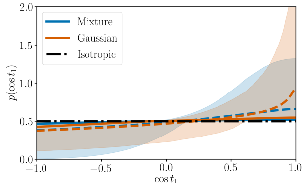
Figure 9. Inferred distribution of cosine spin tilt for the more massive black hole for two choices of prior (see Section 2.4). The dash-dotted line denotes a completely isotropic distribution (see Appendix B). The solid lines show the median. The shaded regions denote the 90% symmetric intervals and the dashed line denotes the PPD.
