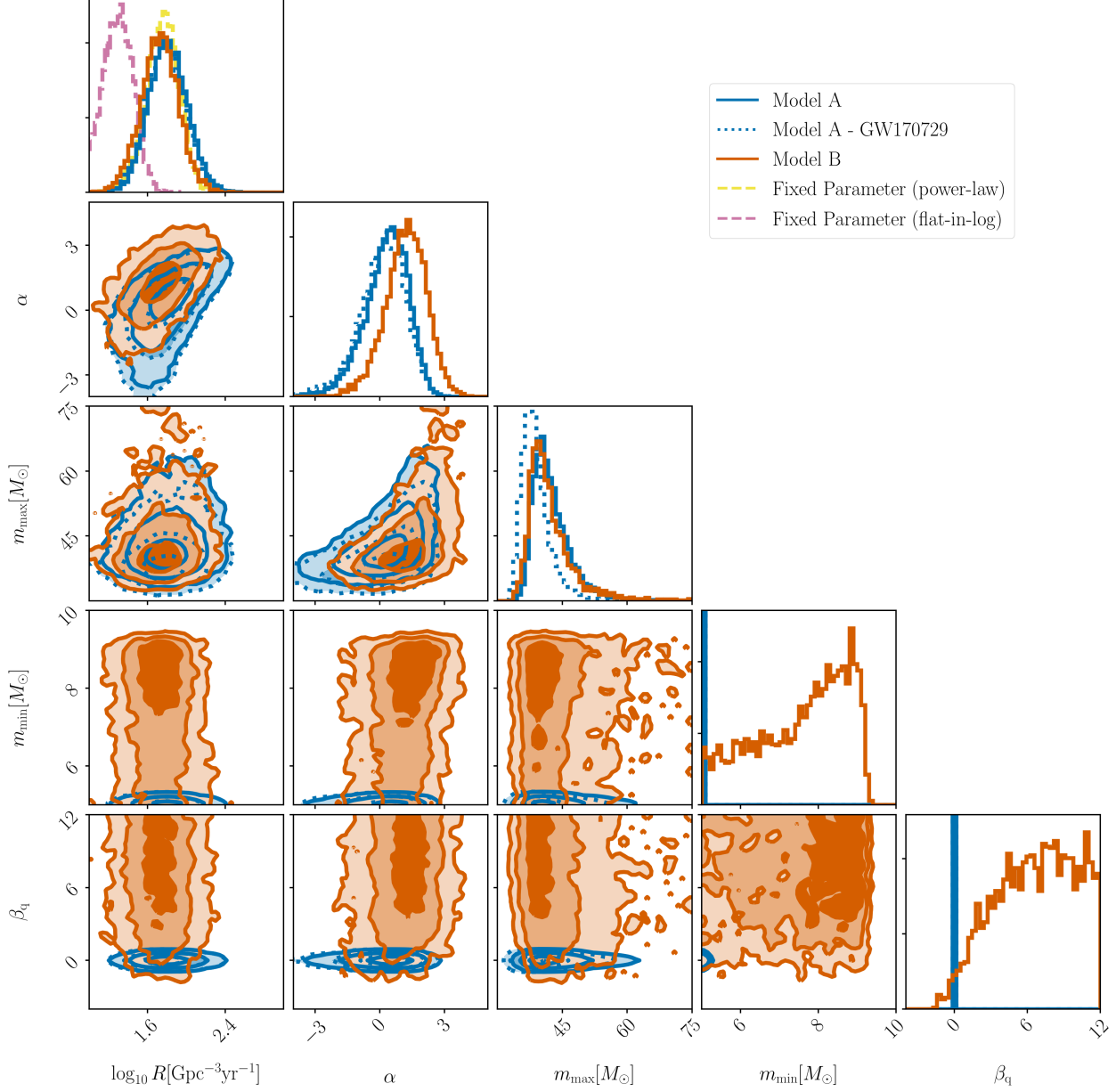
Figure 3. One- and two-dimensional posterior distributions for the hyperparameters describing Models A and B. Large values of \alpha correspond to a mass distribution which rapidly decays with increasing mass. Large values of \beta correspond to a mass-ratio distribution which prefers equal mass binaries. Also shown is the one-dimensional posterior distribution for the merger rate discussed in Abbott et al. (2018), and the stability of Model A to the removal of the GW170729 event.
