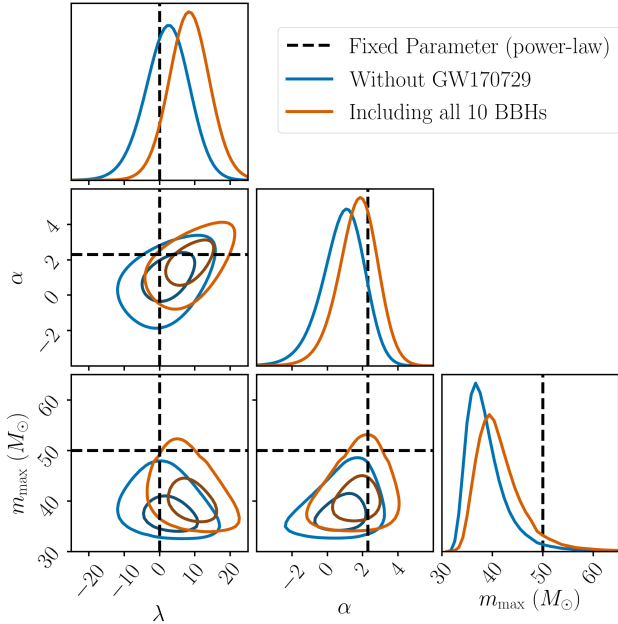
Figure 7. The posterior PDF on the redshift evolution parameter \lambda , mass power-law slope \alpha , and maximum mass m_{\max} , marginalized over the local rate parameter R_0 , and assuming a flat prior on \lambda , \alpha , and m_{\max} and a flat-in-log prior on R_0 . In order to analyze the stability of the model against outliers, we repeat the analysis once with the sample of 10 BBHs (results shown in blue), and once excluding the most distant and massive event in our sample, GW170729 (results shown in red). The contours show 50% and 90% credible intervals. The dashed black lines show the values of hyper-parameters assumed for the fixed-parameter power-law model. We infer a redshift evolution that is consistent with a flat in comoving volume and source-frame time merger rate ( \lambda = 0 ) with a preference for \lambda \geq 0 at 0.93 credibility when considering all 10 events. This preference becomes less significant with the exclusion of GW170729 from the analysis. The inferred power-law slope and maximum mass is consistent with the values inferred in Section 3. This analysis recovers a broader posterior on the mass power-law slope because of the correlation with the redshift evolution parameter, but the maximum mass remains well-constrained at \lesssim 45M_{\odot} .
