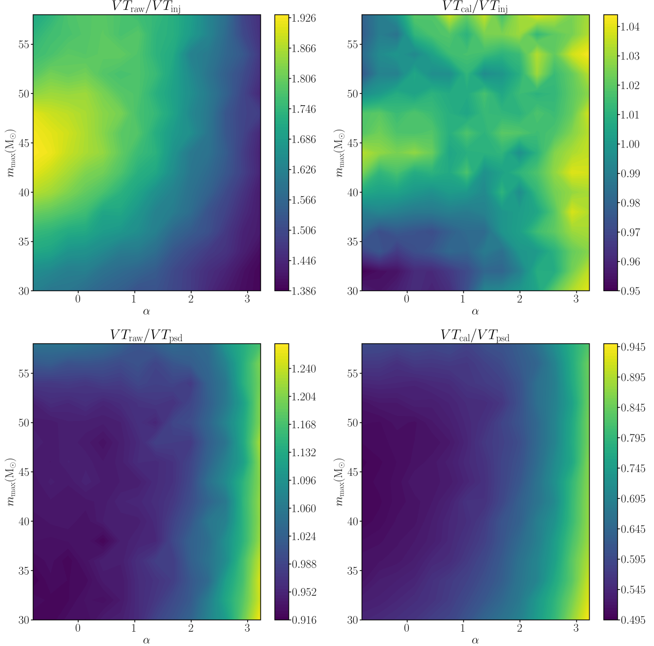
Figure 11. Ratio between the raw semi-analytic computation of \langle VT \rangle to the \langle VT \rangle computed by injections into the PyCBC search pipeline (top left panel), and the same ratio for the mass-calibrated \langle VT \rangle (top right panel), for different mass distributions described by the two-parameter Model A. The bottom panel shows the same ratios, but this time comparing the \langle VT \rangle derived with the time-varying PSDs applied to the semi-analytic calculation VT_{\text{psd}} to the raw and the calibrated \langle VT \rangle . The \langle VT \rangle for the injections is calculated for a threshold of \varrho = 8.0 , where \varrho is the signal-noise model statistic used in the PyCBC analysis of O2 data. This threshold roughly matches the detection statistic of the lowest significance detection, GW170729, which has \varrho = 8.7 in PyCBC. We use the mass-calibrated VT_{\text{cal}} for the parametric mass- and spin-distribution analyses in Section 3 and 5 in order to better match the injection results, while the redshift evolution analysis uses VT_{\text{psd}} in order to carefully track the sensitivity at high redshift. The discrepancy between the methods may be due to the limited number of high-redshift injections. However, the difference between all three methods is relatively constant as a function of the mass population, particularly where posterior support for the mass distribution hyper-parameters is high, indicating that systematic uncertainties in the \langle VT \rangle estimation do not have a large impact on our results.
