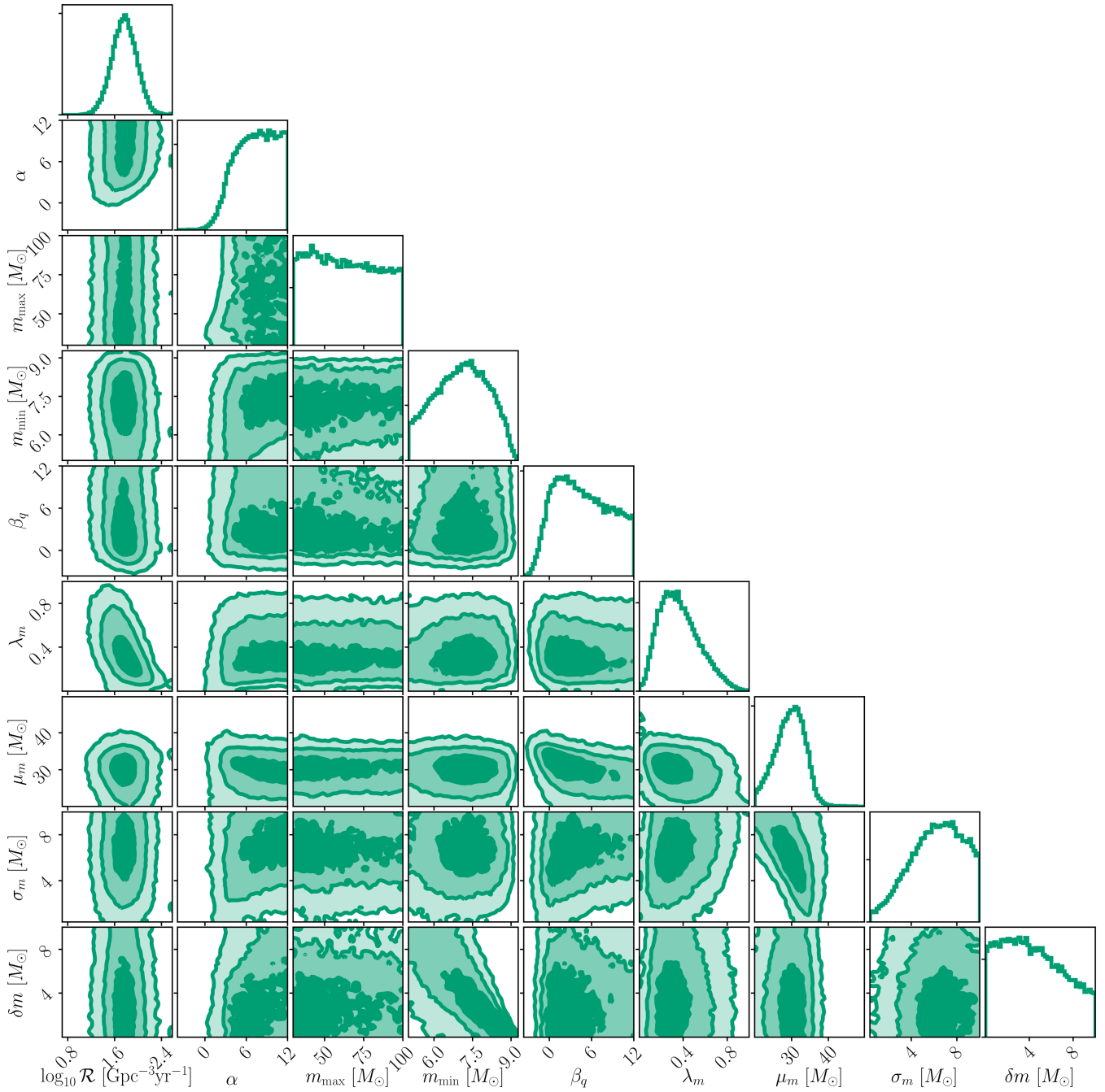
Figure 4. One- and two-dimensional posterior distributions for the hyperparameters describing Model C. This model consists of the power-law distribution in Model B with an additional Gaussian component at high mass. The parameters \alpha , \beta , m_{\text{max}} , and m_{\text{min}} describe the power-law component. The Gaussian has mean \mu_m and standard deviation \sigma_m . The fraction of black holes in the Gaussian component is \lambda_m . This model also allows for a gradual turn-on at low masses over a mass range \delta m .
