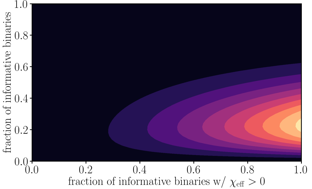
Figure 14. Posterior distribution for the fraction of informative binaries (i.e., |\chi_{\text{eff}}| > 0.05 ), and the fraction of those informative binaries with positive \chi_{\text{eff}} (i.e., \chi_{\text{eff}} > 0.05 ).
