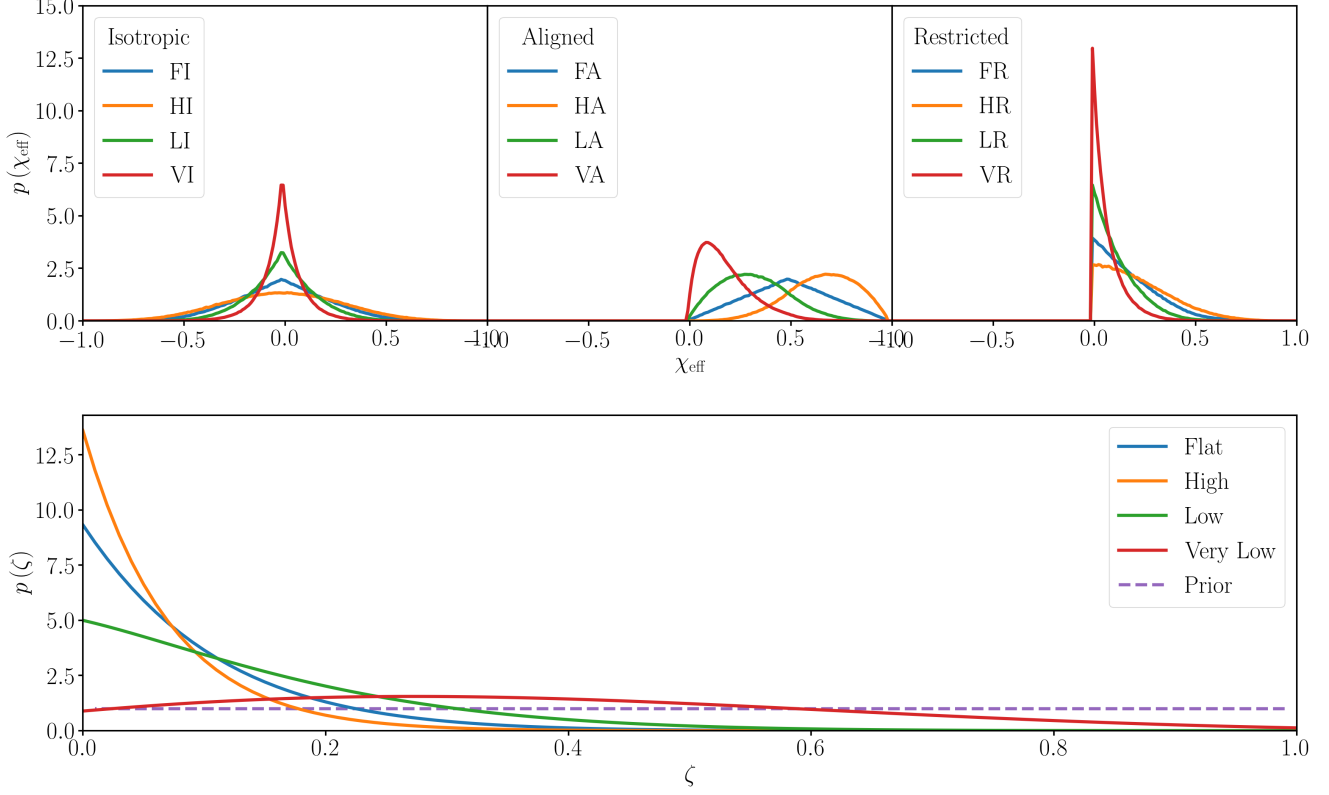
Figure 13. Upper row: p(\chi_{\text{eff}}) under various model assumptions. Labels in each subpanel legend correspond to the tilt and magnitude models defined in B.1. Isotropic models (left) provide support for both negative and positive \chi_{\text{eff}} . Aligned models (center) assume perfect alignment for each of the four magnitudes distributions. Restricted models (right) have the same shape as the Isotropic ones, with support over \chi_{\text{eff}} > 0 only. However they can be generated with nonprecessing spins. Bottom row: Posterior on the mixture fraction \zeta between isotropic and aligned distributions. \zeta = 0 corresponds to a completely isotropic distribution.
