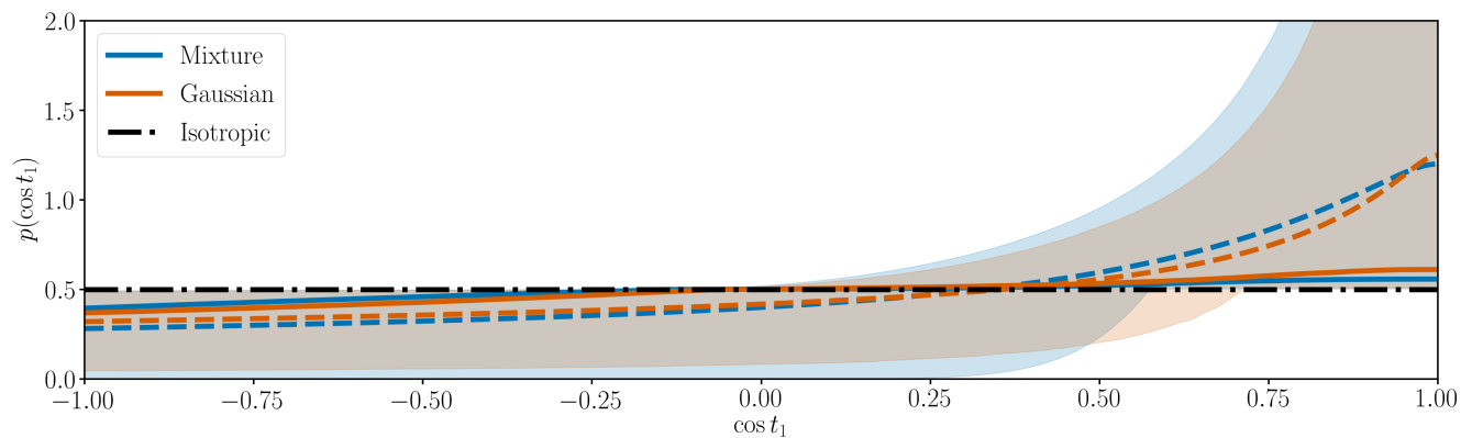
Figure 10. Inferred distribution of cosine spin tilt for the more massive black hole for two choices of prior (see Section 2.4 ) with the SEOBNRv3 waveform model, with the same definitions as Figure 9 .
