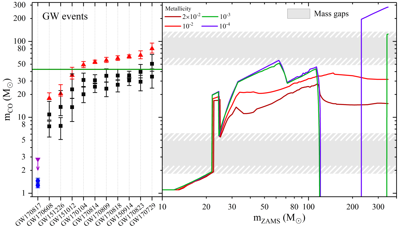
Figure 5. The left-hand panel shows compact object masses ( m_{\text{CO}} ) from GW detections in O1 and O2, with the black squares and error bars representing the component masses of the merging black holes and their uncertainties, and red triangles representing the mass and associated uncertainties of the merger products. The horizontal green line shows the 99th percentile of the mass distribution inferred from the Model B PPD. In the right-hand panel, the predicted compact-object mass is shown as a function of the zero-age main sequence mass of the progenitor star ( m_{\text{ZAMS}} ) and for four different metallicities of the progenitor star (ranging from Z = 10^{-4} to Z = 2 \times 10^{-2} , Spera & Mapelli 2017). This model accounts for single stellar evolution from the PARSEC stellar-evolution code (Bressan et al. 2012), for core-collapse supernovae (Fryer et al. 2012), and for pulsational-pair instability and pair-instability supernovae (Woosley 2017). The shaded areas represent the lower and upper mass gaps. There is uncertainty as to the final product of GW170817. It is shown in the left-hand panel to emphasize that BNS mergers might fill the lower gap.
