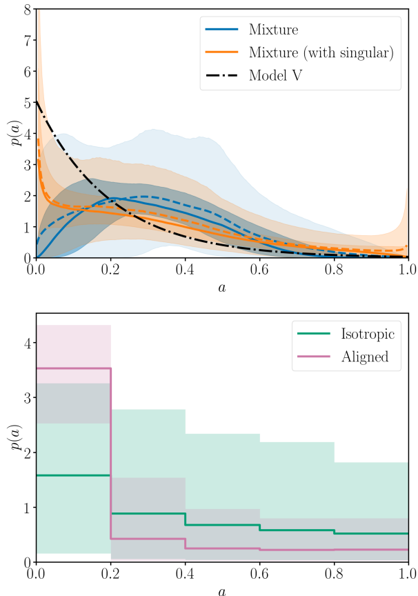
Figure 8. Inferred distribution of spin magnitude for a parametric (top) and non-parametric binned model (bottom). Both component magnitudes are included in these distributions. The solid lines show the median and the dashed line shows the PPD. The shaded regions denote the 50% and 90% symmetric intervals. In the upper panel, the parametric model is presented with both singular (orange) and non-singular (blue) model configurations. For comparison purposes, the V (very low spin magnitude) model is plotted in a dash-dotted black line. In the bottom panel, the distribution of spin magnitude is inferred over five bins, assuming either perfectly aligned (pink) or isotropic (green) population. The solid lines denote the median, and the shaded regions denote the central 90% posterior credible bounds. In both cases, the magnitude is consistent within the uncertainties with the parametric (singular and non-singular) results. The number of bins in the model were chosen to balance resolution with the amount of information in the data; analyses with more bins do not indicate any additional features in the spin distributions.
