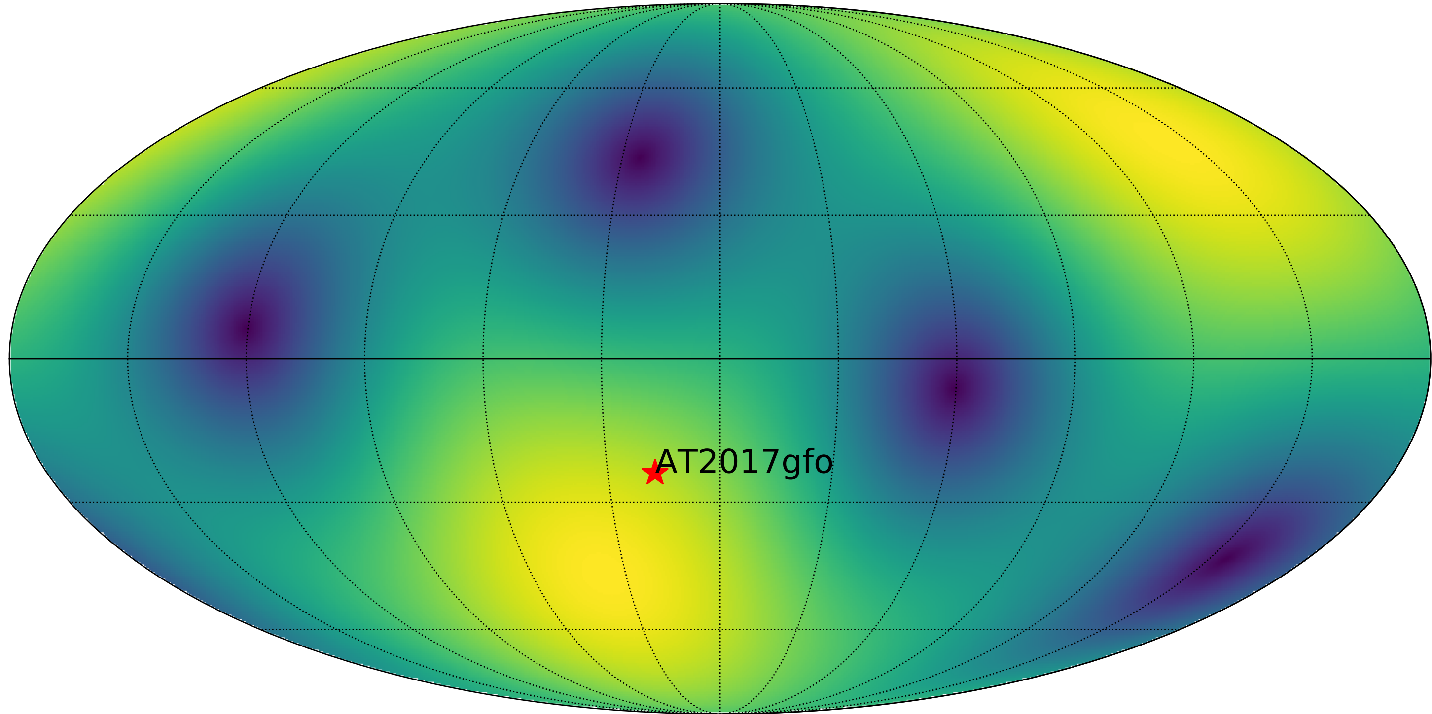
LIGO Hanford beam pattern
