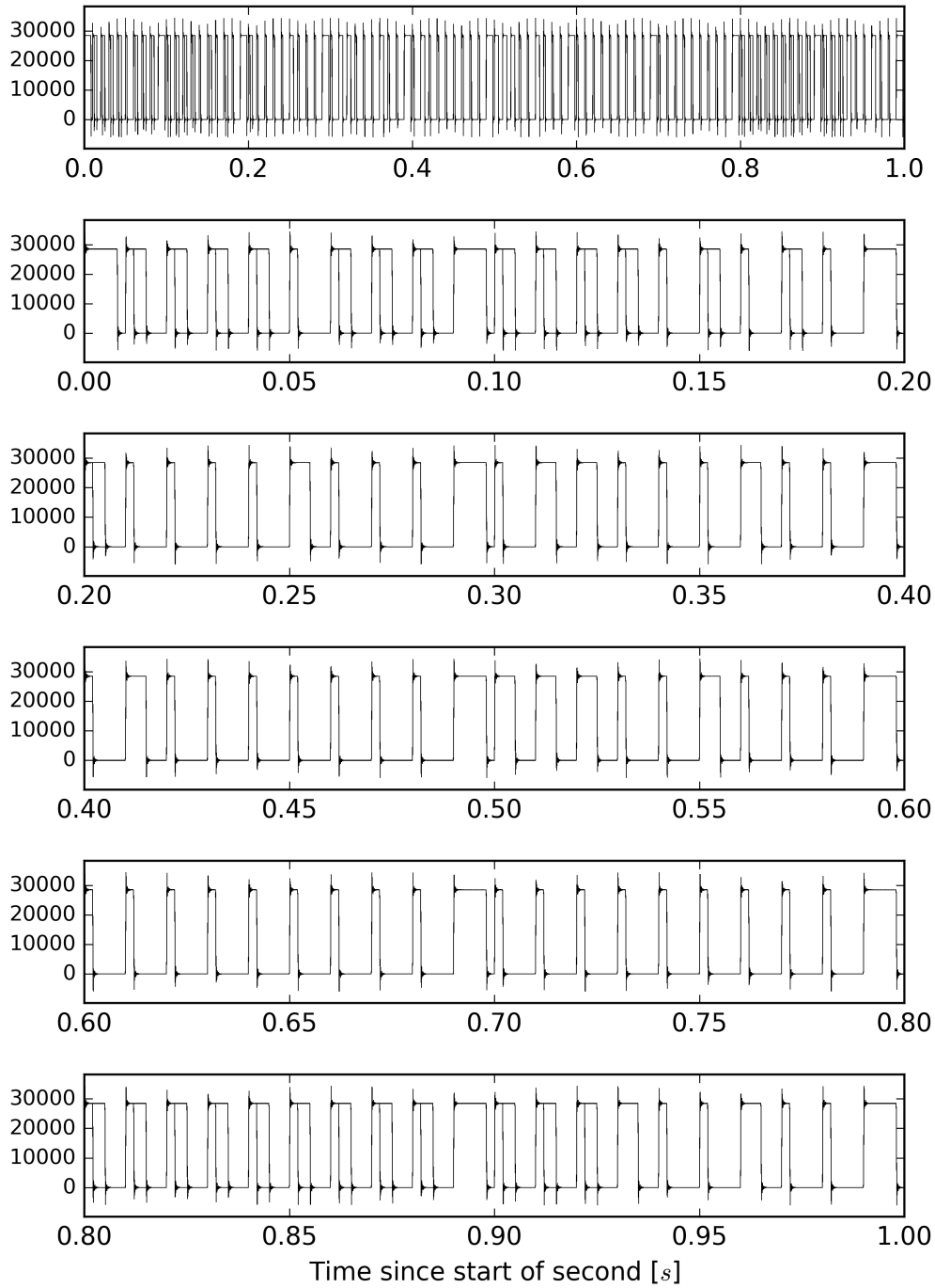
Overlay of L1:CAL-PCALX_IRIGB_OUT_DQ from 1186744560 to 1186744561
