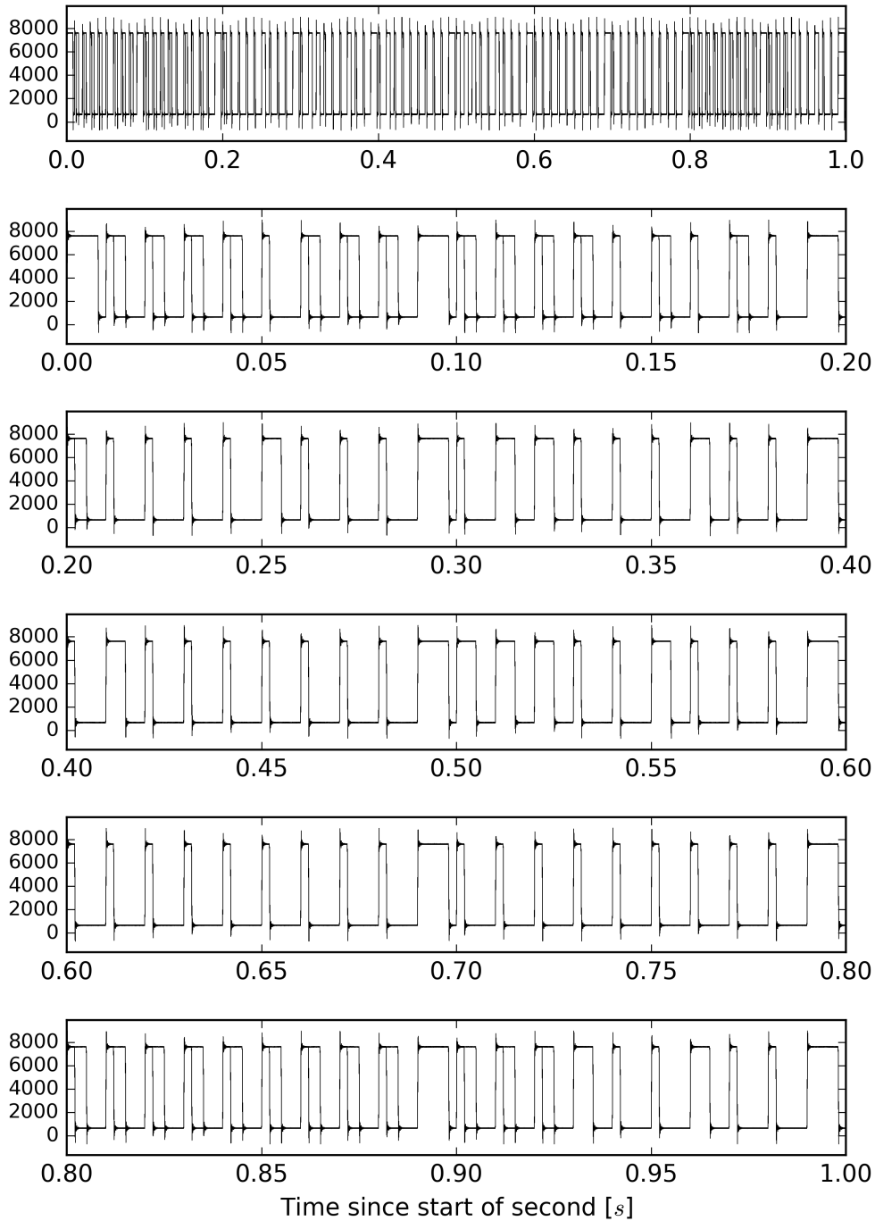
Overlay of H1:CAL-PCALY_IRIGB_OUT_DQ from 1186744560 to 1186744561
