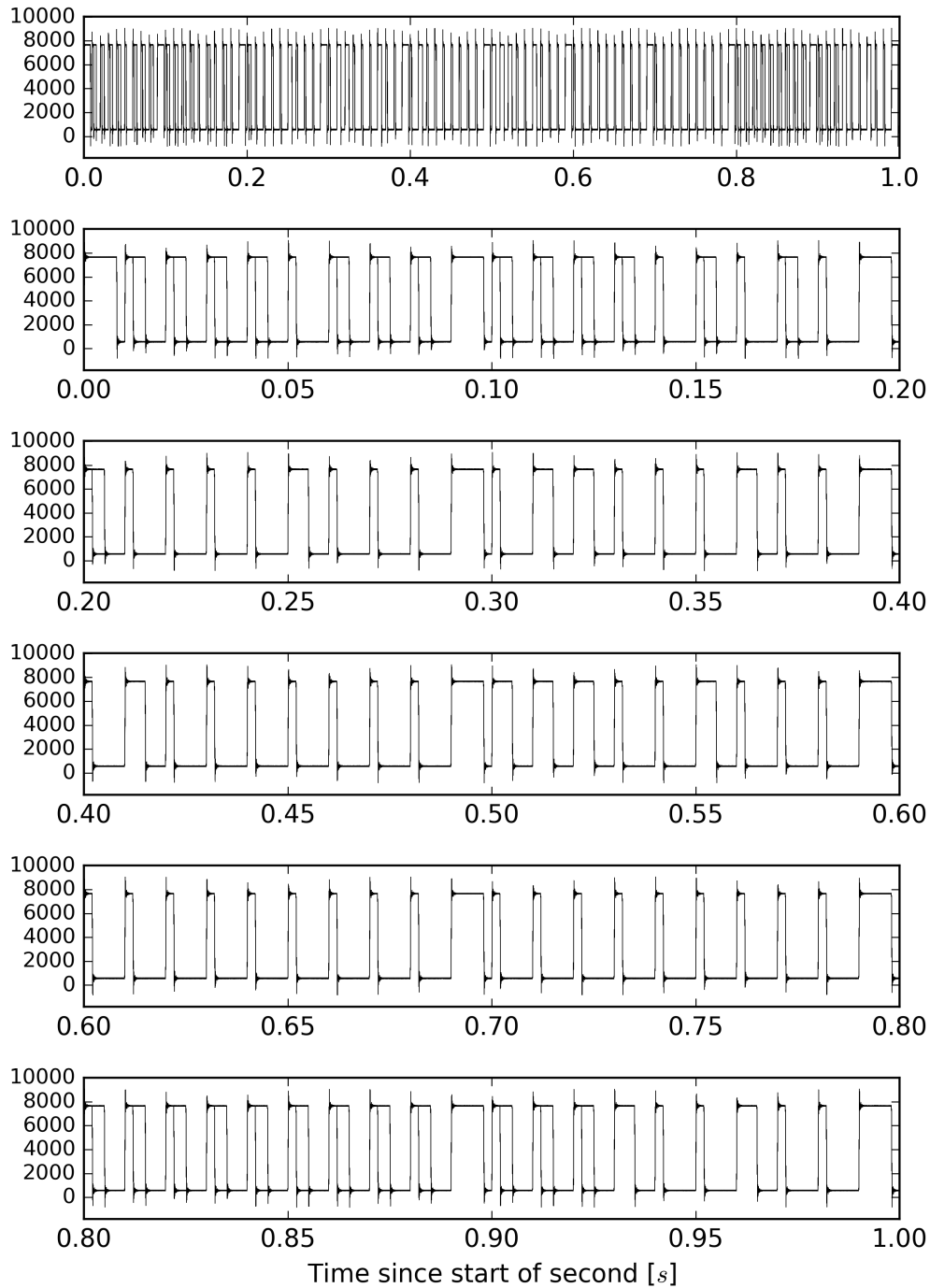
Overlay of H1:CAL-PCALX_IRIGB_OUT_DQ from 1186744560 to 1186744561
