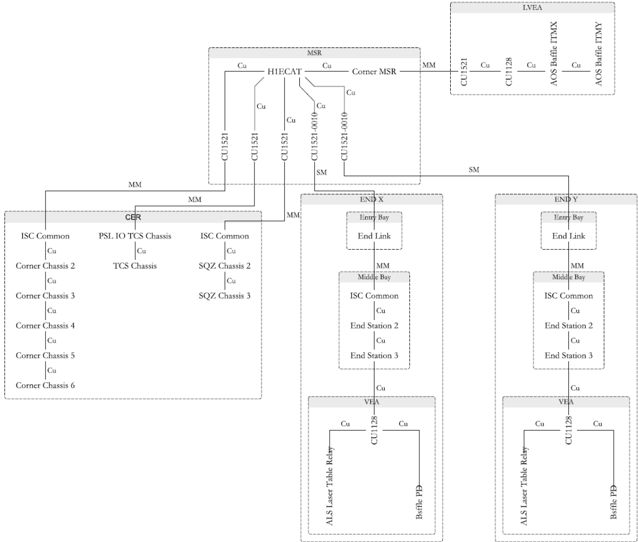
Figure 1: New star topology for the main EtherCAT system.
