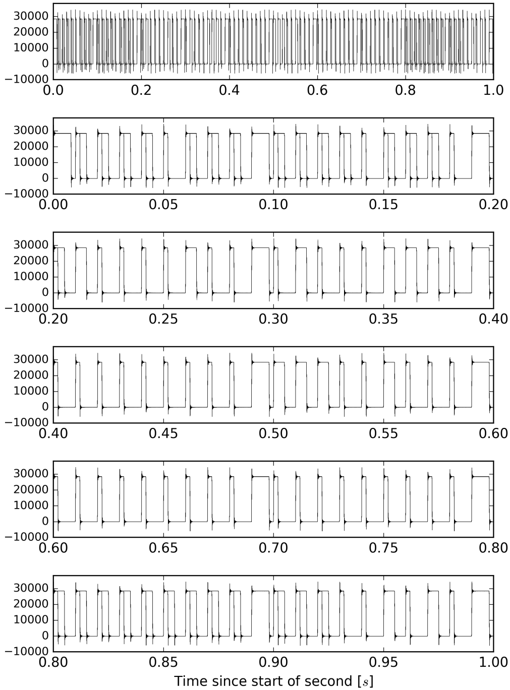
Overlay of L1:CAL-PCALY_IRIGB_OUT_DQ from 1173482726 to 1173482727
