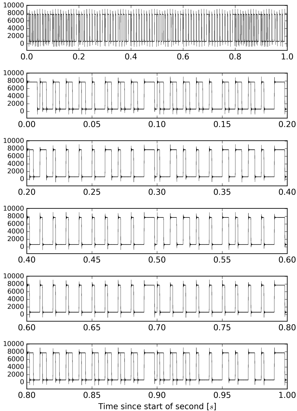
Overlay of H1:CAL-PCALX_IRIGB_OUT_DQ from 1173482726 to 1173482727
