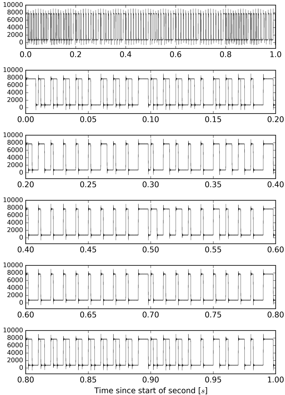
Overlay of H1:CAL-PCALY_IRIGB_OUT_DQ from 1173482726 to 1173482727
