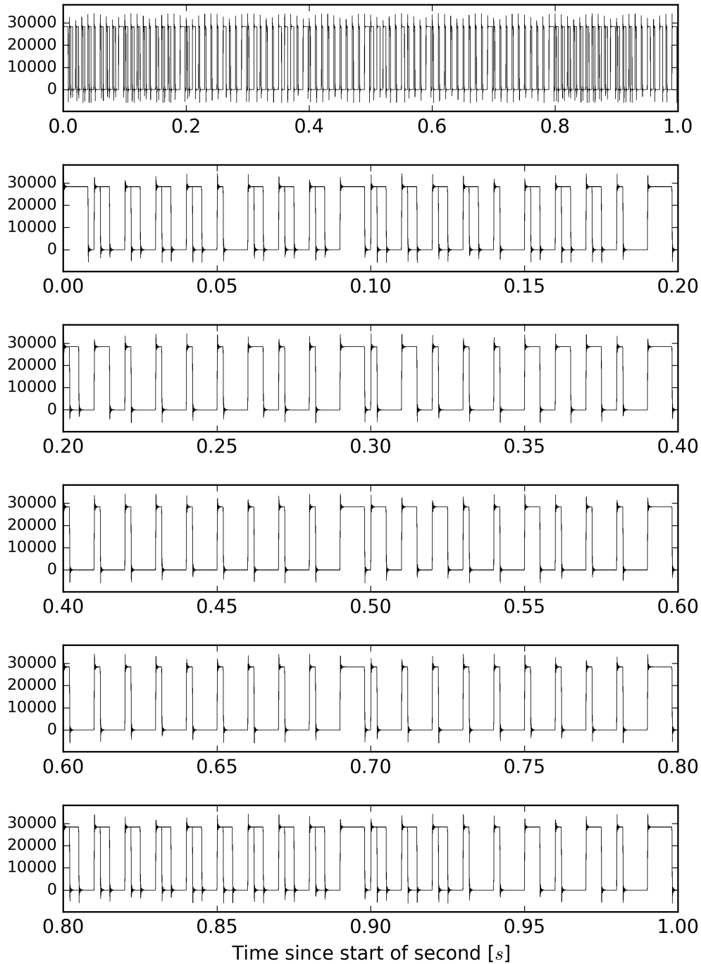
Overlay of L1:CAL-PCALX_IRIGB_OUT_DQ from 1173482726 to 1173482727
