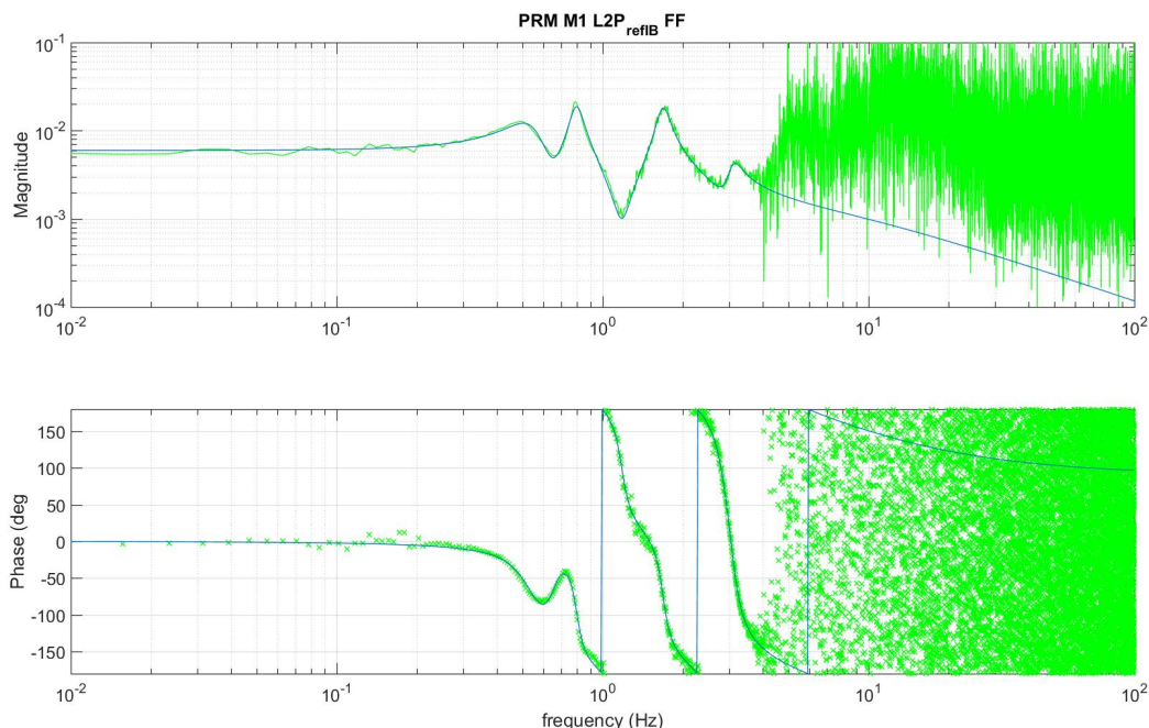
Figure 30: Local feedforward correction filter for length-to-pitch decoupling for the Power Recycling Mirror (PRM), M1 stage. Trend data indicates improved robustness to disturbances (wind, earthquakes) after implementing length-to-pitch (L2P) and length-to-yaw (L2Y) feedforward (FF) filters from the ReflB photodiode for the PRM.
