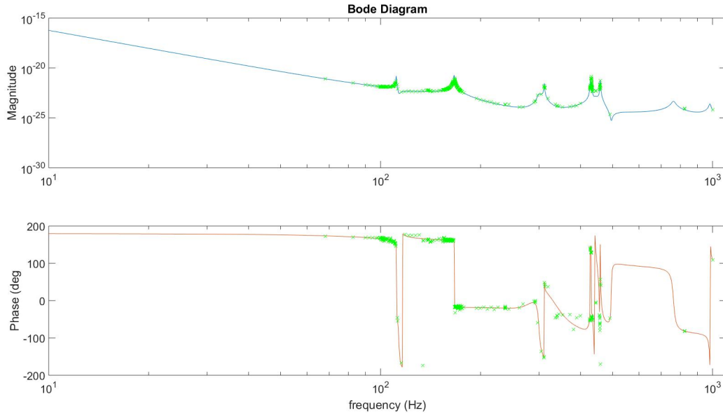
Figure 31: High Frequency Suspension Dynamics: A number of dynamical, resonant features have been found in the quadruple pendulum suspension (UIM/L1 actuation stage) in the frequency range of 100 to 500 Hz. Measurements are a combination of swept-sine (SS) and broad-band (BB) transfer function ratios. For system calibration, a pole-zero fit of this transfer function above 20 Hz, that can be used as a "correction" filter to a model that falls off as f^6 , was needed. While this filter does not need to perfectly resolve the details of all of the high-Q features, but it must track the overall frequency dependence over the 20 - 500 Hz region well. The best pole:zero fit is the stable, non-minimum phase, zero delay, 22:28 order model shown (compatible with a Linear Time Invariant (LTI) representation).
