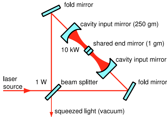
Figure 26: Ponderomotive Squeezer, taken from Corbitt et al. [7]
