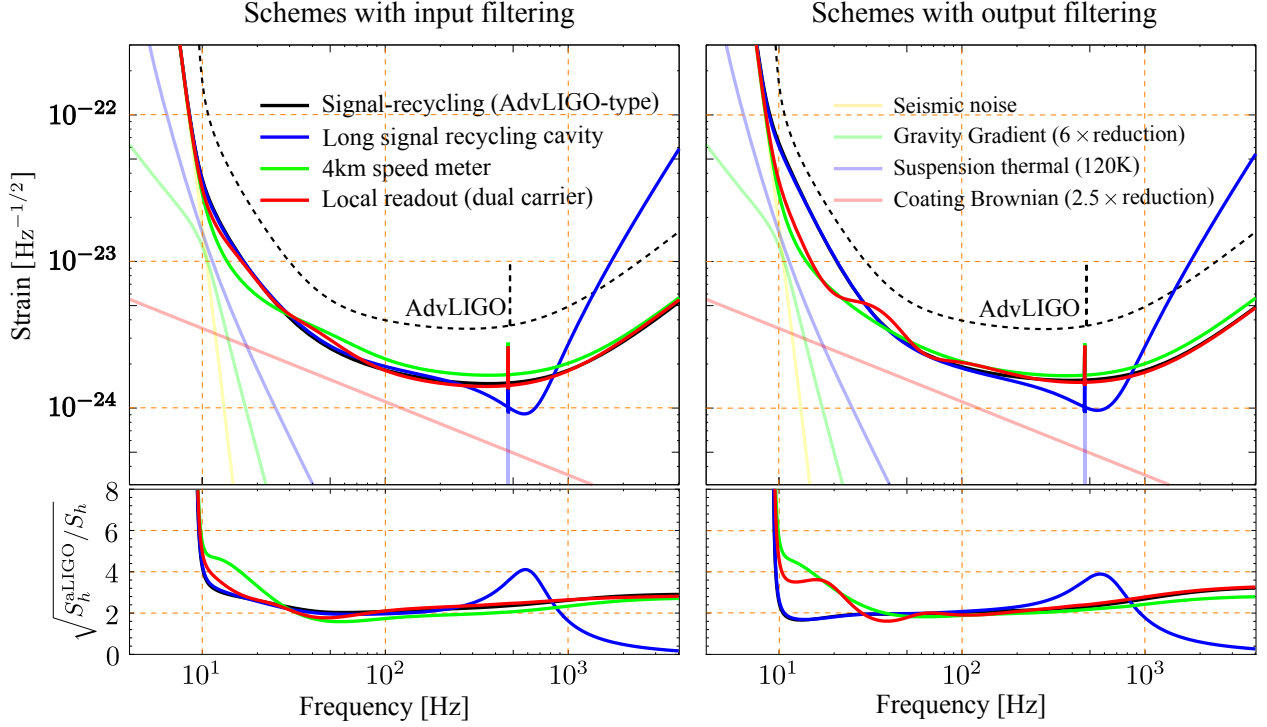
Figure 24: The optimized total noise spectrum for different schemes assuming a moderate improvement of the thermal noise compared with aLIGO baseline design. The lower panels show the linear strain sensitivity improvement over aLIGO.
