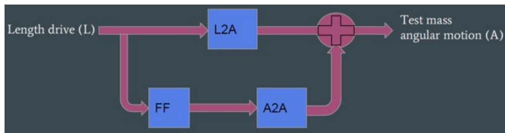
Figure 29: Local feedforward correction filter for length-to-angle decoupling. FF = -L2A/A2A .
