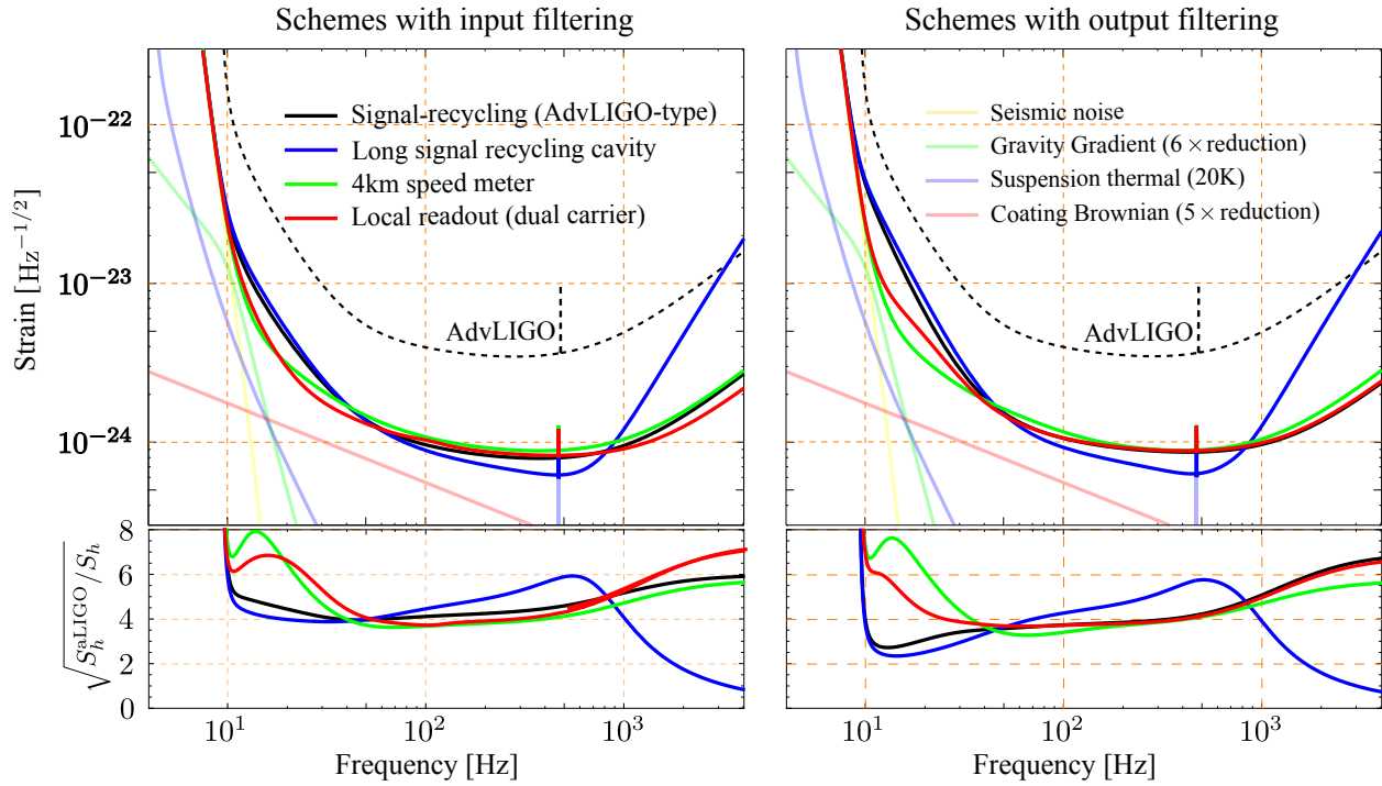
Figure 25: Optimization results for different schemes assuming more substantial thermal noise improvements, increasing the mirror mass from 40 to 150 kg, and increasing the arm cavity power from 800 to 3000 kW.
