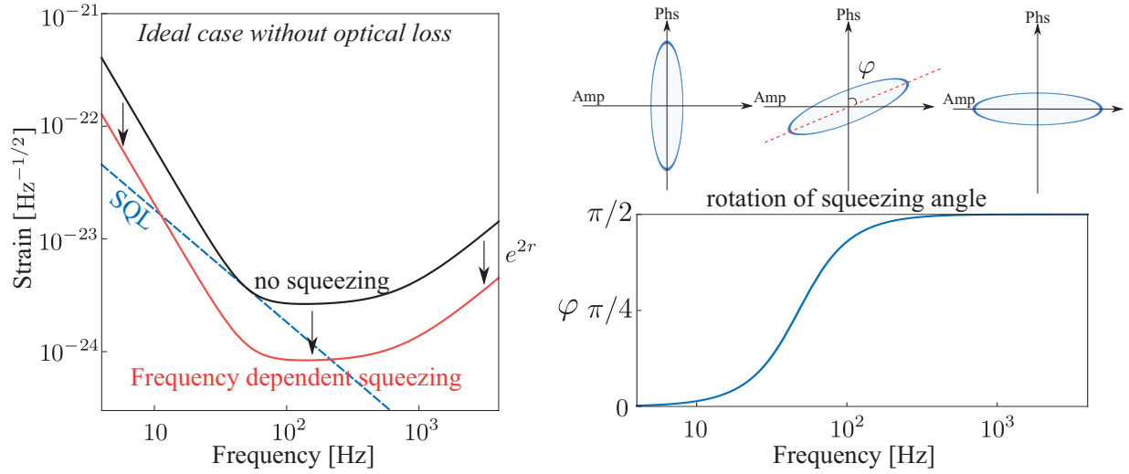
Figure 15: Noise spectrum for frequency-dependent squeezing (left) and rotation of the squeeze angle (right).
