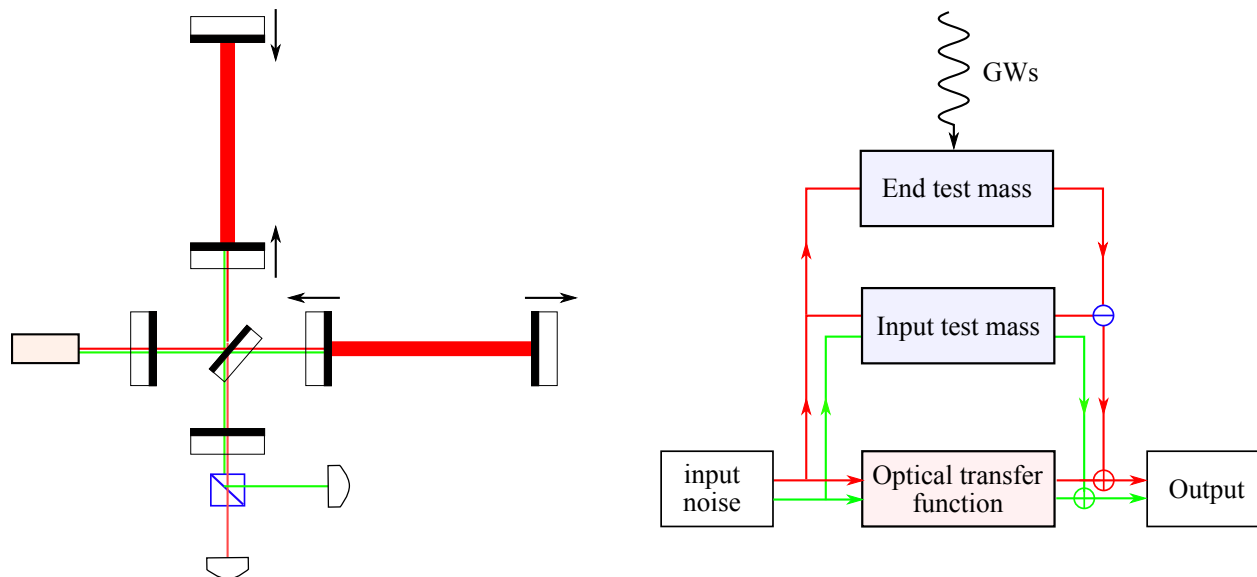
Figure 23: Diagram of the local-readout topology (left) and the resulting feedback loops (right).
