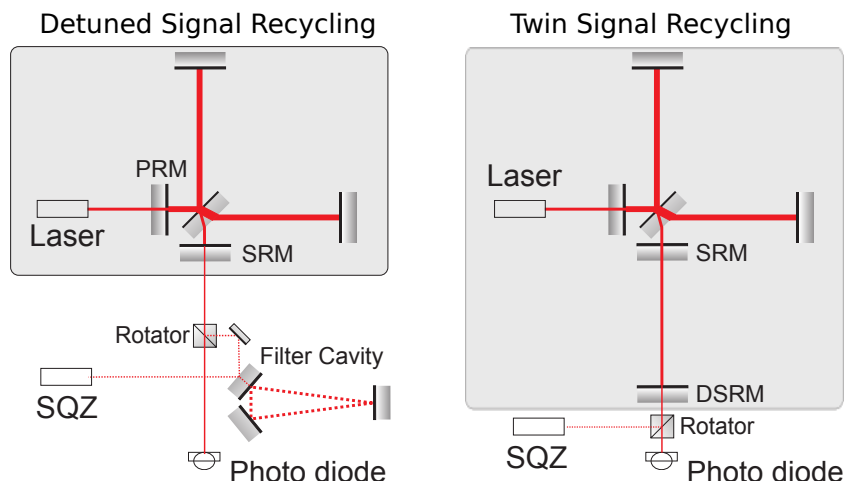
Figure 20: (Color online) Top left (shaded): Topology of the current gravitational wave detector GEO 600. The mirror in the laser input port (PRM) realizes so-called power-recycling. The signal-recycling mirror (SRM) in the output port establishes a carrier light detuned single-sideband signal recycling cavity. Bottom left: Extension for a broadband shot-noise reduction utilizing squeezed states. Right: Topology, proposed here. Two optically coupled cavities are formed with the help of an additional mirror DSRM. Their resonance doublet enables detuned dual-signal-recycling resulting in lower shot noise. Squeezed states can be used without additional filter cavity.
