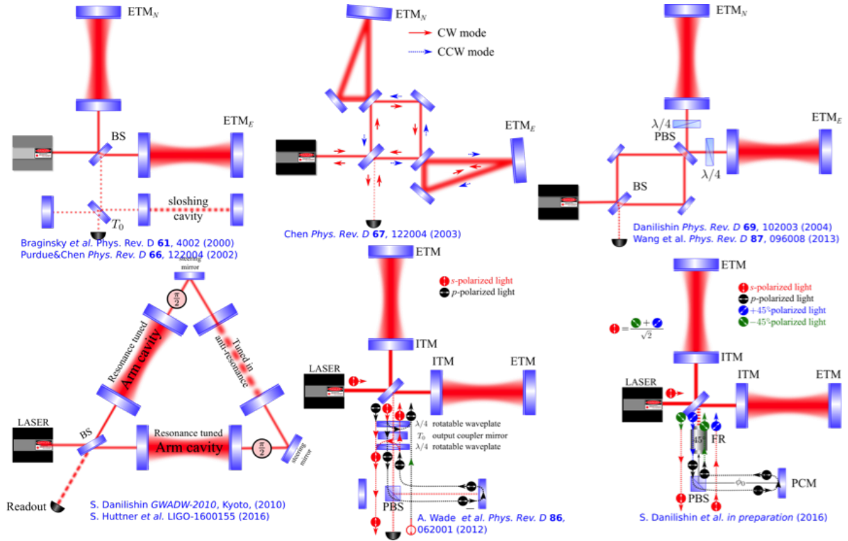
Figure 10: Different incarnations of speed meters [3, 4, 5].
