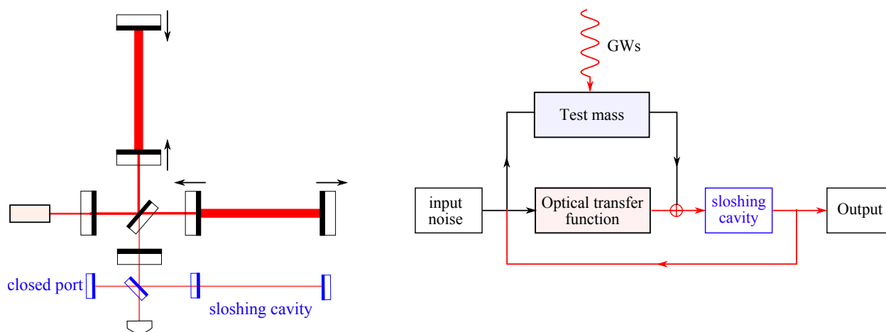
Figure 21: Schematics showing a speed-meter configuration (left) and its flow chart (right).
