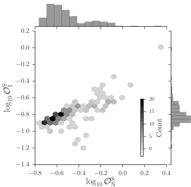
FIG. 2. Log-odds distributions. Distributions of log-odds comparing the any-signal hypothesis to the instrumental (ordinate axis, right) and Gaussian noise (abscissa axis, top) hypotheses for all pulsars. This plot contains the same information as Fig. 1 and displays the same non-significant outlier. These results were obtained without incorporating any information on the source orientation, and are tabulated in Table II in the supplementary material [40]. Expressions for both odds in this plot are given in Eq. (10) and Eq. (12). We underscore that, although this plot looks similar to Fig. 2 in [25], the signal hypothesis here incorporates scalar, vector and tensor modes, in all possible combinations.
