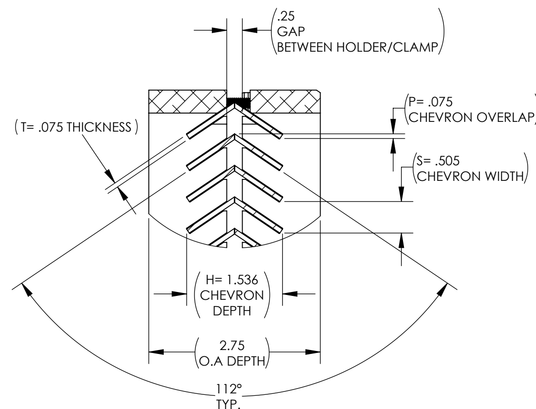
DETAIL B SCALE: ENLARGED (SEE LIGO T1600426 FOR REFERENCE)
