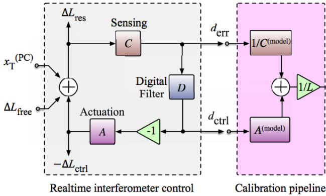
FIG. 5.— A block diagram of the DARM feedback control servo from [20]. This schematic shows that aLIGO’s output is dependent on the performance of the feedback loop. Each component of the feedback loop is described by a transfer function and the uncertainty on the overall loop transfer function yields the CEs on the GW strain detection. The transfer functions of all of the components in the feedback loop are necessary to reconstruct the GW signal. The subsystems are described more thoroughly in [15, 20].
