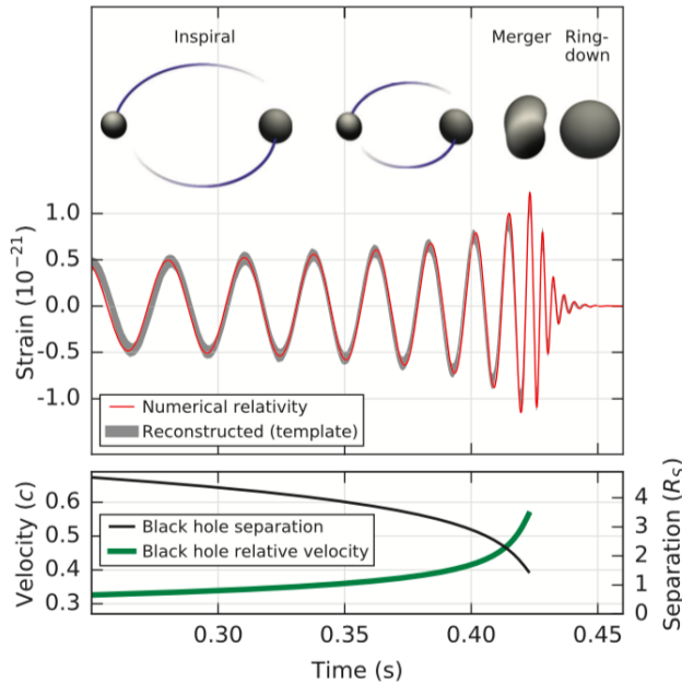
FIG. 4.— A figure illustrating an inspiral-merger-ringdown of a compact binary system from [2]. According to GR, two objects in orbit will slowly spiral inwards due to a loss of energy and angular momentum via GWs. The frequency and amplitude of the emitted GWs increases as the orbital distance between the objects shrink. When the objects finally merge they can radiate GWs as a superposition of quasinormal ringdown modes. One mode will eventually dominate with an exponentially damped, constant frequency wave [4]. We observe this as a lower frequency inspiral phase, a post-merger peak at some fixed frequency, and then a higher frequency ringdown. In this work we investigate the differences due to non-GR conformity as described in a parameter pertaining to the ringdown of the GW.
