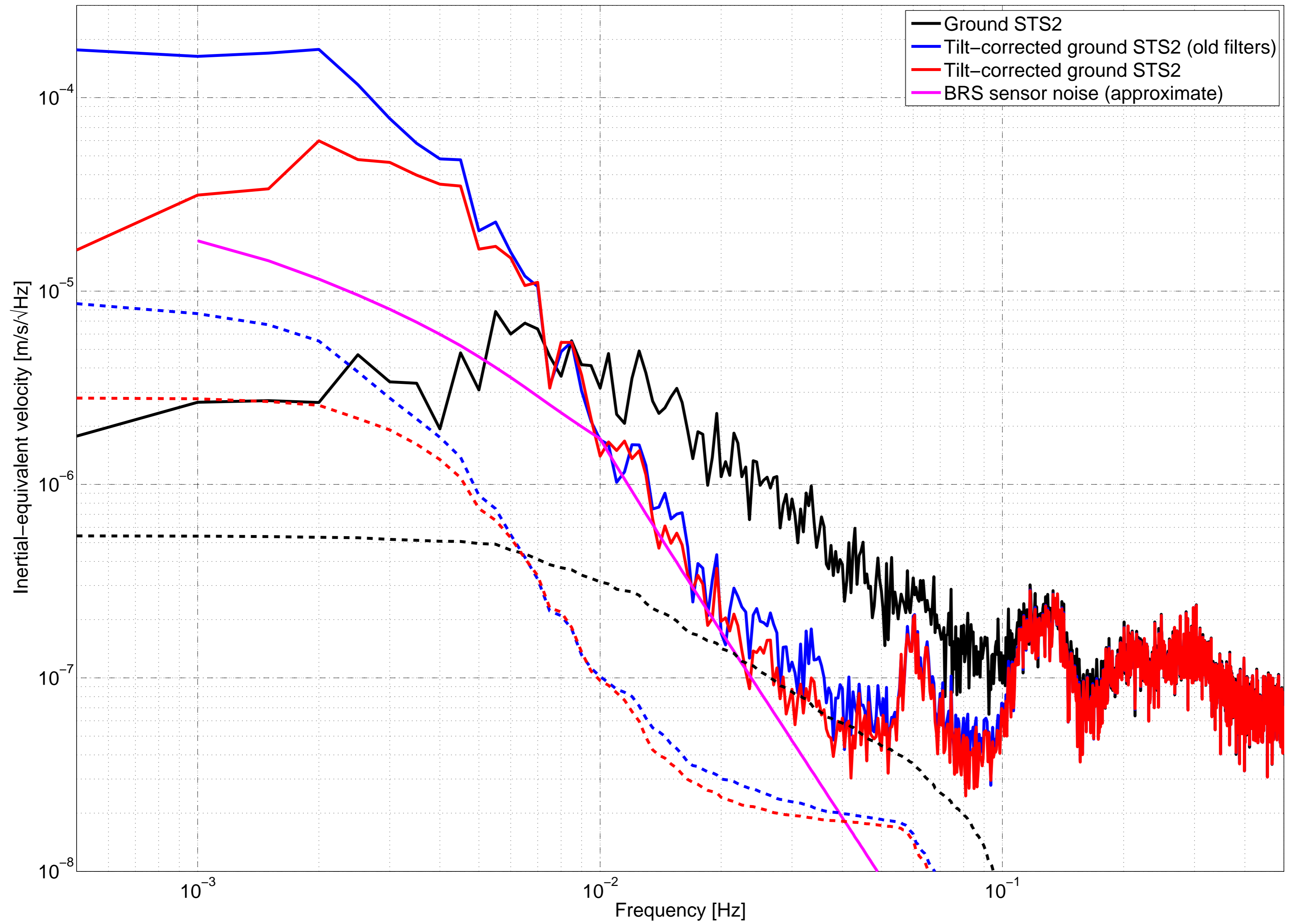
ETMX Tilt-correction filter tuning
