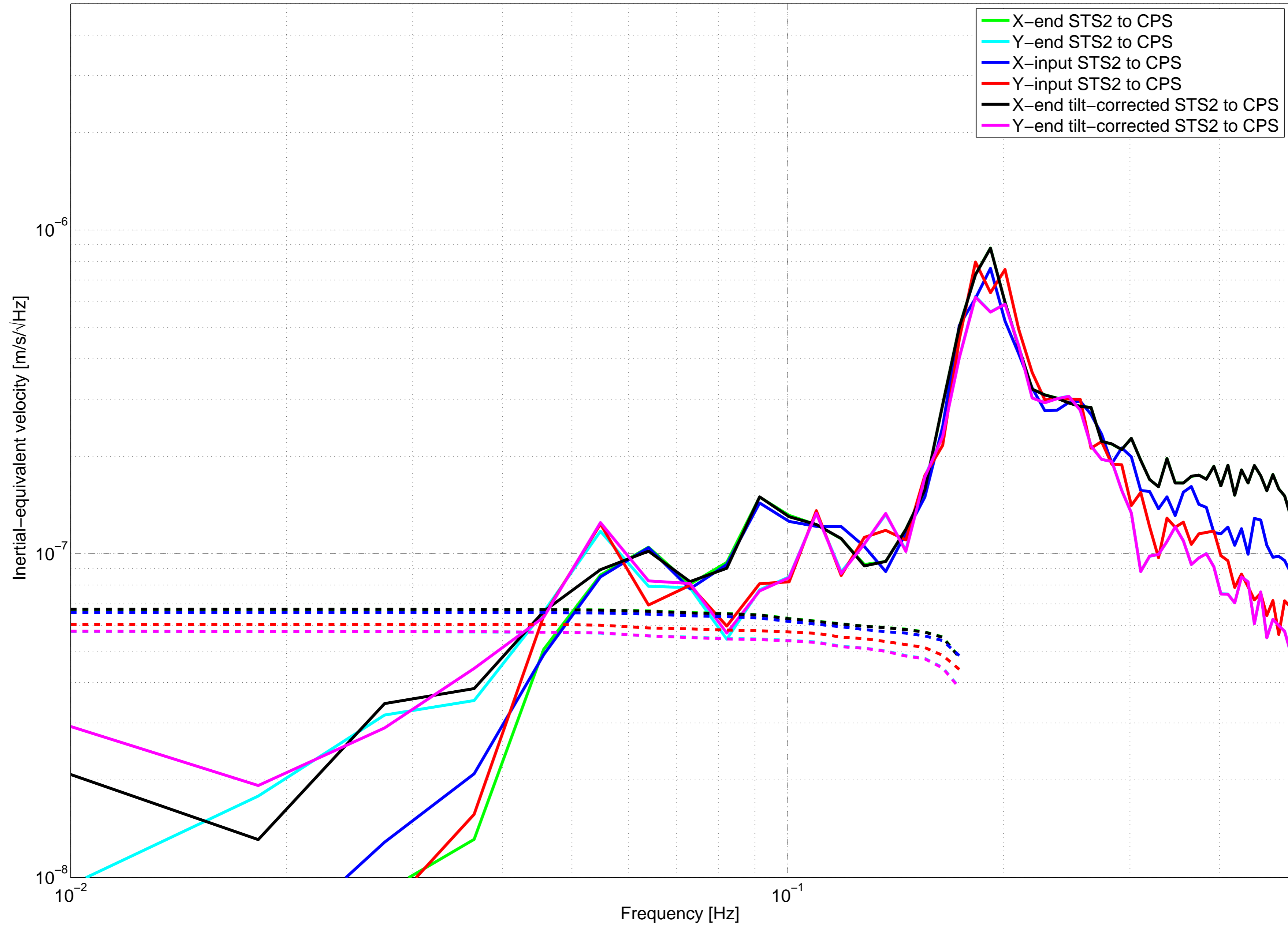
Ground-to-CPS Sensor correction
