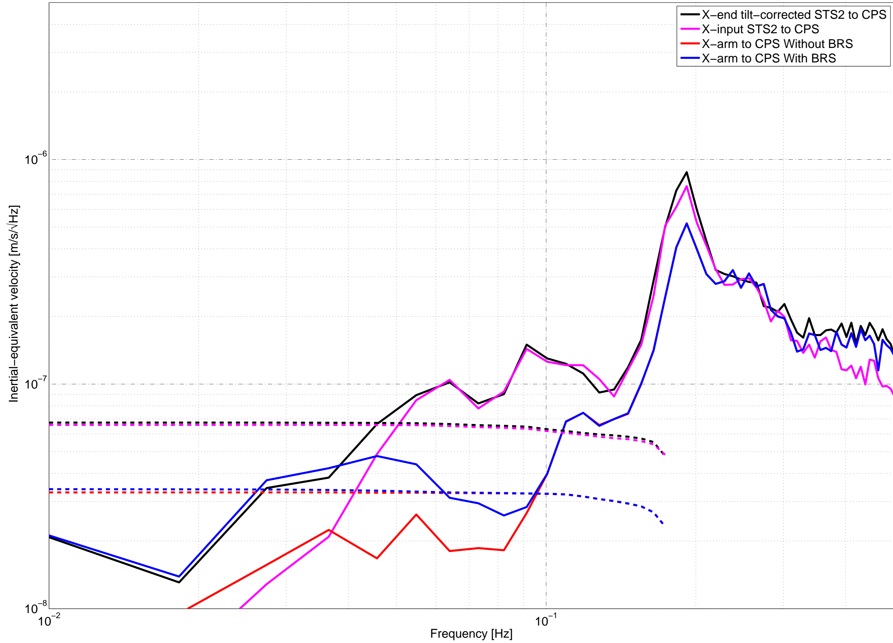
X-arm Ground-to-CPS Sensor correction
