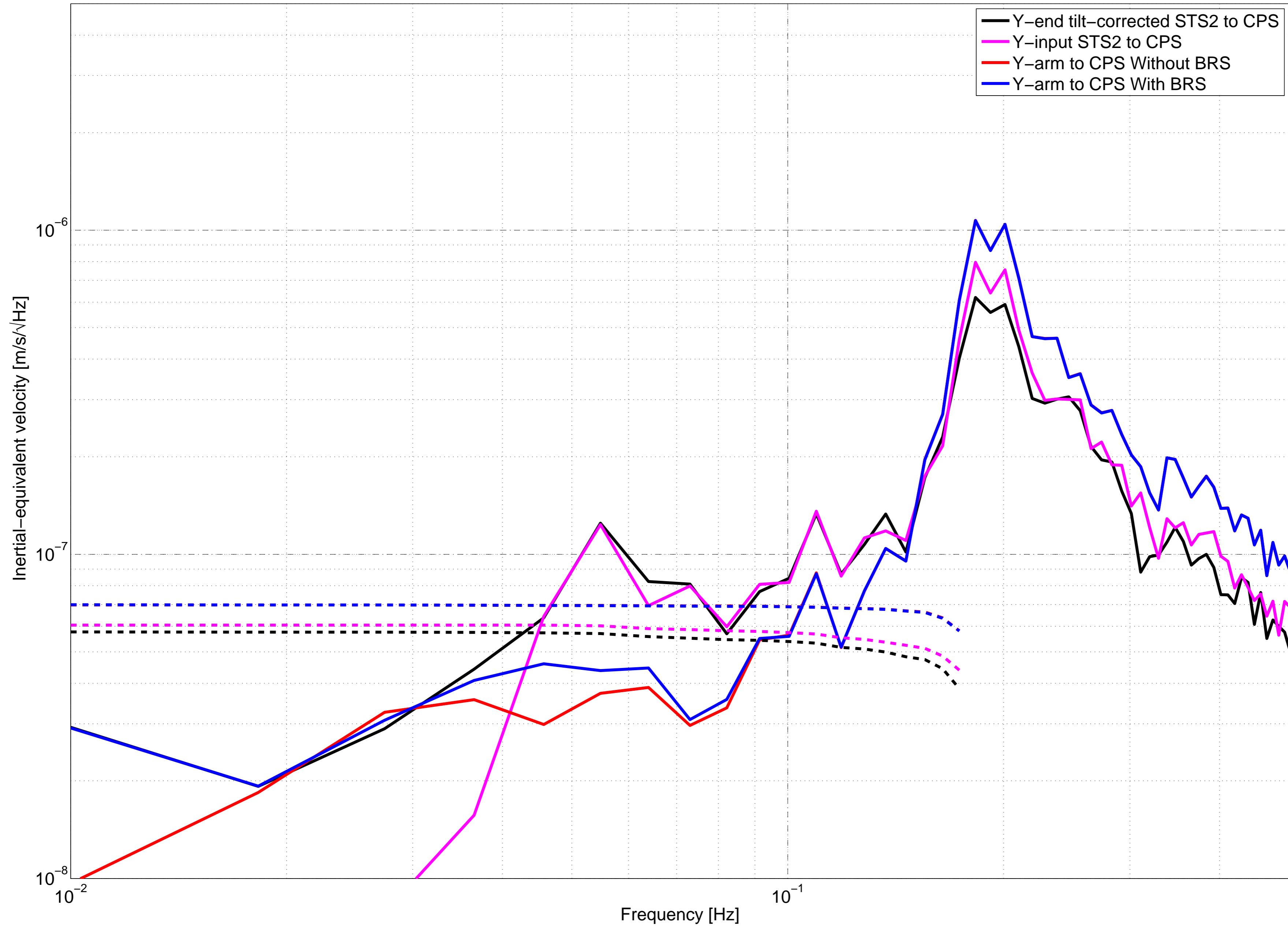
Y-arm Ground-to-CPS Sensor correction
