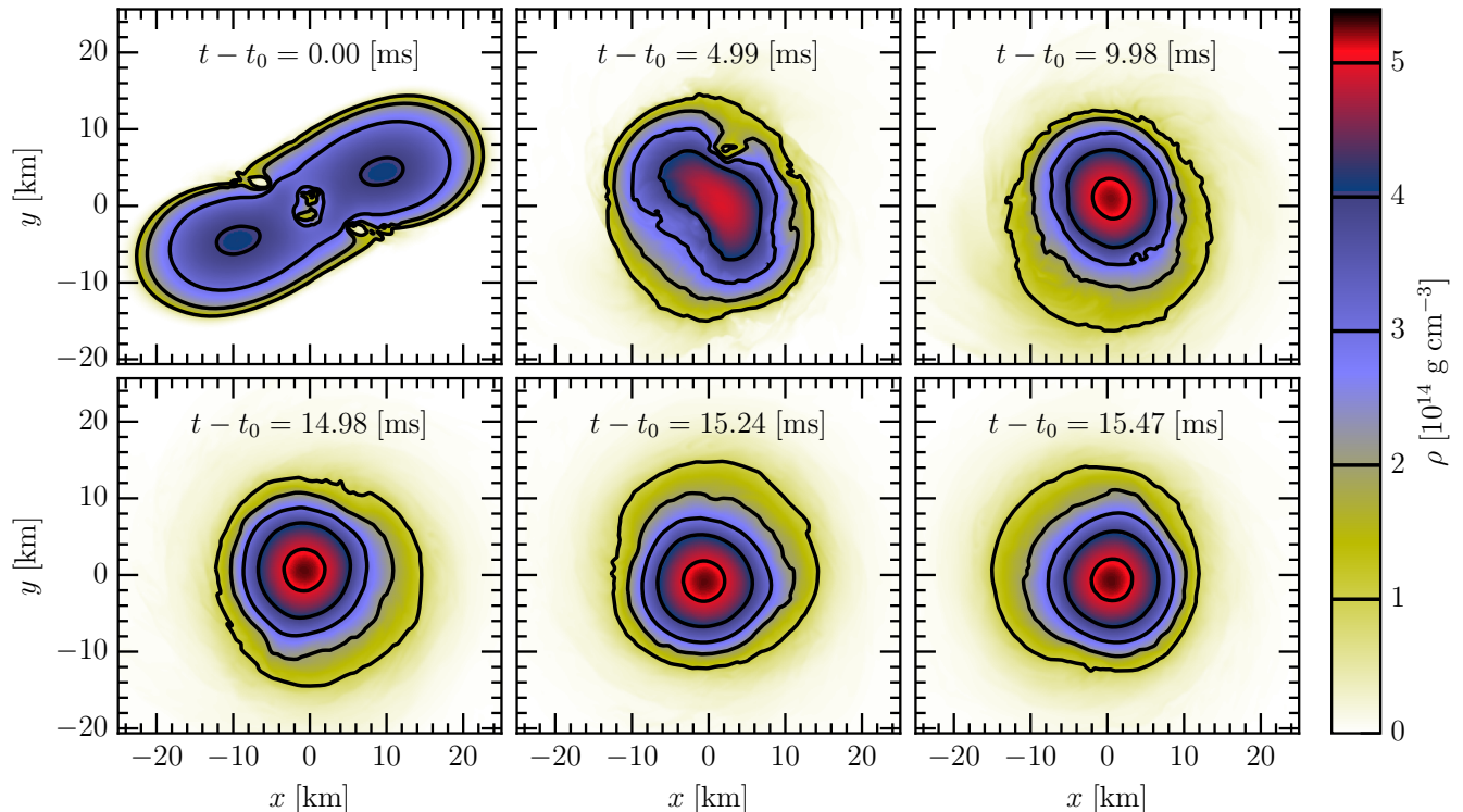
FIG. 1. Color coded rest-mass density in the orbital plane for our highest-resolution MS1b simulation at representative times after merger ( t_0 ). In the upper panels: merger and development of the m = 1 instability. In the bottom panel: roughly half a cycle of the saturated spiral mode. The 180^\circ rotational symmetry of the system is broken by hydrodynamic instabilities originating at the Kelvin-Helmholtz-unstable shear layer between the two stars shortly after merger. This causes the spiral mode to grow. Animations of the density in the orbital plane for both MS1b and SLy binaries are available as supplemental online material and at https://stellarcollapse.org/BNSm1 .
