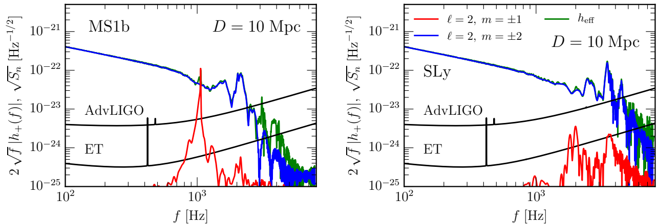
FIG. 3. Spectrum of the effective GW signal seen edge-on from a distance of 10 Mpc. We show the spectrum of the hybrid waveforms constructed from the highest resolution data and the noise curves of Advanced LIGO and ET. The \ell = 2 , m = 1 spectrum is mostly concentrated in a narrow maximum located at half of the frequency of the \ell = 2 , m = 2 peak.
