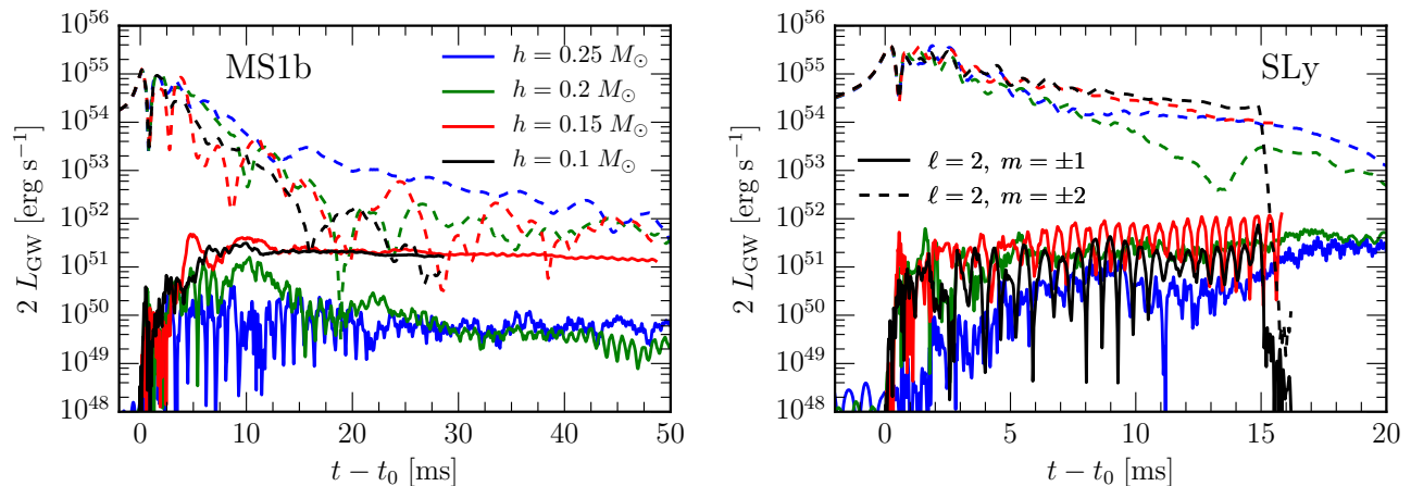
FIG. 2. GW luminosity of the \ell = 2 , m = 2 and \ell = 2 , m = 1 modes for all simulations as a function of time from merger ( t-t_0 ). The data are multiplied by a factor of two to account for the symmetry between positive and negative m . A contribution from the m = 1 mode is present in all simulations, especially at high resolution. GWs from the spiral mode are subdominant during most of the evolution, but show negligible damping.
