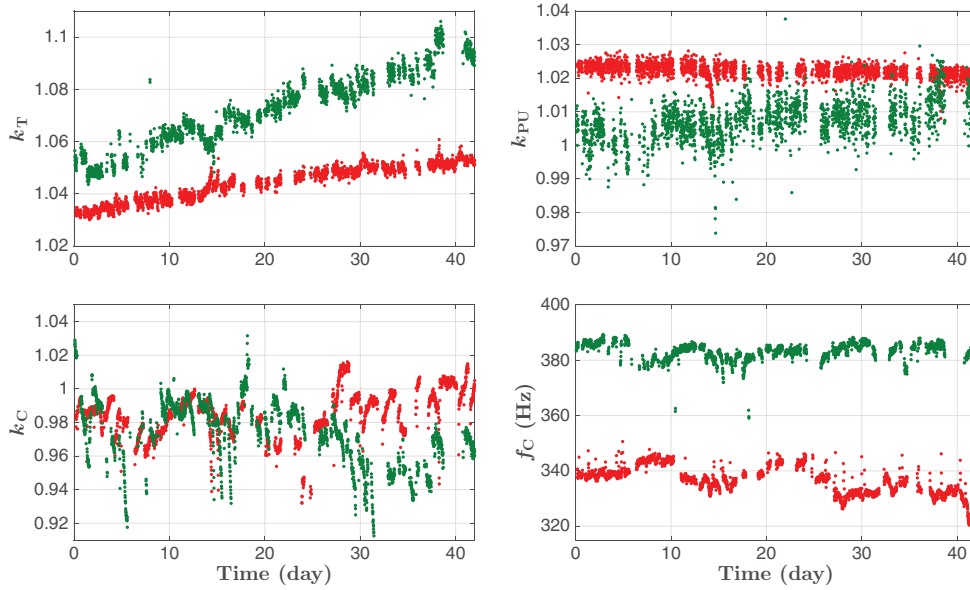
Figure 5. DARM time-dependent parameters calculated from calibration lines—LIGO Hanford ( red traces ) and LIGO Livingston ( green traces ). Nominal values of all three scalar factors \kappa_T , \kappa_{PU} and \kappa_C are 1, and the nominal value of the coupled cavity pole frequency, f_C , for LIGO Hanford is 341 Hz and for LIGO Livingston is 388 Hz [16].
