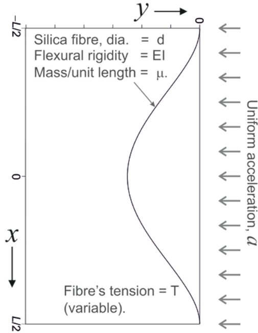
Figure A1: Deflection of a silica fibre, of length L , as it is loaded by a uniform (along the x -axis, and in the y -direction) transverse acceleration, a .
