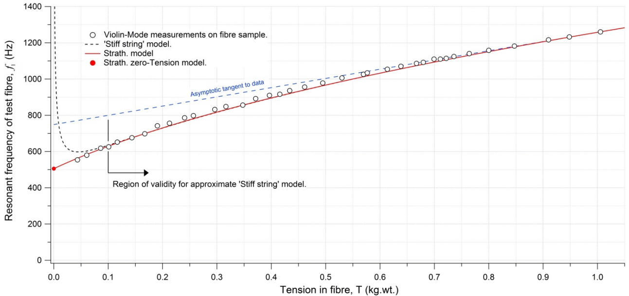
Figure 6. Resonant (Violin-Mode) frequency of the test fibre in air, measured at the AC (VM) output of the amplifier as a function of applied tension in the fibre sample, as the fibre was excited acoustically by a distant loudspeaker (open circles). The fibre's tension was increased steadily from 43.5 grammes wt. (0.427 N) to 1.0054 kg. wt. (9.863 N). Theoretical traces: please refer to the legend in the Figure (and to the text).
