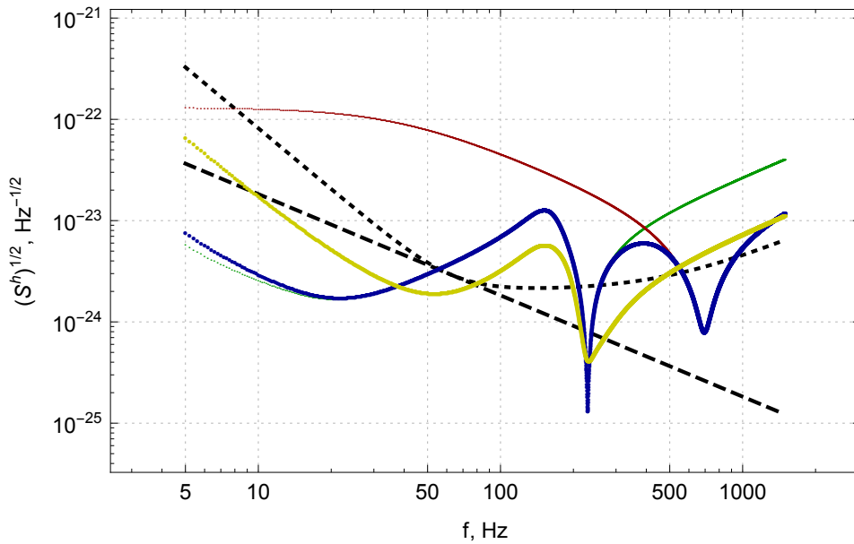
Figure 3: Dashed line: SQL, dotted line: baseline configuration. Yellow curve: simultaneous optimization. Blue: separate optimization. Green: negative optical inertia pair for separate optimization from 5 to 100 Hz. Red: antisymmetric pair for separate, optimized with presence of negative pair. All parameters are presented in Table 2.
