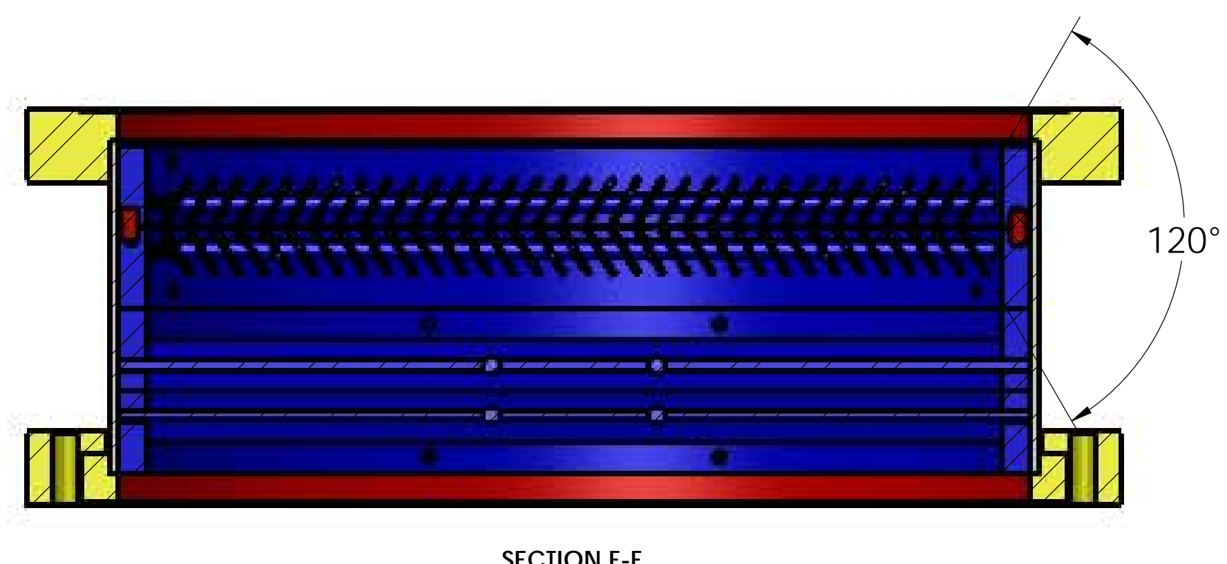
SECTION F-F
