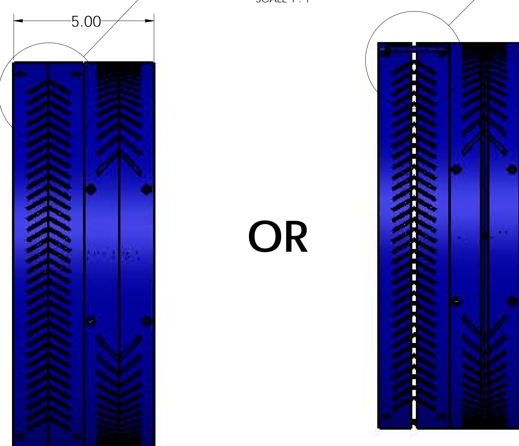
SIDE VIEW (16.5" CF, FULL NIPPLE, NOT SHOWN REFER TO SHEET 1 FOR DETAILS)
