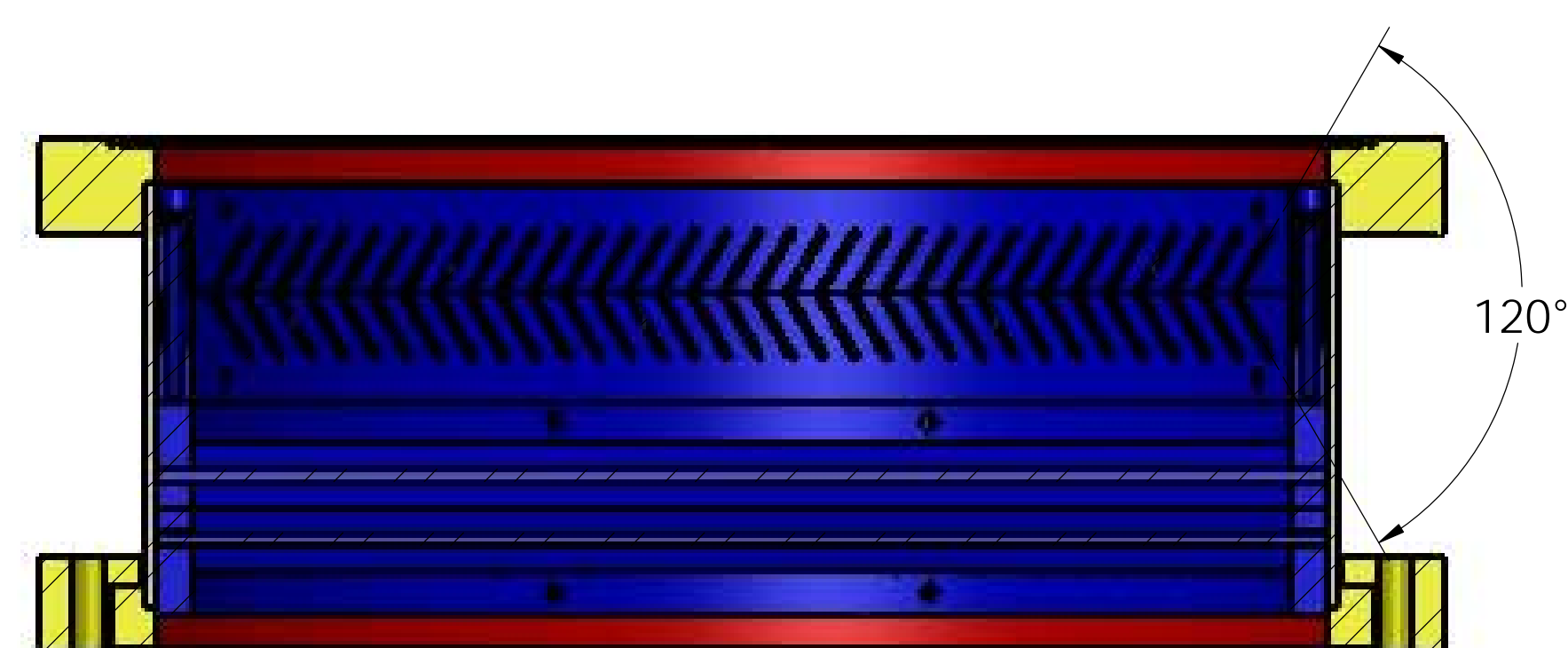
SECTION G-G
