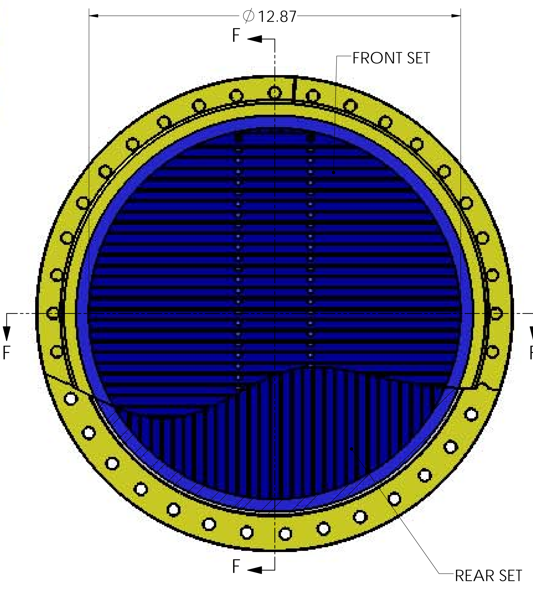
FRONT VIEW
