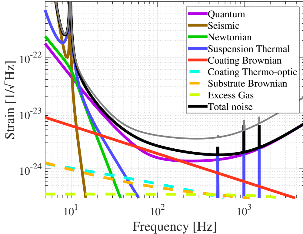
Figure 3: Strain sensitivity of A+ (BNS range of 320 Mpc). The results of improved quantum noise (16m filter cavity and 6 dB of measured squeezing at high frequency) and modestly improved thermal noise (factor of two lower loss high index material), are shown. The Advanced LIGO sensitivity curve is shown in gray for reference.
