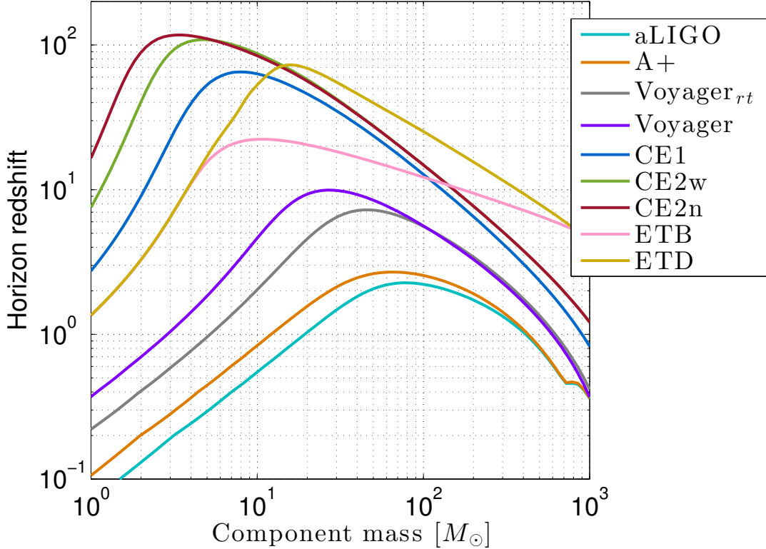
Figure 10: Astrophysical reach of various interferometers for equal-mass compact binary inspiral systems. The maximum observable distance is shown as a function of the intrinsic mass of one of the components. Clearly, at redshifts larger than z \simeq 10 there will be few sources, and yet a horizon of z > 20 for a given mass should be taken to indicate that essentially all compact binary coalescence in the universe will be observed, many with a high signal to noise ratio. Similar curves for the Einstein Telescope are shown for comparison (see figures 11 and 12). A Hubble constant of 67.9 km/s/Mpc and a \Lambda CDM model of expansion was used.
