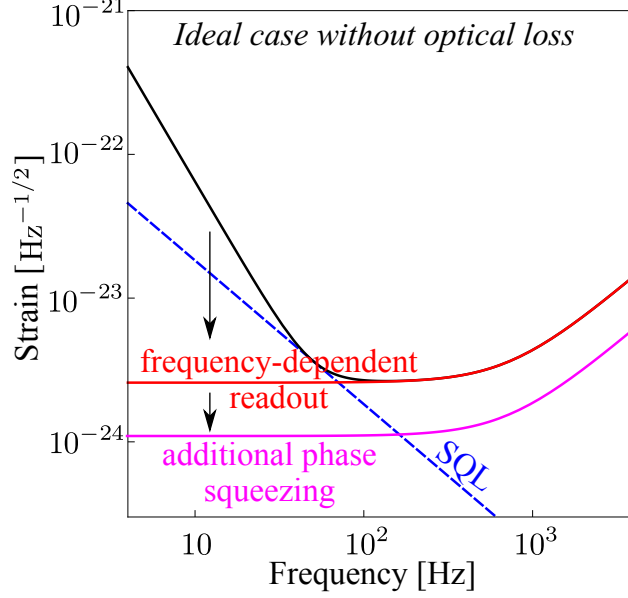
Figure 20: The noise spectrum for the frequency-dependent readout scheme.
