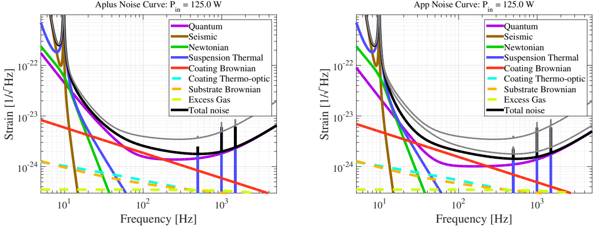
Figure 8: Strain sensitivity of “nominal” A+ (left, 320 Mpc) and “optimistic” A+ (right, 460 Mpc). The left curve uses a 16 m filter cavity and 6 dB of measured squeezing at high frequency, along with a factor of 2 lower loss in the coating high index layer relative to aLIGO (i.e., a loss angle of 10^{-4} ). The right curve uses a 4 km filter cavity and 8 dB of measured squeezing at high frequency, with a factor of 4 lower loss in the coating high index layer relative to aLIGO (i.e., a loss angle of 5 \times 10^{-5} ). The Advanced LIGO sensitivity curve is shown in gray for reference in both plots, while the “nominal” A+ curve is also shown on the “optimistic” plot.
