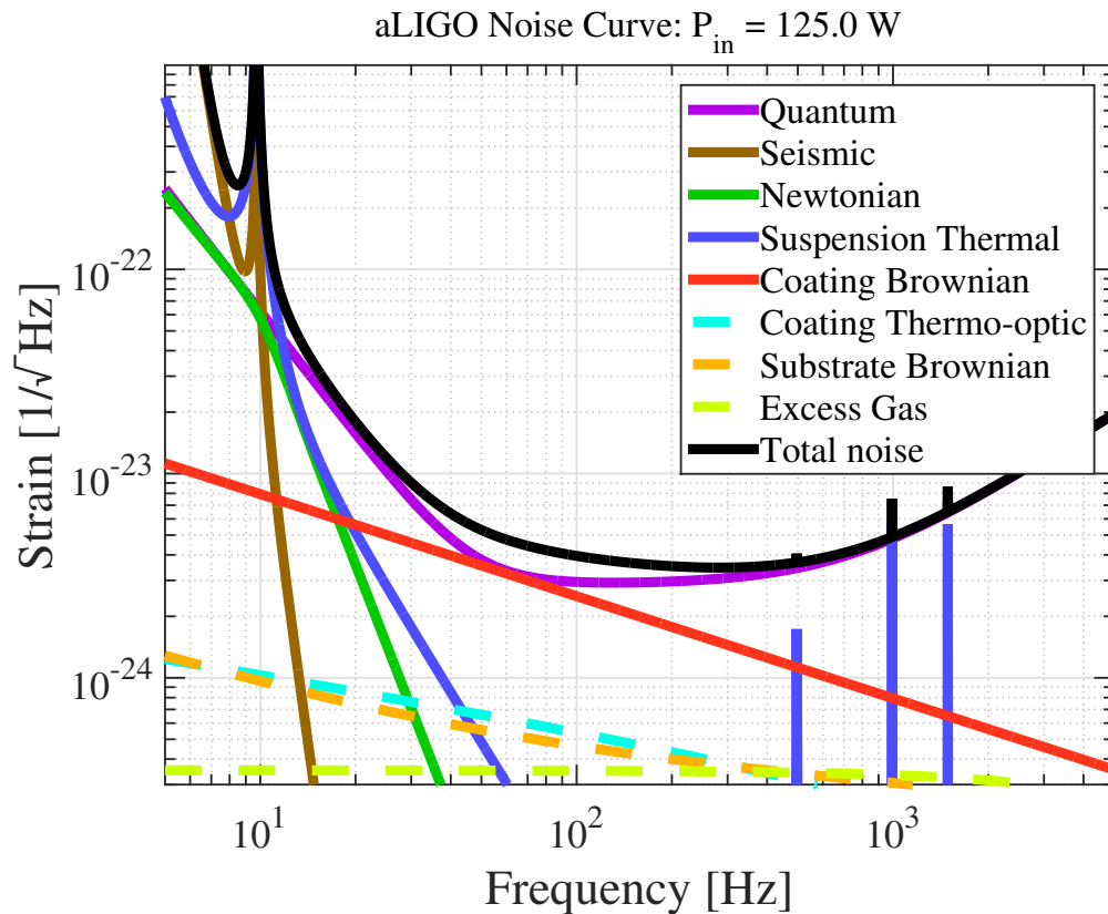
Figure 1: Baseline aLIGO Noise Budget (GWINC v2.1). 125 W input power; broadband RSE tuning. Experience to date with the aLIGO instruments has not uncovered any barrier to achieving performance consistent with these curves. Updated calculations give a binary neutron star (BNS) range of 210 Mpc.
