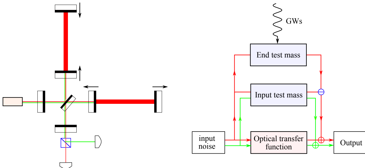
Figure 26: Diagram of the local-readout topology (left) and the resulting feedback loops (right).
