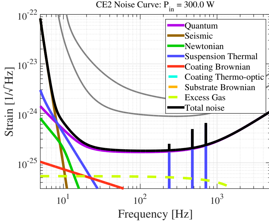
Figure 5: Conceptual noise budget for CE2 (BNS range 64 Gpc, or z of 13). These curves are based on a 40 km facility which utilizes Voyager technology. The A+ and Voyager sensitivities are shown in gray for reference.
