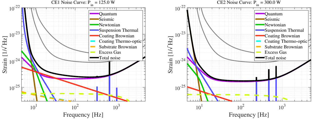
Figure 11: Strain sensitivity of room temperature Cosmic Explorer (CE1, left, with a BNS range of 19 Gpc or z = 4.5 ) and cryogenic Cosmic Explorer (CE2, right, 70 Gpc or z = 14 ). CE1, based on A+, makes the very conservative assumption that little improvement is made in coating technology in the next 20 years, and that cryogenic silicon operation turns out not to be a viable technology. That is, CE1 is based on demonstrated technology and thus serves as a lower bound to the performance of a new facility. CE2, based on Voyager technology, represents a more realistic scenario in which significant progress is made in coating thermal noise and power handling technology. The A+ and Voyager sensitivity curves are shown in gray for reference.
