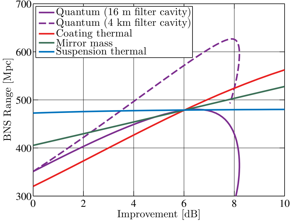
Figure 7: BNS range as a function of individual improvements. For the quantum noise the horizontal axis depicts the measured squeezing at high frequency, for the mirror mass the increase in mass, for the coating thermal noise and for the suspension thermal noise it shows the reduction factor. For each trace the remaining parameters are held fixed at their higher sensitivity. The four continuous curves intersect at the 6 dB point, where they all yield a factor of two improvement. For this configuration a longer filter cavity is significantly more effective (dashed curve).
