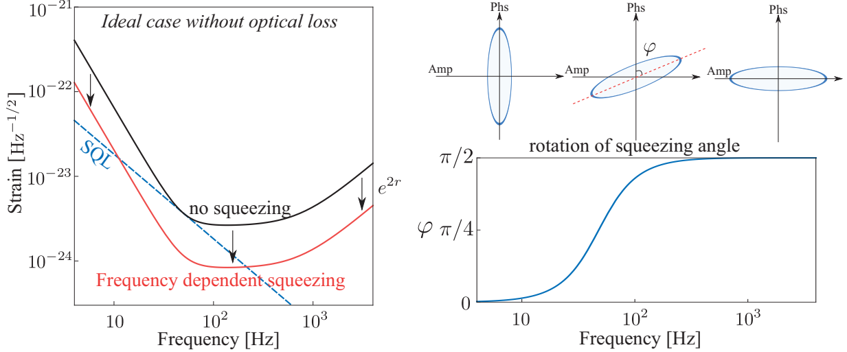
Figure 17: Noise spectrum for frequency-dependent squeezing (left) and rotation of the squeezing angle (right).
