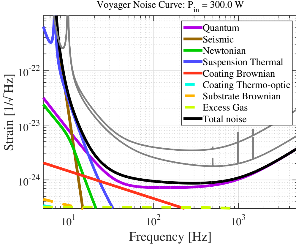
Figure 4: Conceptual noise budget for Voyager (BNS range of 1.3 Gpc). The technology assumed for these curves includes cryogenic operation at 123K, silicon optics, AlGaAs coatings, and 1550nm laser wavelength, and 8dB of frequency dependent squeezing. The Advanced LIGO and A+ sensitivities are shown in gray for reference.
