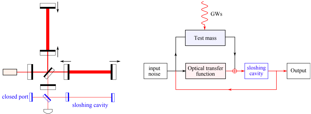
Figure 23: Schematics showing the speed-meter configuration (left) and its flow chart (right).
