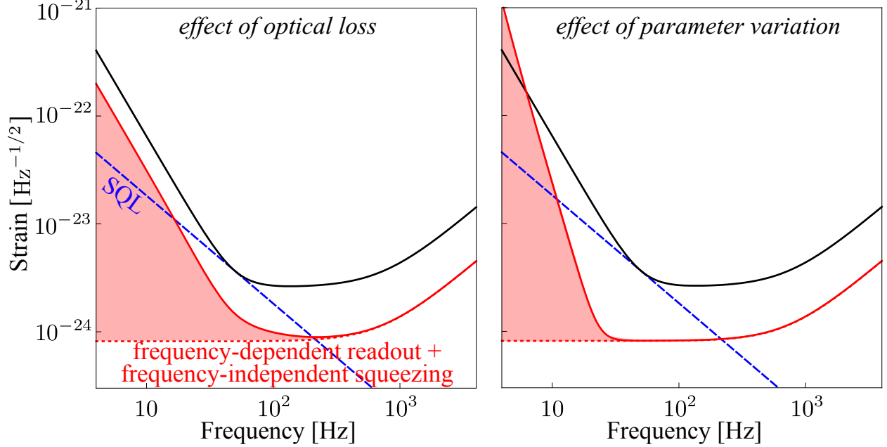
Figure 21: The effect of optical loss (left) and parameter variation of the filter cavity (right) for frequency-dependent readout (output filtering). Similar to Fig. 18, we have used a total optical loss of 20%. In contrast, the parameter variation is chosen to be only 10^{-4} in order to produce reasonable sensitivity, as it is much more sensitive than input filtering.
