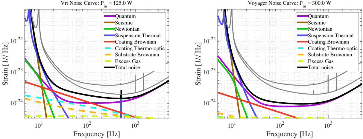
Figure 9: Strain sensitivity of room temperature Voyager (left, 700 Mpc) and cryogenic Voyager (right, 1.3 Gpc). These two versions of Voyager assume the same coating (AlGaAs) and squeezing technology, but differ in their operating temperature (295 K vs. 123 K), substrate material (Silica vs. Silicon) and wavelength (1064 nm vs. 1550 nm). The advantages of cryogenic operation are seen in the reduced coating thermal noise (by \sqrt{T} ) and the high operating power which results from the high thermal conductivity of silicon. The Advanced LIGO and A+ sensitivity curves are show in gray for reference.
