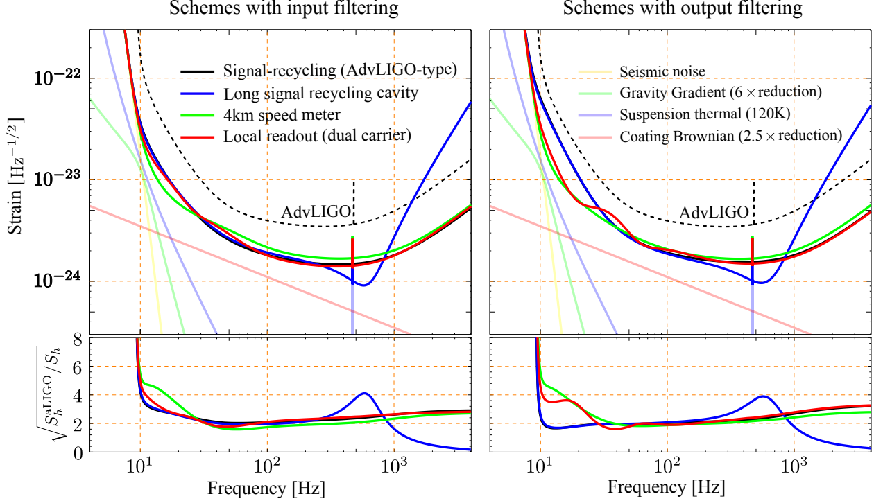
Figure 27: The optimized total noise spectrum for different schemes assuming a moderate improvement of the thermal noise compared with aLIGO baseline design. The lower panels show the linear strain sensitivity improvement over aLIGO.
