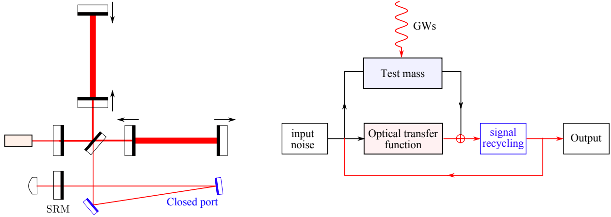
Figure 22: Schematics showing the long signal-recycling cavity scheme (left) and its associated flow chart (right). The signal-recycling mirror coherently reflects back the signal, forming a feedback loop as indicated in the flow chart.
