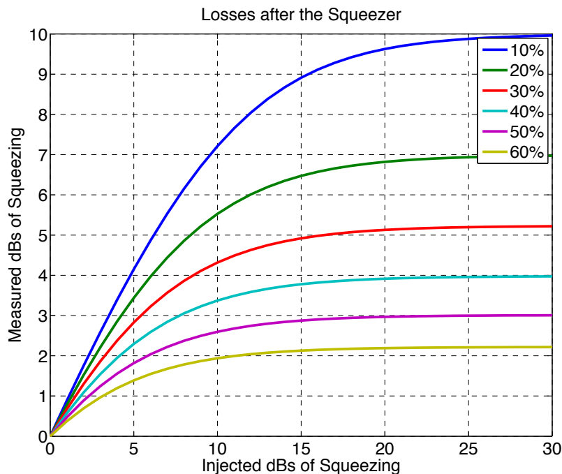
Figure 32: Measured squeezing as function of the injected squeezing for different levels of losses in the squeezed path.
