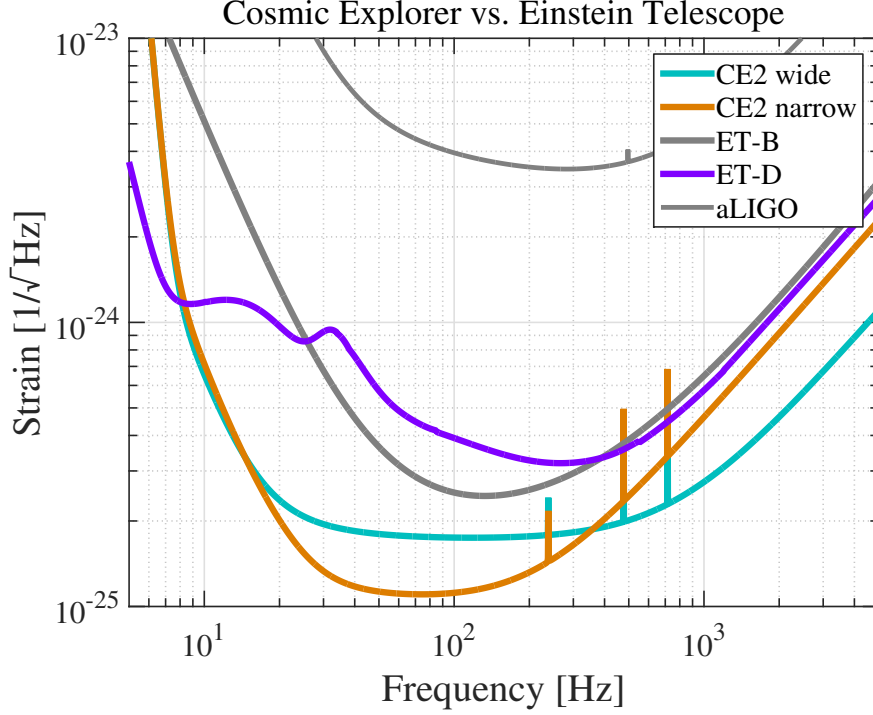
Figure 12: Strain sensitivity of CE2, ET-B and ET-D. CE2 is shown in the nominal wide-band configuration, as well as a narrow-band (reduced RSE) configuration which has a more similar shape to ET-B. Narrow-band CE2 sacrifices high frequency performance for improved inspiral range; its BNS range is 138 Gpc, or z = 26 . The choice of interferometer bandwidth has few implications for interferometer design, and so can be made after, and informed by, many years of detections.
