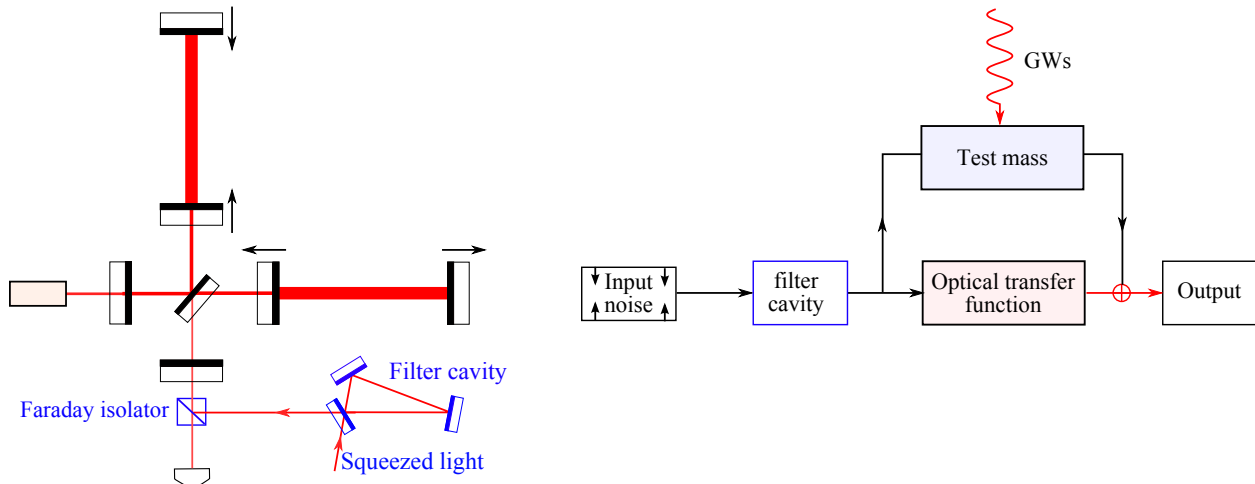
Figure 16: Schematics showing the frequency-dependent squeezing scheme (left) and its associated flow chart (right).
