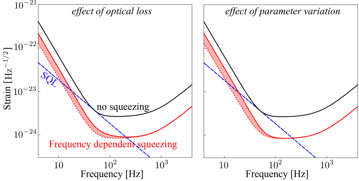
Figure 18: The effect of optical loss (left) and the parameter variation of the filter cavity (right) for input filtering. The shaded regions illustrate the degradation in sensitivity. Here we have assumed the total optical loss of 20% (round-trip loss multiplied by the number of bounces inside the cavity) and parameter variations of 10%.
