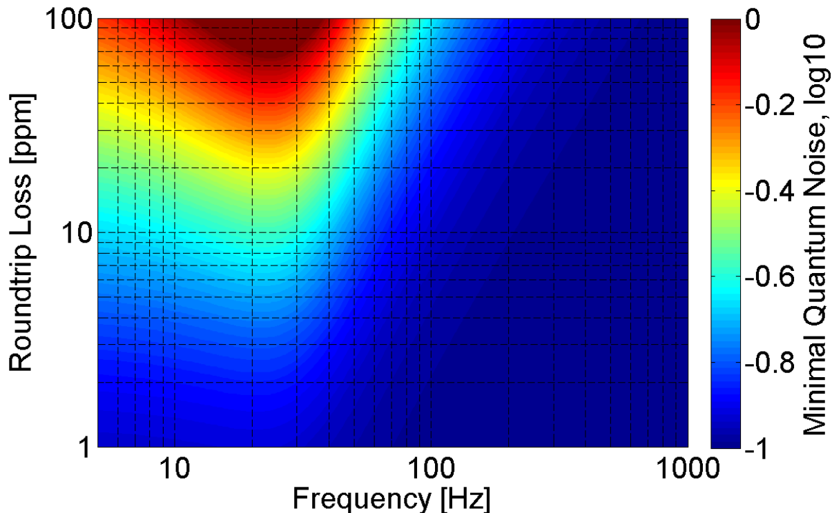
Figure 15: Degradation of 10 dB external squeezing reflected from a 300 m filter cavity as function of round-trip loss (in addition to input transmission) and frequency.
