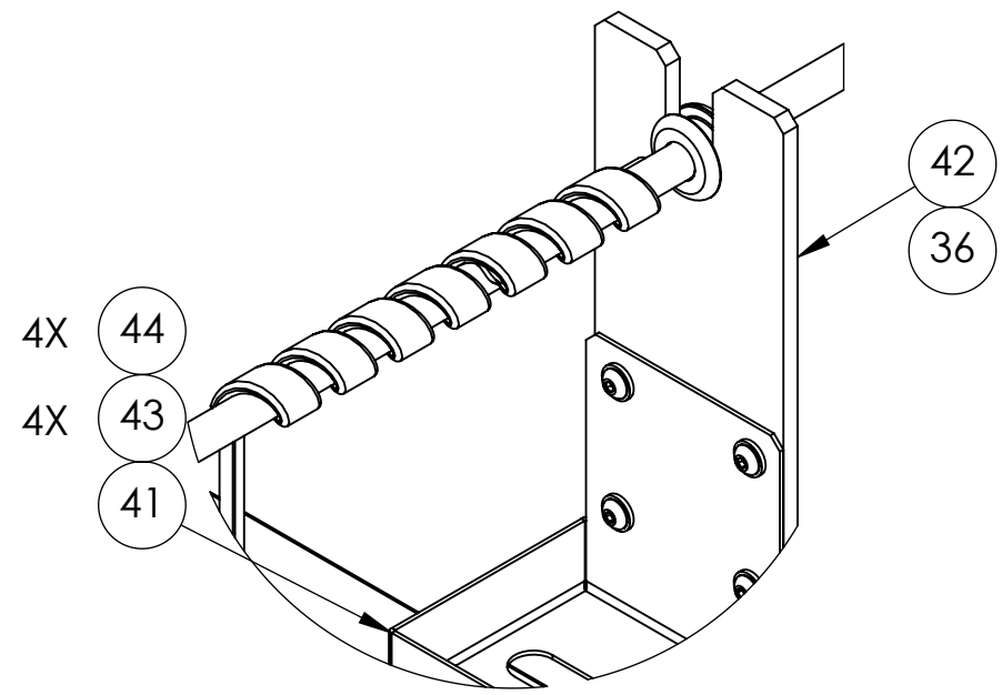
DETAIL D SCALE 1 : 2
