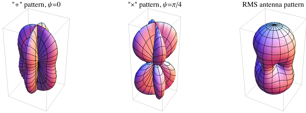
Figure 2.1 The directional dependence of the +, ×, and root mean square (RMS) antenna patterns of a LIGO-style GW detector. The detector is at the center of the light box, with its two arms parallel to the horizontal edges.
