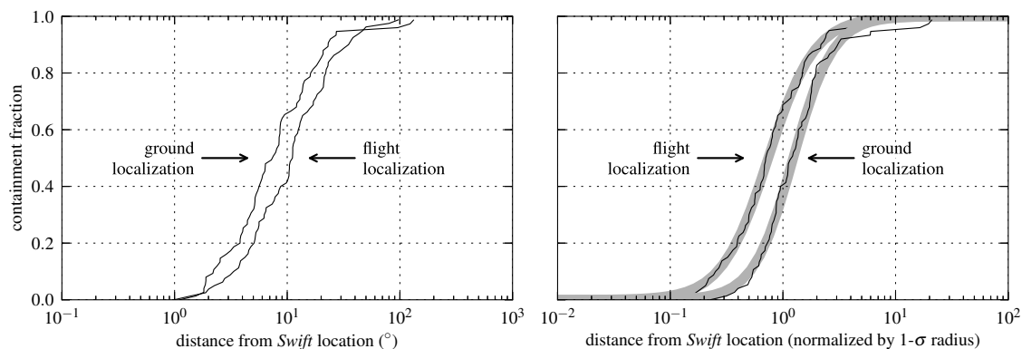
Figure 6.2 Localization accuracy of Fermi GBM positions, generated by searching for coincidences with GRBs detected by the Swift satellite. The left panel shows the fraction of bursts contained within a given distance from the Swift position, both for in-flight and refined ground-based localizations. Ground-based localizations are on average about half as far from the true GRB positions as the in-flight localizations. The right panel shows a cumulative histogram of the Fermi – Swift distance, normalized by each trigger’s nominal 1\sigma radius (either ground-based or in-flight). Although the ground-based localizations are more accurate, the nominal ground-based error radii must be interpreted as describing a different confidence level than the in-flight error radius. The thick gray lines are fits to the logistic-like function in Equation 6.1.
