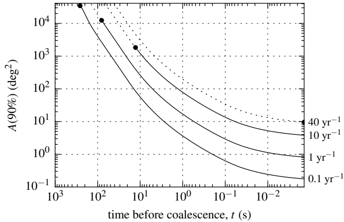
Figure 3.2 Area of the 90% confidence region as a function of time before coalescence for sources with anticipated detectability rates of 40, 10, 1, and 0.1 \text{ yr}^{-1} . The heavy dot indicates the time at which the accumulated SNR exceeds a single-detector threshold of 8.
