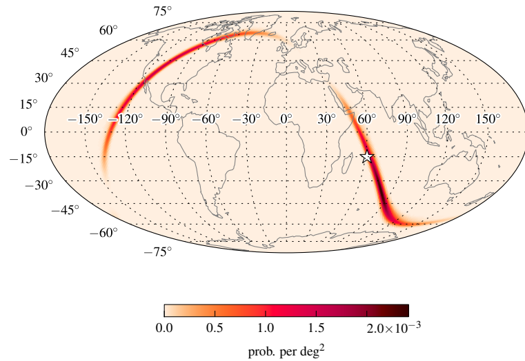
(a) BAYESTAR
