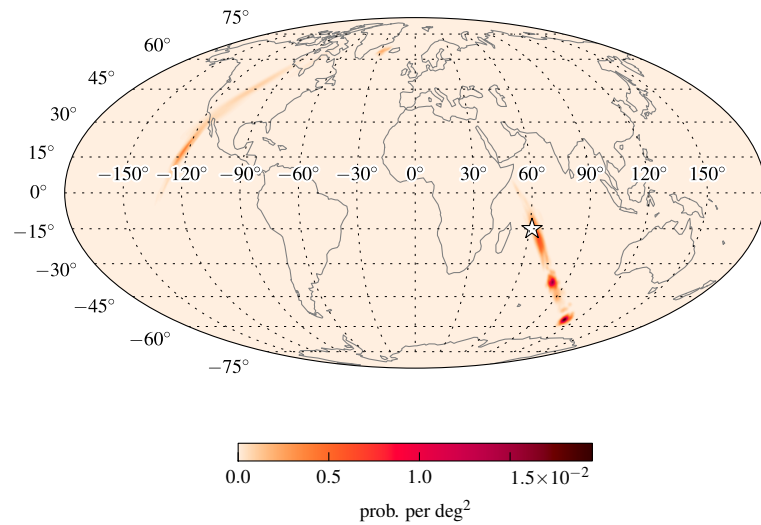
(b) LALINFERENCE_MCMC
