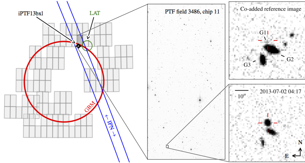
Figure 1.7 P48 imaging of GRB 130702A and discovery of iPTF13bxi. The left panel illustrates the \gamma -ray localizations (red circle: 1\sigma GBM; green circle: Large Area Telescope (LAT); blue lines: 3\sigma InterPlanetary Network (IPN)) and the 10 P48 reference fields that were imaged (light gray rectangles). For each P48 pointing, the locations of the 11 CCD chips are indicated with smaller rectangles (one CCD in the camera is not currently operable). The small black diamond is the location of iPTF13bxi. The right panels show P48 images of the location of iPTF13bxi, both prior to (top) and immediately following (bottom) discovery. Reproduced from Singer et al. (2013).
