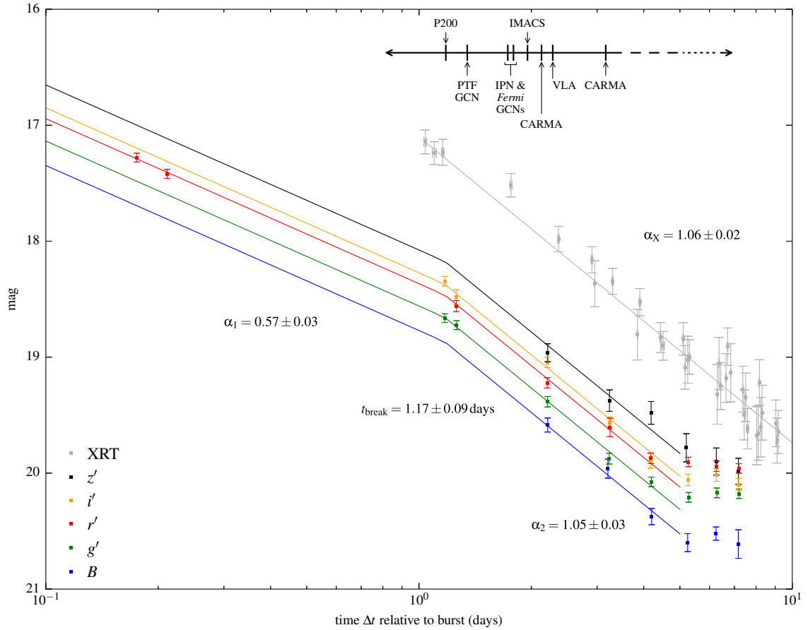
Figure 6.3 P48, P60, and X-ray Telescope (XRT) light curves of iPTF13btl. The broken power-law fit is shown up to \Delta t = 5 days. The XRT observations, re-binned to improve presentation, are shown in gray as m(\text{AB}) - 6.5 at 1 keV. A timeline in the top right puts the P48 and P60 observations in the context of the XRT follow-up, PTF's discovery GCN (Singer et al., 2013), the announcement of the LAT (Cheung et al., 2013) and IPN (Hurley et al., 2013) localizations, and the radio observations.
