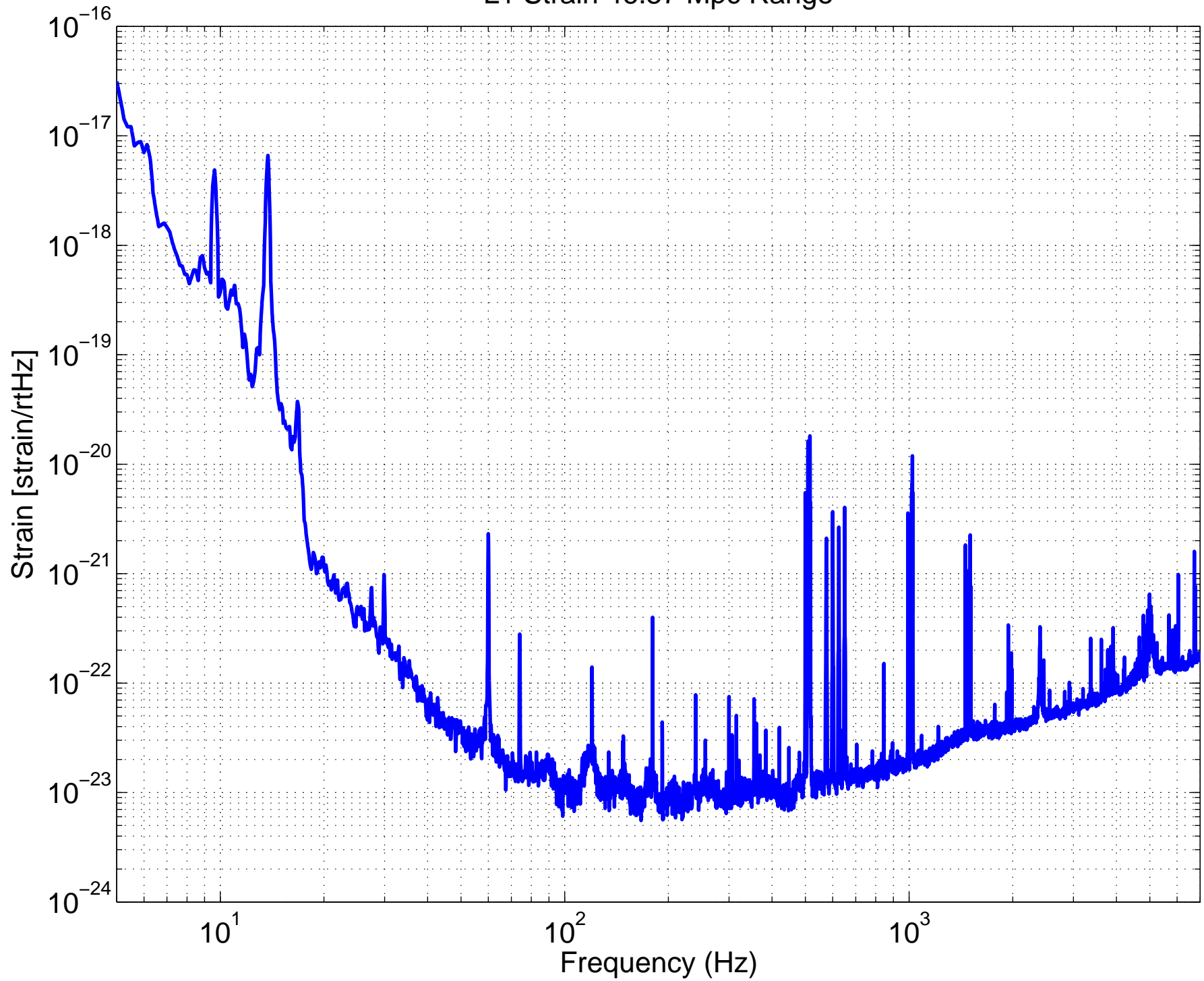
L1 Strain 46.57 Mpc Range
