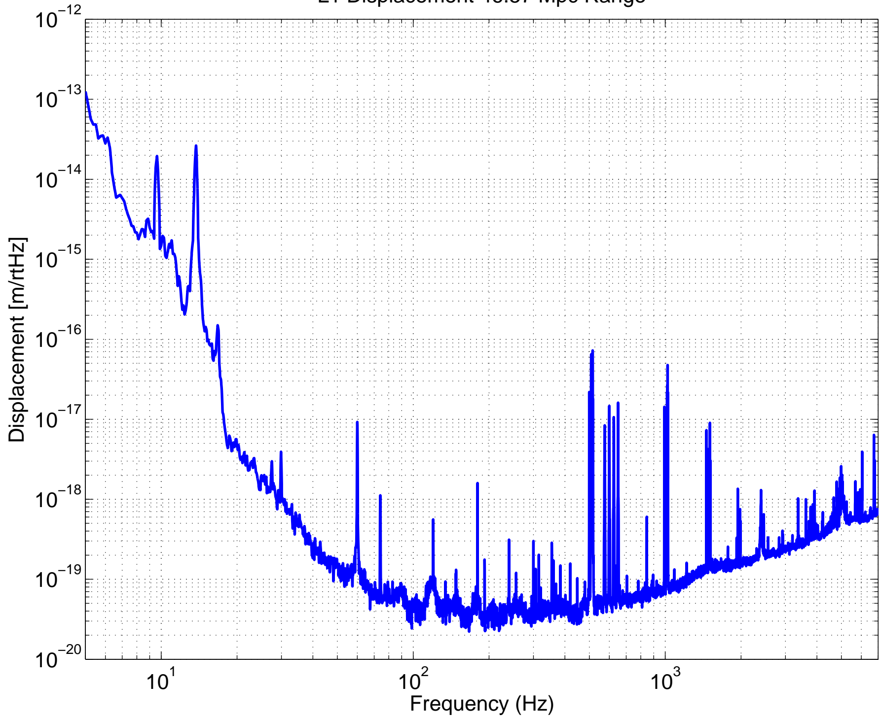
L1 Displacement 46.57 Mpc Range
