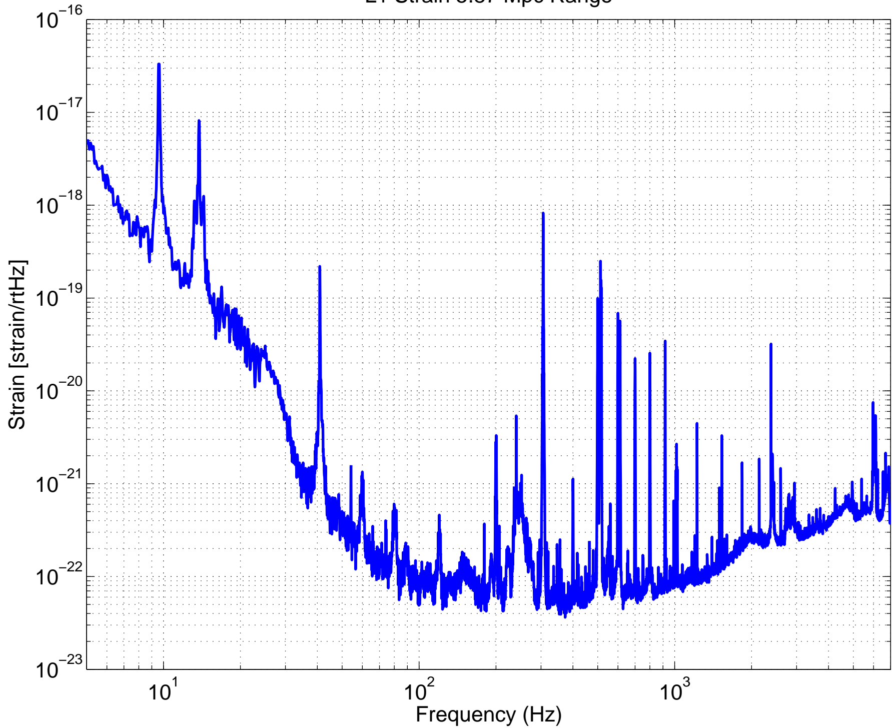
L1 Strain 5.87 Mpc Range
