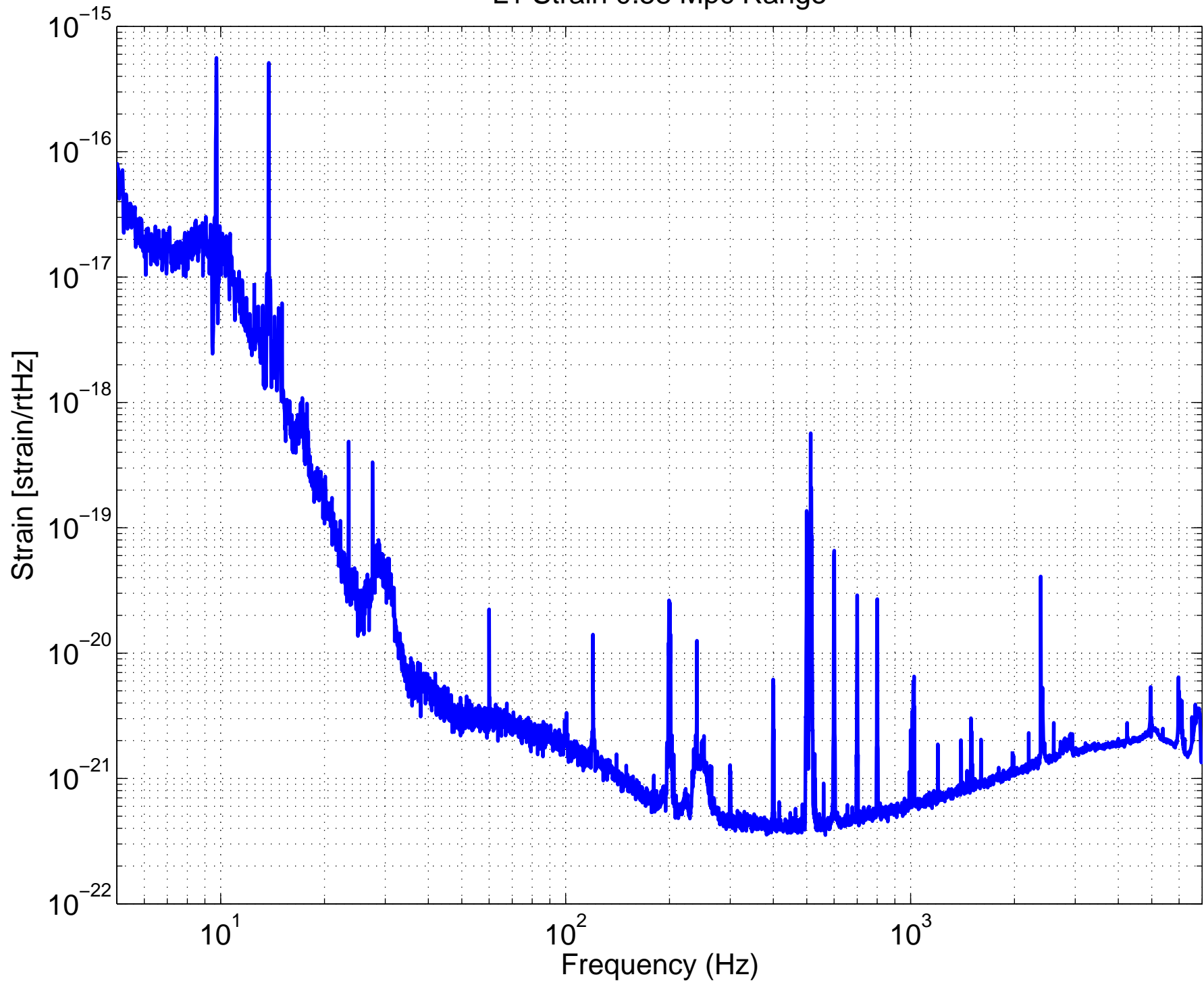
L1 Strain 0.58 Mpc Range
