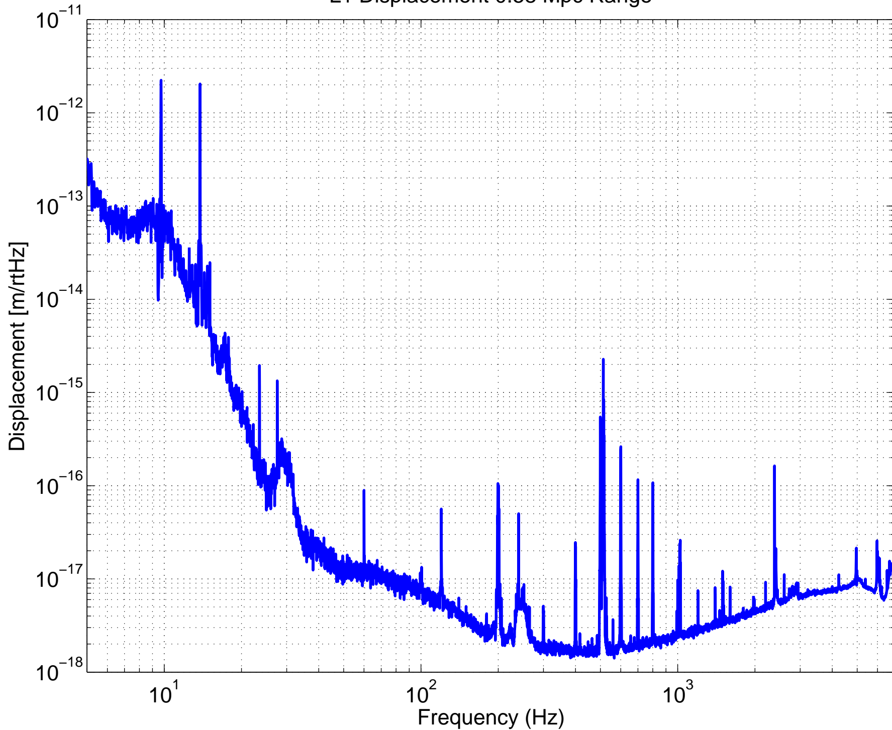
L1 Displacement 0.58 Mpc Range
