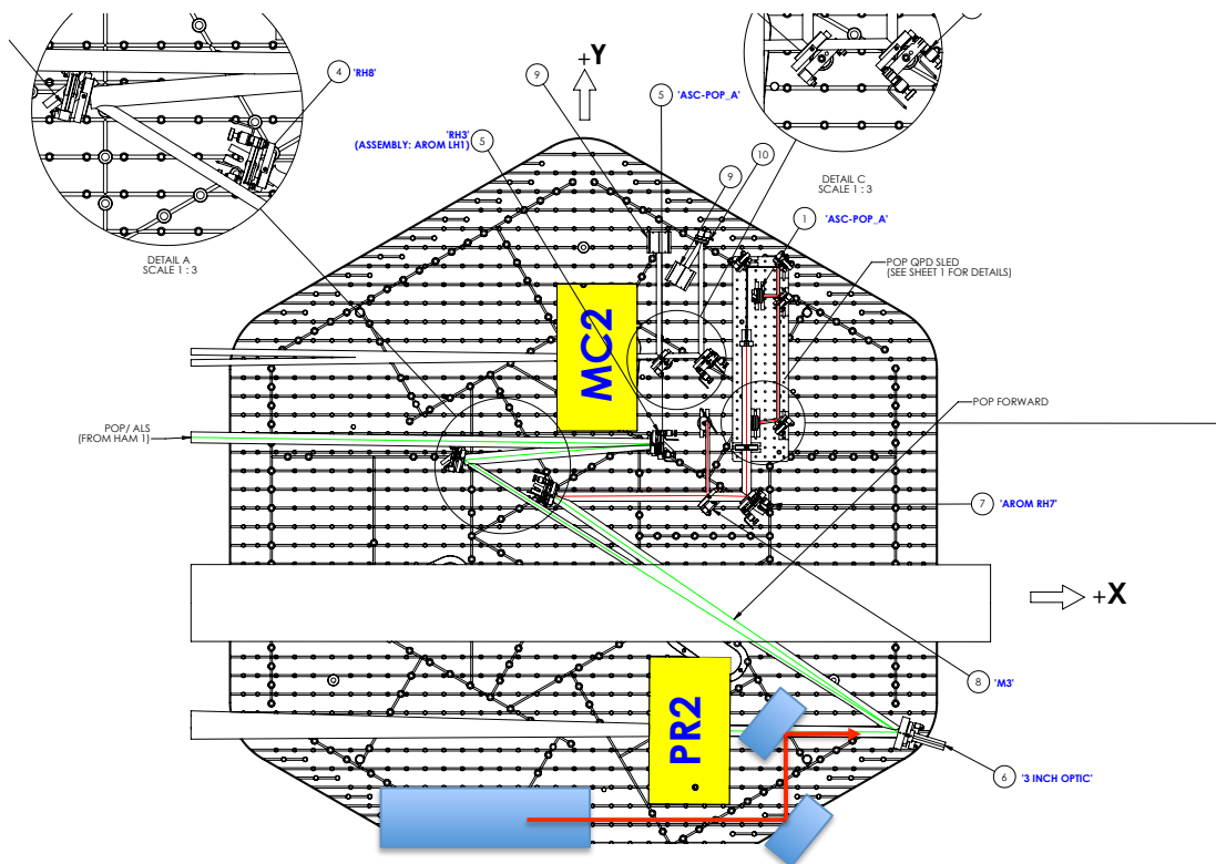
Figure 4: Simplified drawing of the OPTION 2 alignment setup. The auxiliary IR laser source is mounted on a class B breadboard inside the chamber. Both HAM3 doors should be off to have access to the laser source and to the BS.
