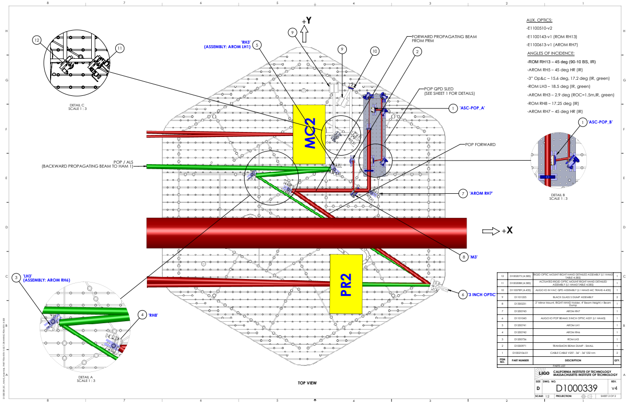
Figure 1: HAM3 ISC layout (D1000339). The installation procedure in this note concerns the POP forward propagating beam (red beam in the drawing).
