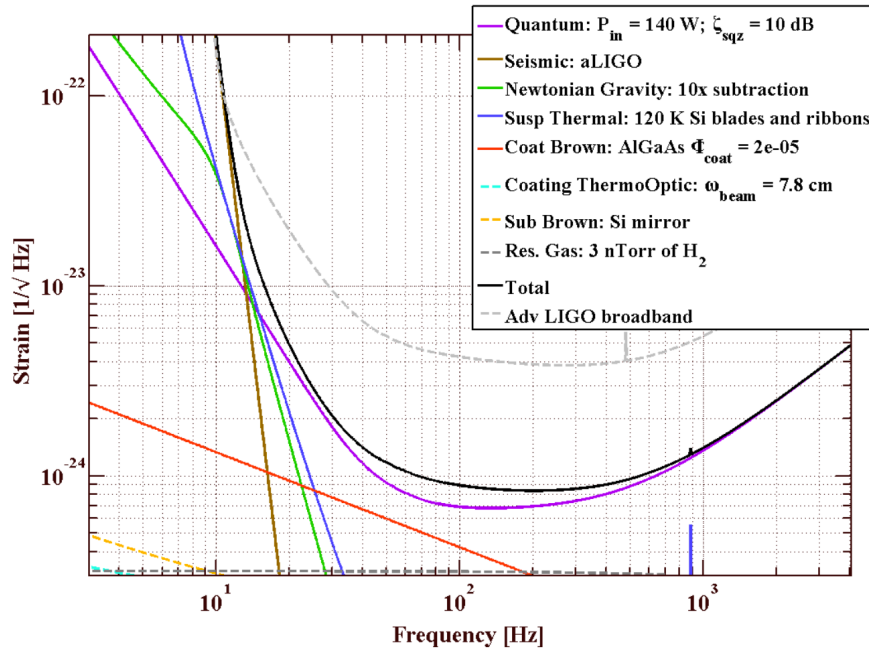
Figure 5: Conceptual noise budget for Voyager.
