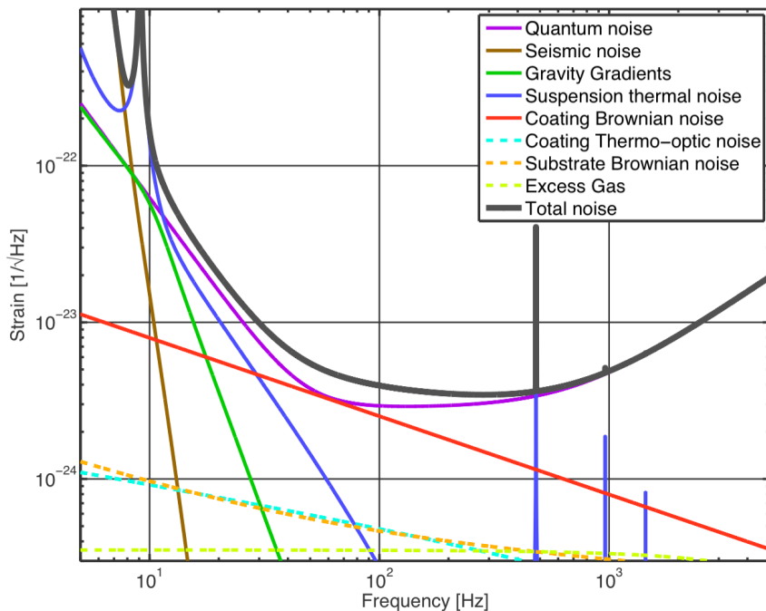
Figure 1: Baseline aLIGO Noise Budget (GWINC v2.0). 125 W input power; broadband RSE tuning. Experience to date with the aLIGO instruments has not uncovered any barrier to achieving performance consistent with these curves.
