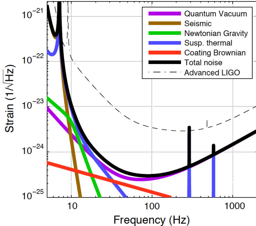
Figure 6: Projected sensitivity of a 40 km long interferometer based on Advanced LIGO. The signal extraction mirror transmission is reduced to 10%, the length of the final suspension stage is extended to 1 meter, and squeezing is injected through a 1 km filter cavity with 80 ppm round trip losses. The minimum spot size for a 40 km arm cavity is assumed in the calculation of the coating Brownian noise.
