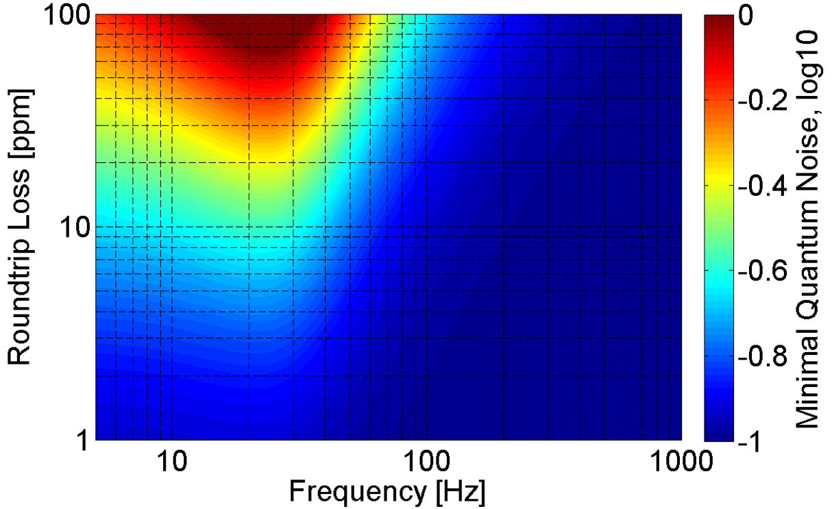
Figure 13: Degradation of 10 dB external squeezing reflected from a 300 m filter cavity as function of round-trip loss (in addition to input transmission) and frequency.
