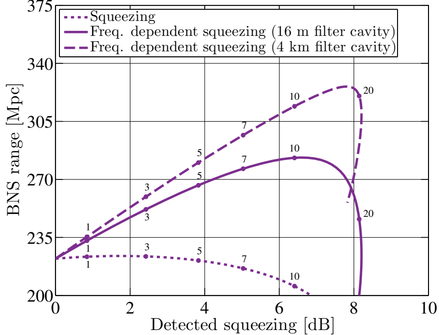
Figure 7: Impact of squeezing in Advanced LIGO on BNS range as a function of measured high-frequency quantum noise reduction. Numerical labels indicate the level of injected squeezing in dB (the best experimentally measured value currently stands at approximately 12 dB [7]). A number of loss mechanisms couple anti-squeezing into the measurement quadrature [8]. These effects are most noticeable with high levels of injected squeezing and are responsible for the curious double-valued nature of the frequency dependent curves.
