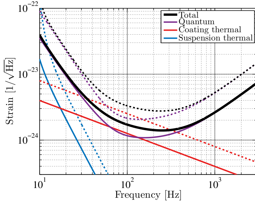
Figure 4: Strain sensitivity of A+. Improved thermal noise (factor of two), improved quantum noise (16 m filter cavity and 6 dB of measured squeezing at high frequency) and heavier test masses (also a factor of two) are shown. The equivalent Advanced LIGO curves are shown as dashed lines.
