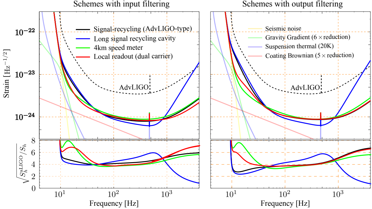
Figure 26: Optimization results for different schemes assuming more substantial thermal noise improvements, increasing the mirror mass from 40 to 150 kg, and increasing the arm cavity power from 800 to 3000 kW.
