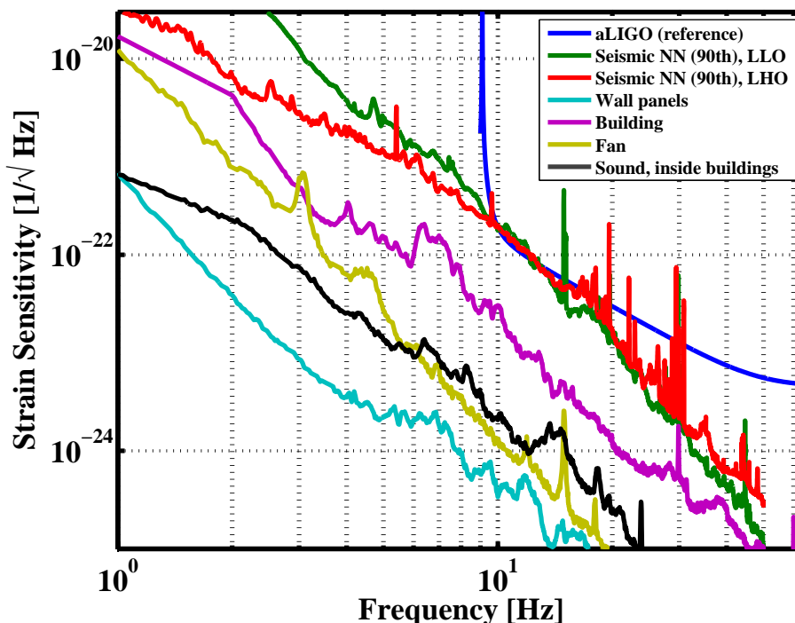
Figure 29: Newtonian noise estimates for the LIGO sites [142]
