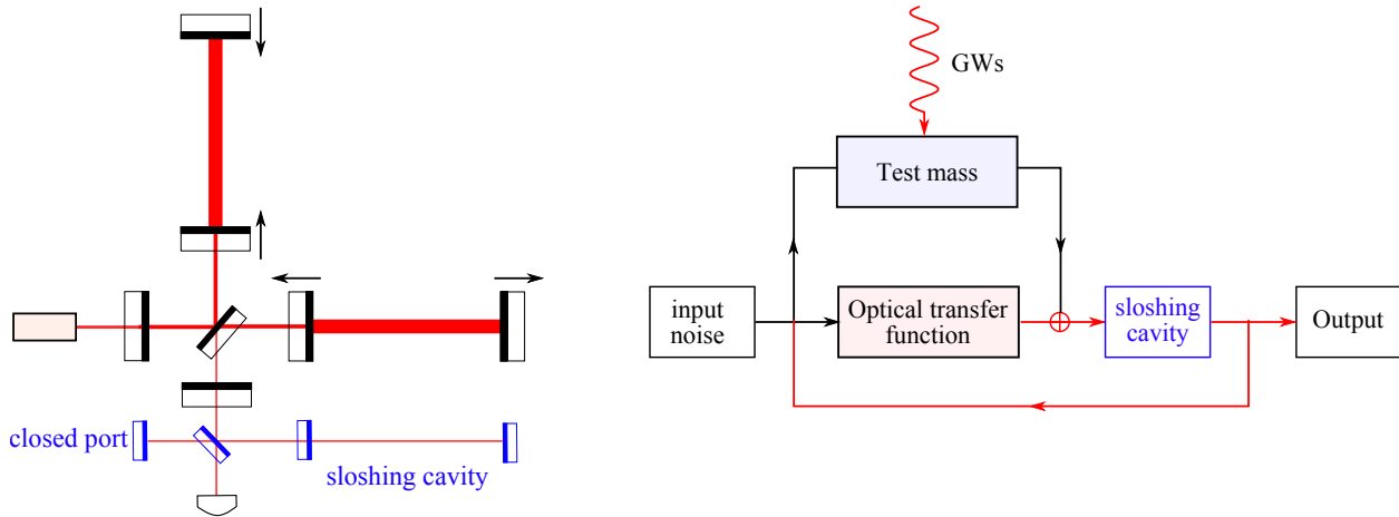
Figure 21: Schematics showing the speed-meter configuration (left) and its flow chart (right).
