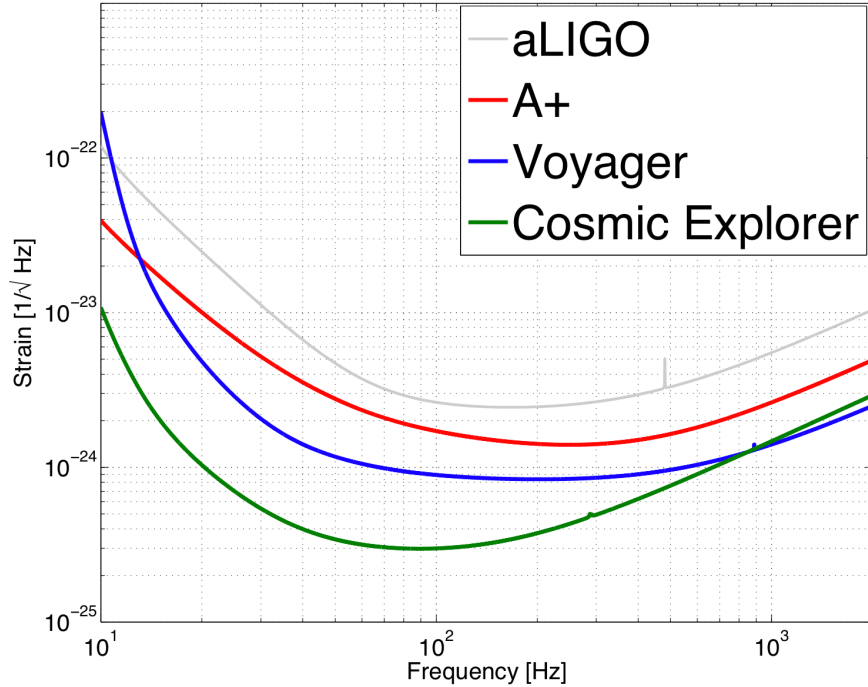
Figure 3: Strawman sensitivity curves for A+, LIGO Voyager and LIGO Cosmic Explorer gravitational wave detectors.
