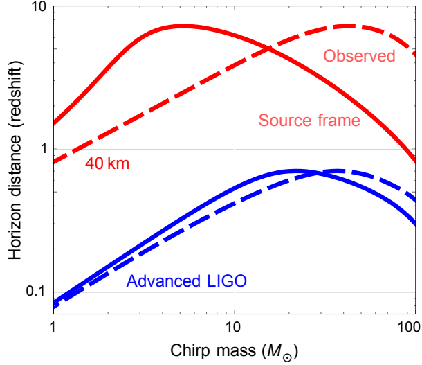
Figure 10: Astrophysical reach for compact binary inspiral systems. The maximum observable distance is shown as a function of the chirp mass in the source frame (solid lines) and as a function of the observed chirp mass seen on Earth (dashed lines). Blue lines represent the reach of Advanced LIGO, whereas red lines represent the reach of Advanced LIGO with extended arms, based on the sensitivity shown in figure 6. A Hubble constant of 67.9 km/s/Mpc was assumed.
