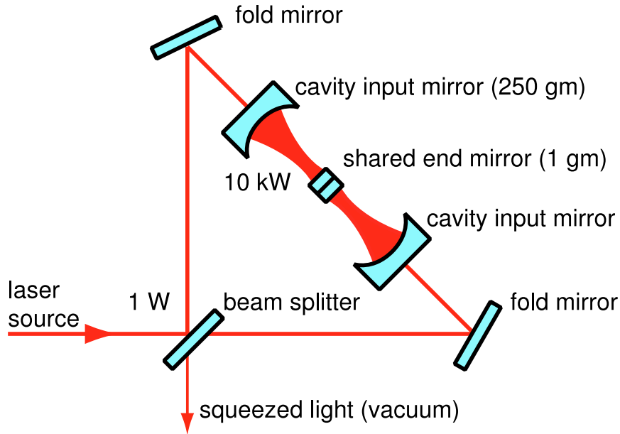
Figure 27: Ponderomotive Squeezer, taken from Corbitt et al. [74]
