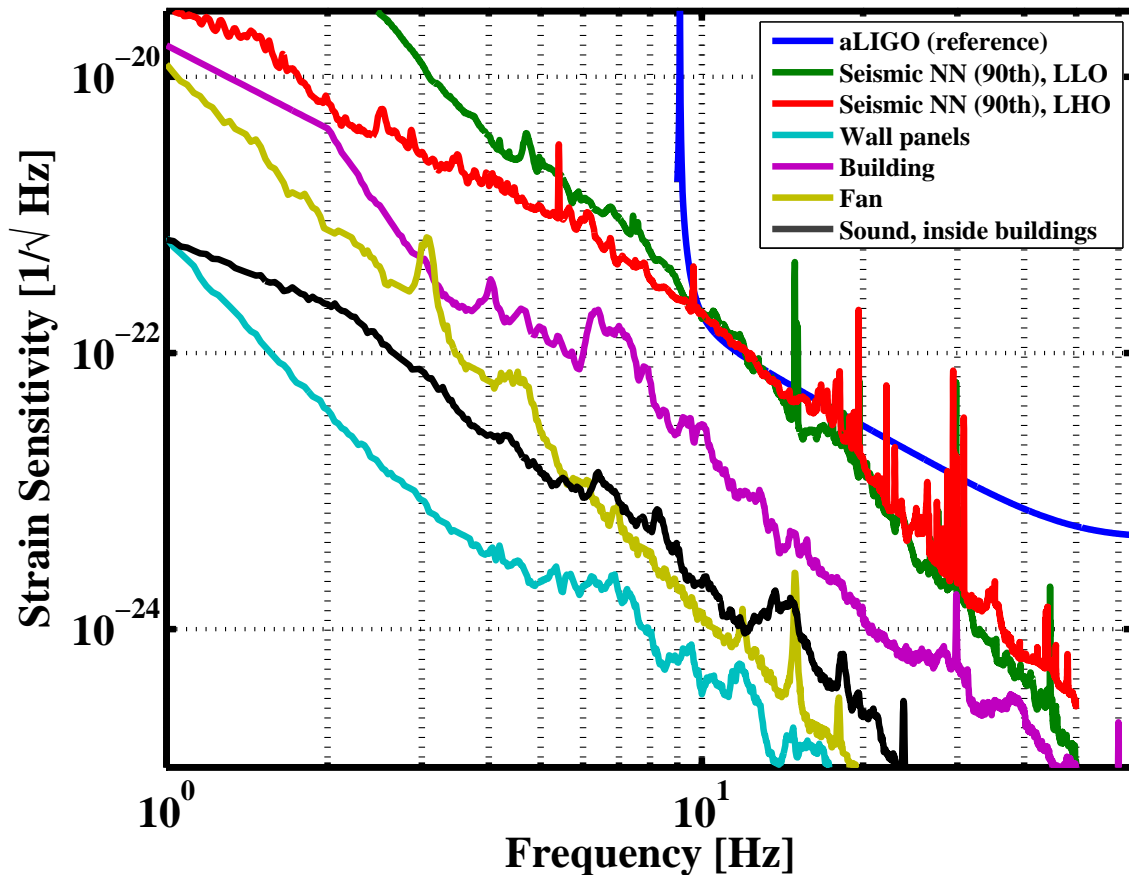
Figure 29: Newtonian noise estimates for the LIGO sites [143]
