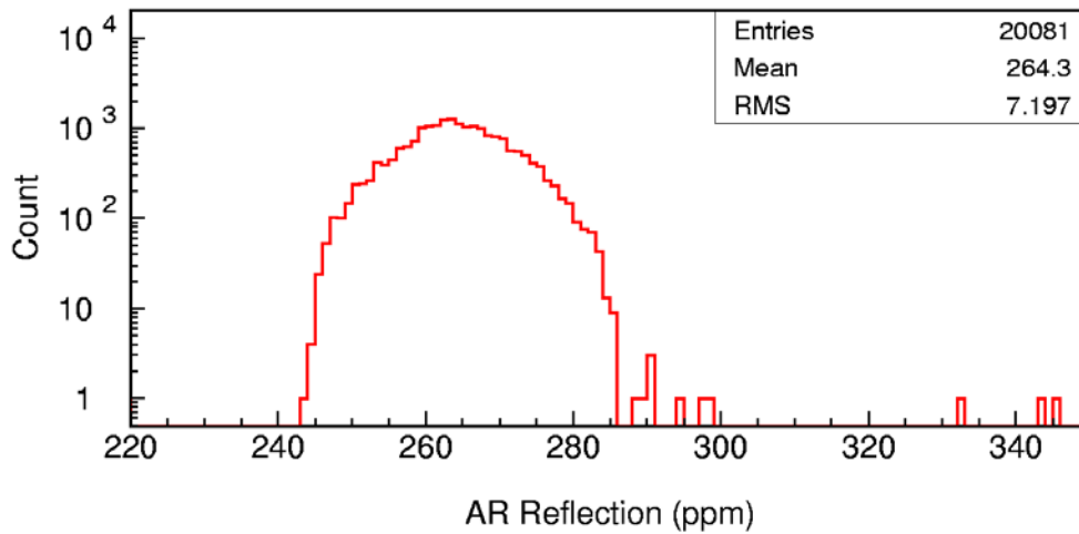
Fig. 1 ITM03 S2 AR reflection over a 160 mm diameter aperture.
