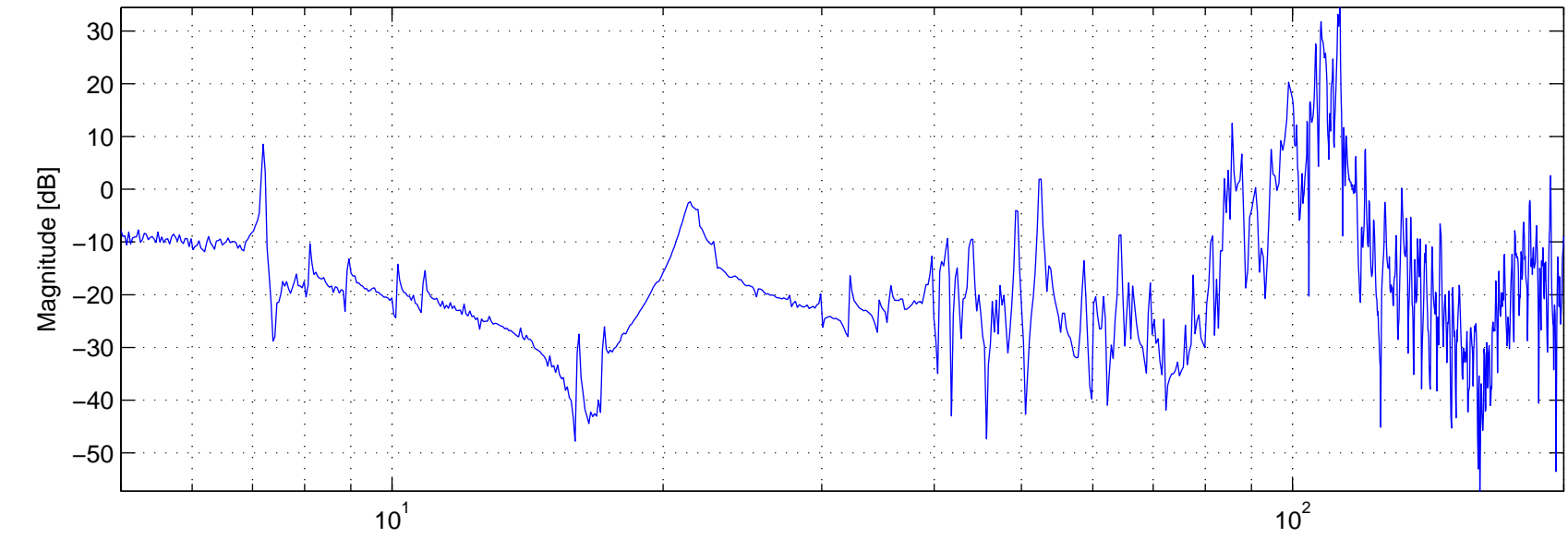
CPBS, Prototype Transmissibility Z Direction (Vertica Axis)
