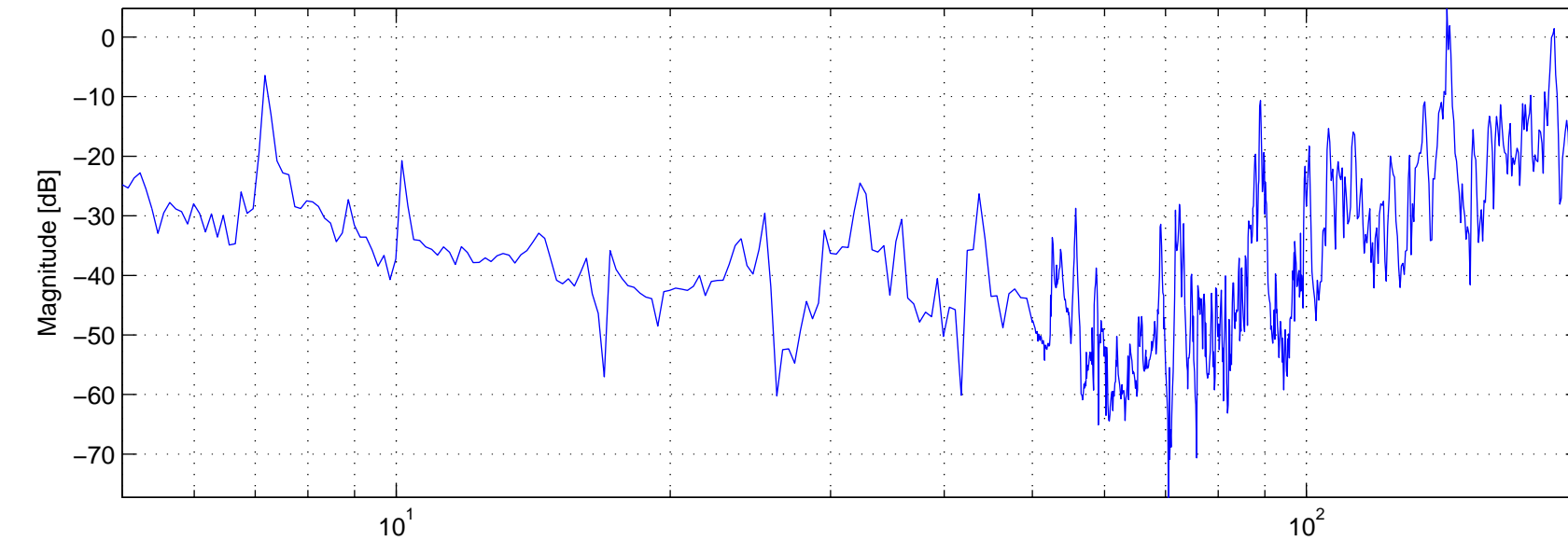
CPBS, Prototype Transmissibility Y Direction (along the beam)
