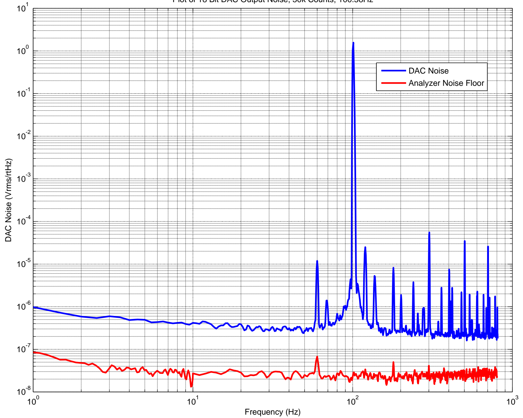
Plot of 18 Bit DAC Output Noise, 50k Counts, 100.58Hz
