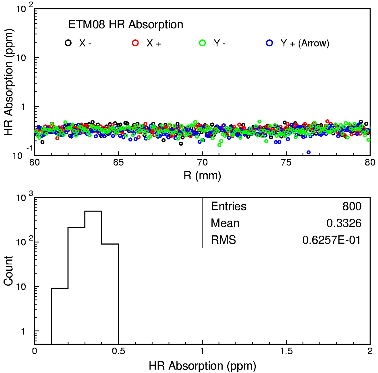
Fig.1 ETM08 HR absorption radial scans along 4 directions outside 120 mm aperture.
