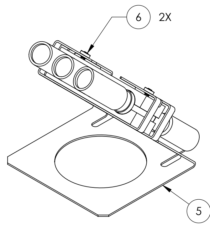
ISO VIEW (SHOWN WITH OPTIONAL 45 DEGREE MT.)
